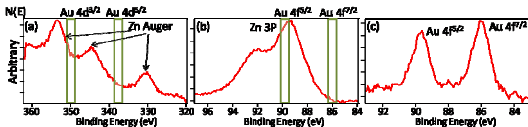
Fig.10 XPS spectra. (a) and (b) are the spectra of ZnO nanorods grown on Si substrate with gold NPs by solid source CVD method (substrate temperature was 450°C). (c) is the spectrum of Si substrate with gold NPs annealed at 450°C for 30min. There were no gold peaks in (a) and (b).
