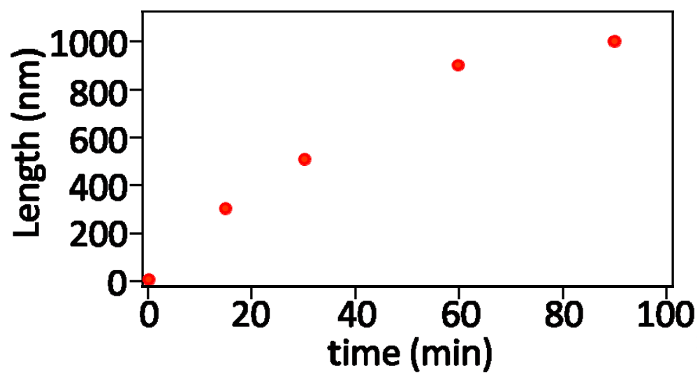
Fig.11 Relationship between reaction time and length of ZnO nanorods.
