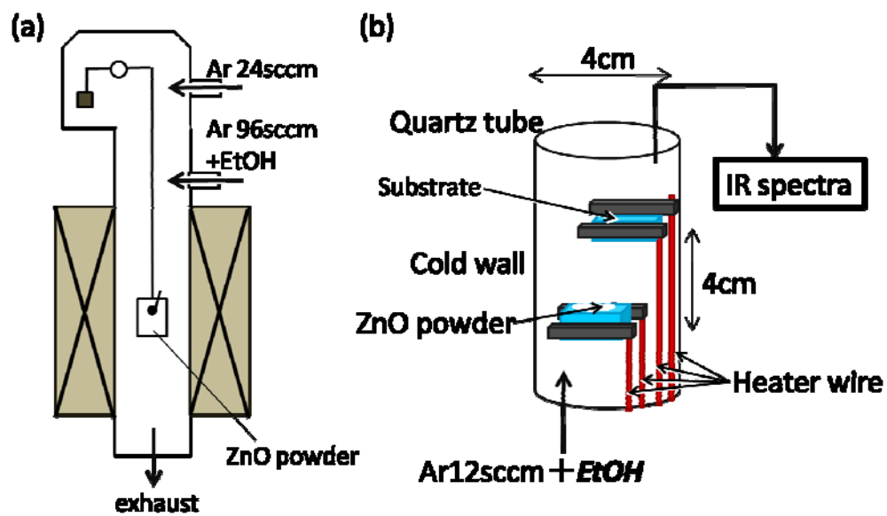
Fig.1 Schematic diagrams of equipment used in this research. (a) is that of TG, and (b) is that of atmospheric pressure solid source CVD.
