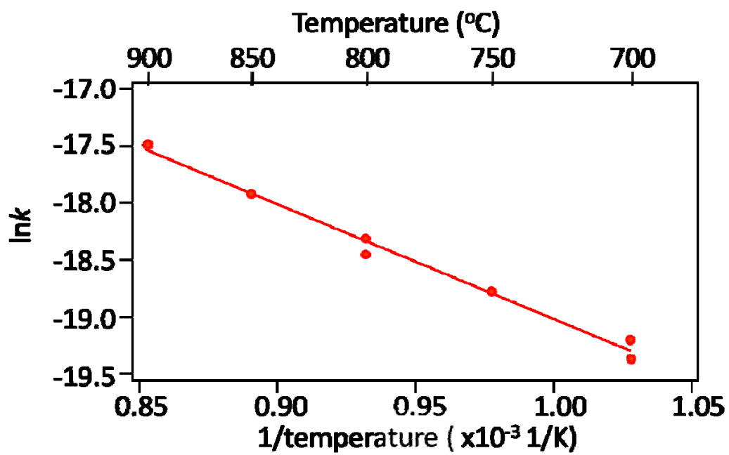
Fig.3 Arrhenius plot calculated by TG results.
