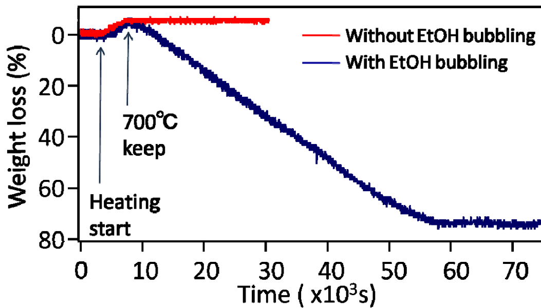
Fig.2 TG results : time versus weight loss of ZnO. Red line is the result in condition without ethanol bubbling, and blue one is the result in condition with ethanol bubbling.
