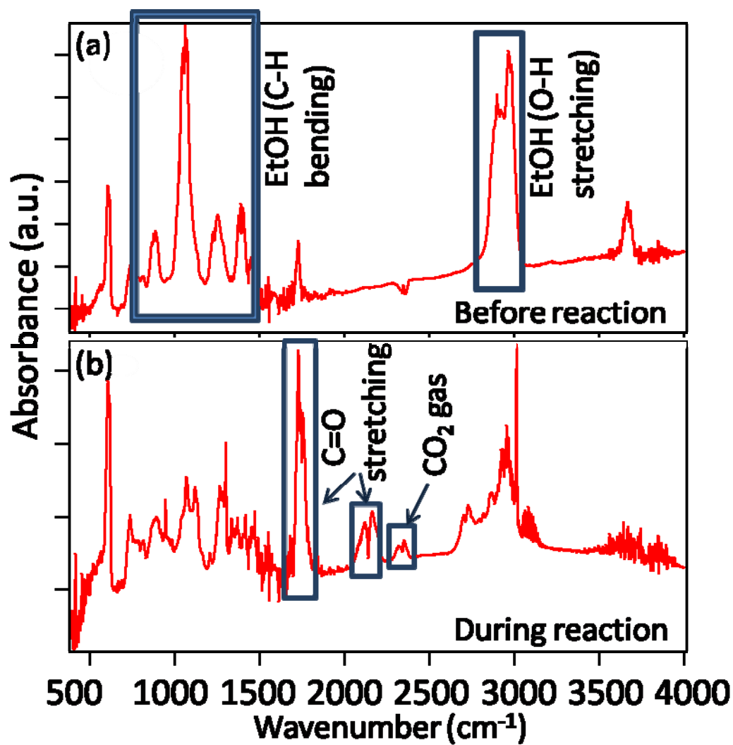
Fig.4 IR absorption spectra of exhaust gas of solid source CVD method. Upper graph (a) is measured before heating source, and lower one (b) is measured during reaction.
