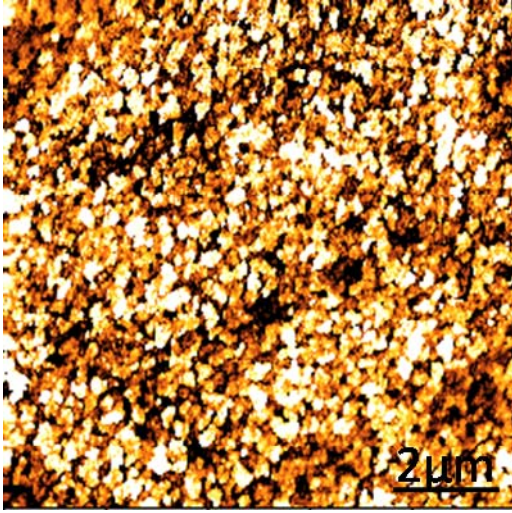
Fig.6 AFM image of the surface of an ITO substrate used in this experiment. The substrate temperature was 550°C. RMS roughness of the surface was approximately 2.7nm and many nanoscale particles were observed.
