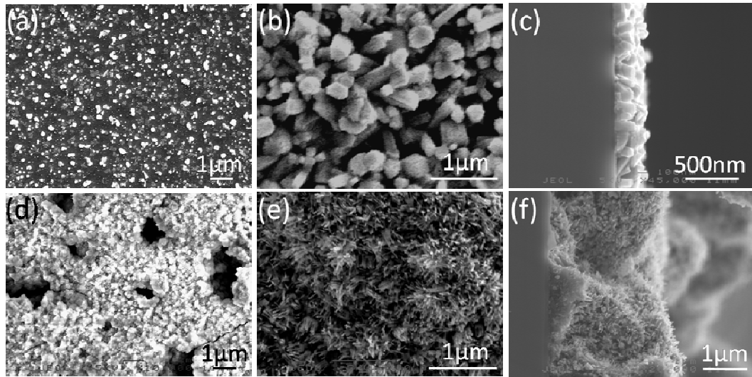
Fig.9 SEM images. (a) is gold NPs with low density on Si substrate, (b) is top view of ZnO nanorods grown in the area of gold NPs with low density, and (c) is cross-section. (d) is gold NPs with high density on Si substrate, (e) is top view of ZnO nanorods grown in the area of gold NPs with high density, and (f) is cross-section. The substrate temperature of (b),(c),(e),and (f) is 450°C.
