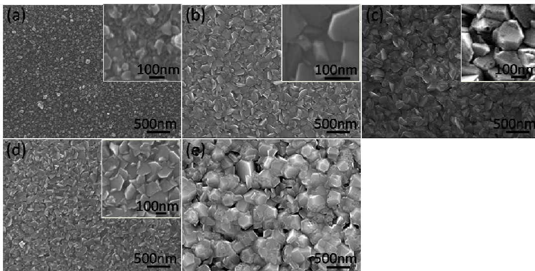
Fig.7 SEM images of ZnO on Si substrates. (a) is that substrate temperature is 300°C, (b) is 350°C, (c) is 400°C, (d) is 450°C, and (e) is 500°C. (b), (d) are rather thin film like. In narrow scale, (a),(c), and (e) has skeleton crystals but (b), (d) does not have.
