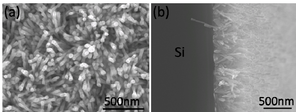
Fig.8 SEM images of ZnO on Si substrate with gold NPs. (a) is top view and (b) is cross-section. The substrate temperature was 450°C.
