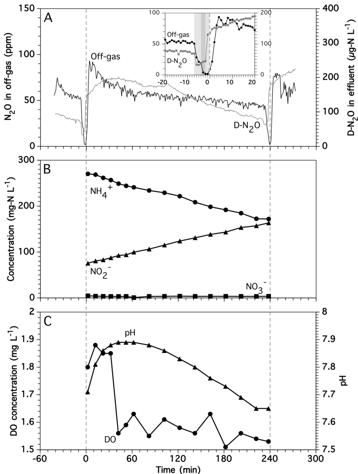
Figure 3. The concentration profiles of (A) \text{N}_2\text{O} in the off-gas and \text{D-N}_2\text{O} , (B) \text{NH}_4^+ , \text{NO}_2^- and \text{NO}_3^- , and (C) DO and pH during one typical cycle of the sequencing batch reactor operation. Inset of panel A shows the concentration profiles of \text{N}_2\text{O} in the off-gas
