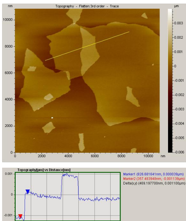
Figure 2. - A typical AFM image of the graphite oxide on a mica substrate. The thickness of the graphene oxide was estimated to be 1.1 nm.
