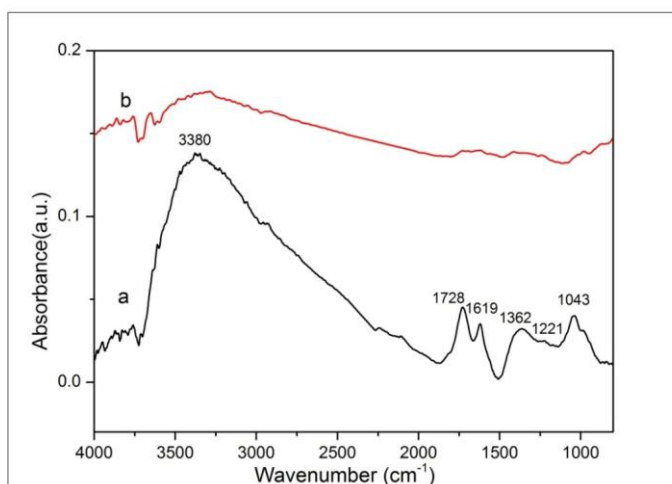
Figure 5. Typical FT-IR spectra of graphene oxide (a) and of the TDO-reduced graphene (b).
