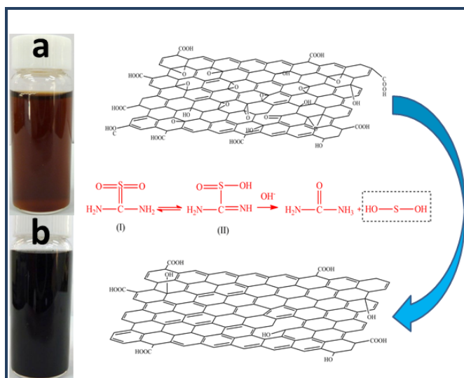
Figure 8. Schematic illustration of the reduction, including photographs of (a) the graphene oxide aqueous solution and (b) the reduced graphene sheets in aqueous solution.
