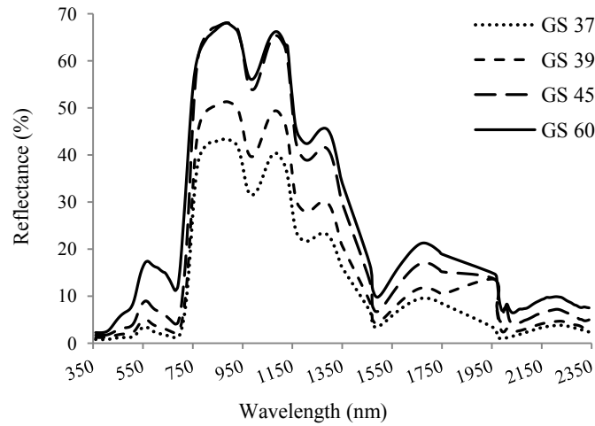
Fig. 4.2 Reflectance measurements in four different growth stages using a spectroradiometer (FS3).
