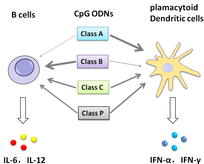
Figure 1.5 Distinct classes of CpG ODNs. Four classes of such chemically modified synthetic CpG ODNs have been defined based on their different ability to stimulate cells that express TLR 9 as well as their structures.
