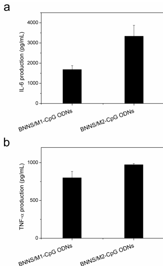
Figure 2.20 Cytokine induction from PBMCs stimulated by BP7 mutants–CpG ODNs conjugate-loaded BNNS. (a) IL-6 production. (b) TNF- \alpha production. Loaded BNNS (87 \mu g/mL) was incubated with PBMCs for 8 h (TNF- \alpha ) and 24 h (IL-6) respectively, M1 (BP7-Y8A) and M2 (BP7-L10A) are mutants of BP7 whose tyrosine (Y8) and leucine (L10) at eighth and tenth positions from N-terminal were replaced by alanine (A), respectively. Data are presented as mean \pm SD (n = 3).
