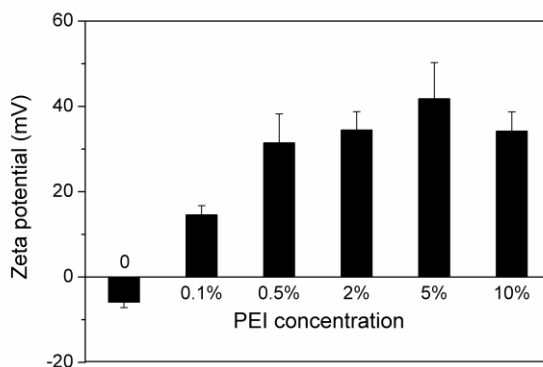
Figure 3.2 Zeta potentials of BNNS and series BNNS-PEI complexes at different starting concentration of PEI.
