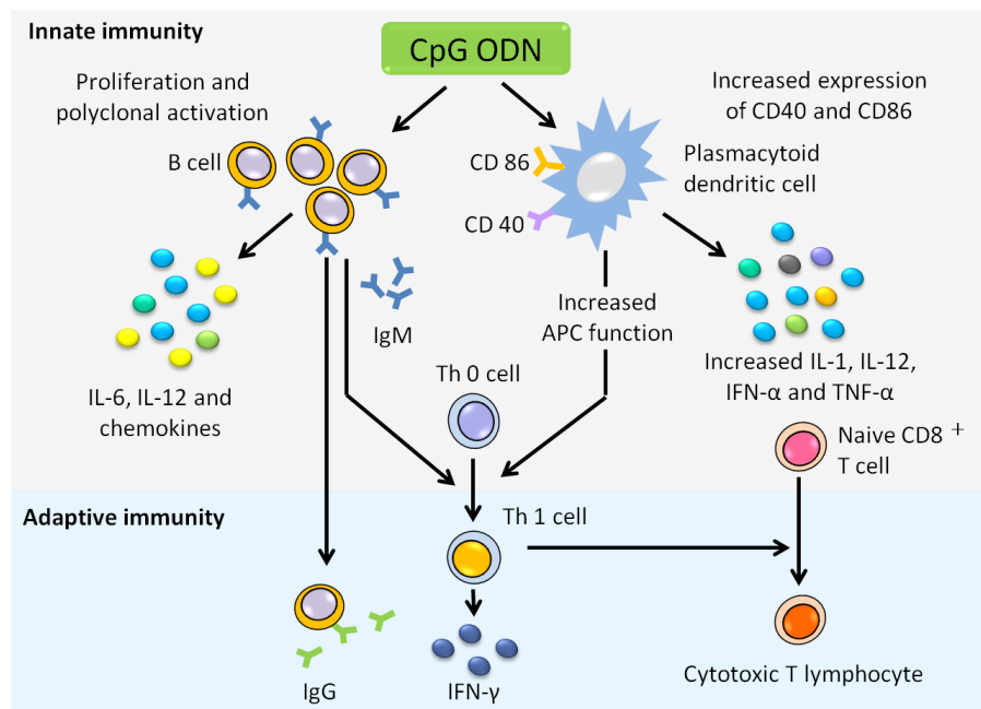
Figure 1.3 Immunostimulatory effect of CpG ODNs. CpG ODNs directly activate human B cells and pDCs, creating an immune milieu that is rich in pro-inflammatory and T helper 1 (Th1)-type cytokines. This innate immune response forms a foundation on which antigen-specific adaptive immunity is based. In particular, by improving the function of professional antigen-presenting cells (APCs), CpG ODNs facilitate the generation of humoral and cellular vaccine-specific immunity. IFN, interferon; IL, interleukin; TNF, tumor-necrosis factor. 14
