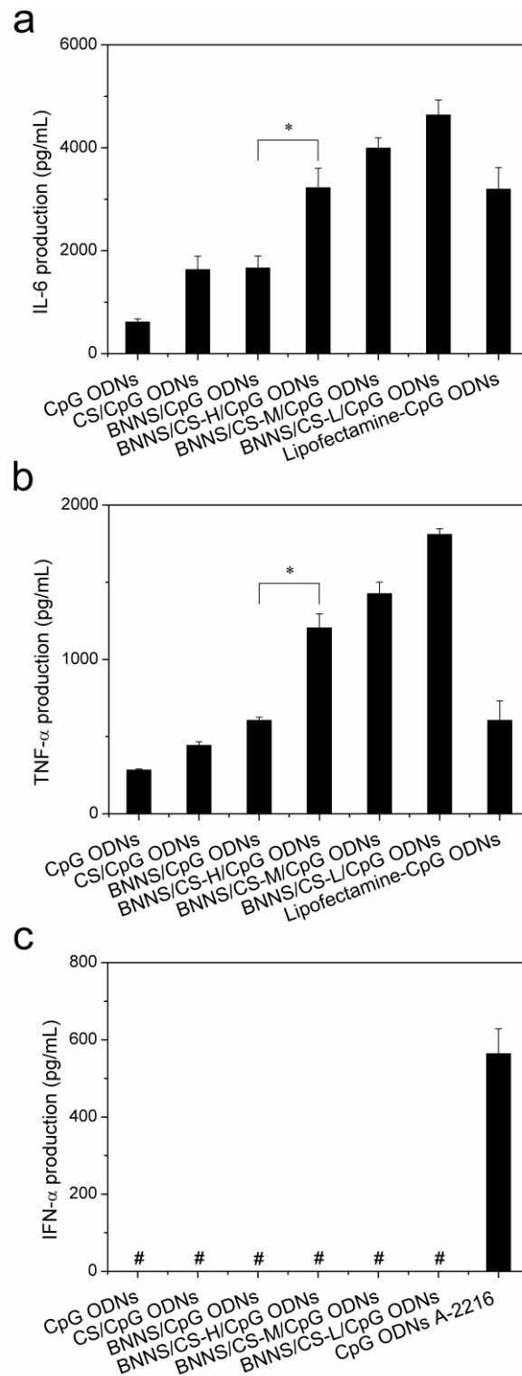
Figure 4.8 Cytokine induction in PBMCs stimulated by CpG ODNs loaded on BNNS and BNNS/CS complexes. Loaded BNNS or BNNS/CS complexes (50 \mu g/mL). (a) IL-6 production. (b) TNF- \alpha production. (c) IFN- \alpha production. Lipofectamine TM 2000 was used for comparison. Data are presented as mean \pm SD (n = 3). The symbol # means not detectable (below detection limit). * p < 0.05.
