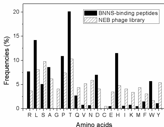
Figure 2.4 Amino acid frequencies in the BNNS-binding peptide sequence.
