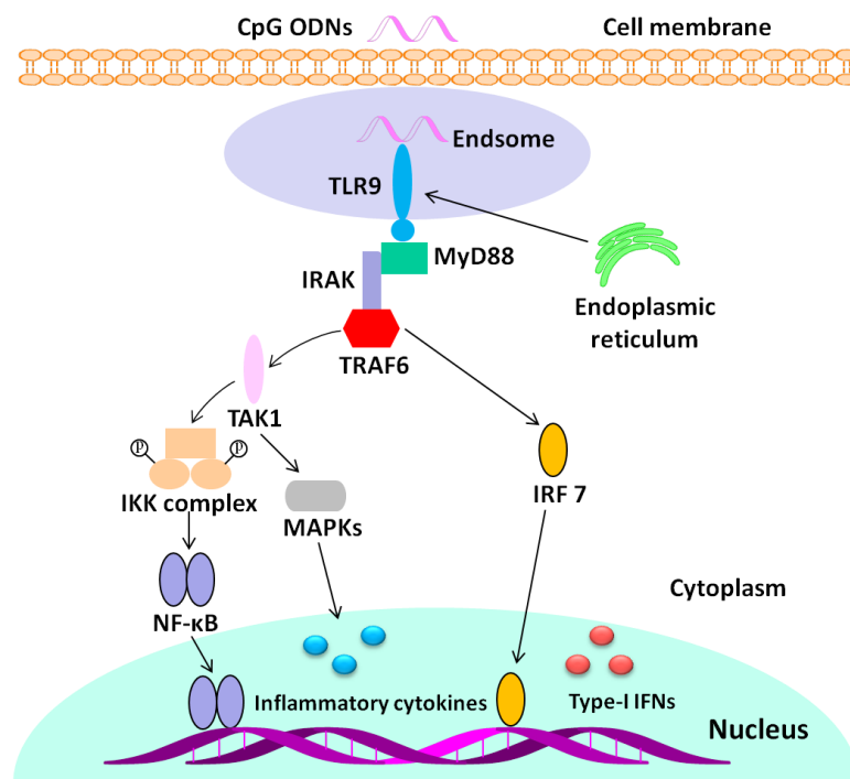
Figure 1.2 CpG ODNs-TLR 9 interaction and cell signaling. CpG ODNs are internalized into endosome and interact with TLR 9. This interaction triggers a MyD88-dependent pathway, leading to the upregulation of NF-κB and IRF-7, which respectively activates production of pro-inflammatory cytokine genes and type I IFN gene.
