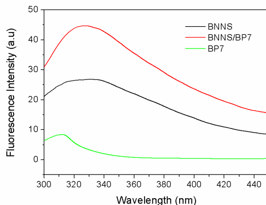
Figure 2.10 Fluorescence emission spectra of BNNS, BP7 and BNNS/BP7 complex in TBS buffer.
