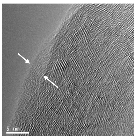
Figure 2.15 TEM image of BP7–CpG ODNs conjugate-loaded BNNS. The white arrows indicate the bound layer of BP7–CpG ODNs conjugate.
