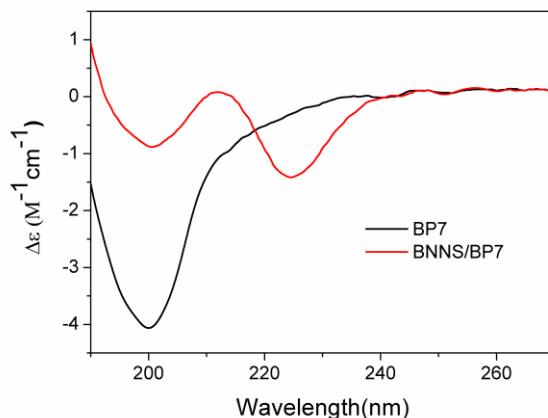
Figure 2.9 CD spectra of BP7 and the BNNS/BP7 complex measured between 190 nm and 270 nm with a scanning speed of 20 nm/min and a bandwidth of 0.5 nm.
