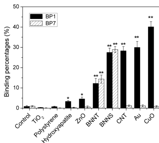
Figure 2.7 Binding specificities of the peptides for BNNS. FITC-labeled BP1 and BP7 were incubated with BNNS or other nanomaterials for 1 h. Solutions were centrifuged and unbound peptide was determined by the fluorescence intensity of supernatant. Binding specificities were calculated as the percentage of peptide that bound to each nanomaterial. Data are presented as mean \pm SD ( n = 3 ); * p < 0.05 , ** p < 0.01 .
