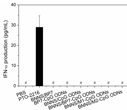
Figure 2.19 IFN- \alpha induction from PBMCs stimulated by CpG ODNs. M1 (BP7-Y8A) and M2 (BP7-L10A) are mutants of BP7 whose tyrosine (Y8) and leucine (L10) at eighth and tenth positions from N-terminal were replaced by alanine (A), respectively. The concentration of the BNNS was about 87 \mu g/mL. PTO-2216 CpG ODNs are positive control. Data presented as mean \pm SD (n =3). The symbol # means not detectable (below detection limit).
