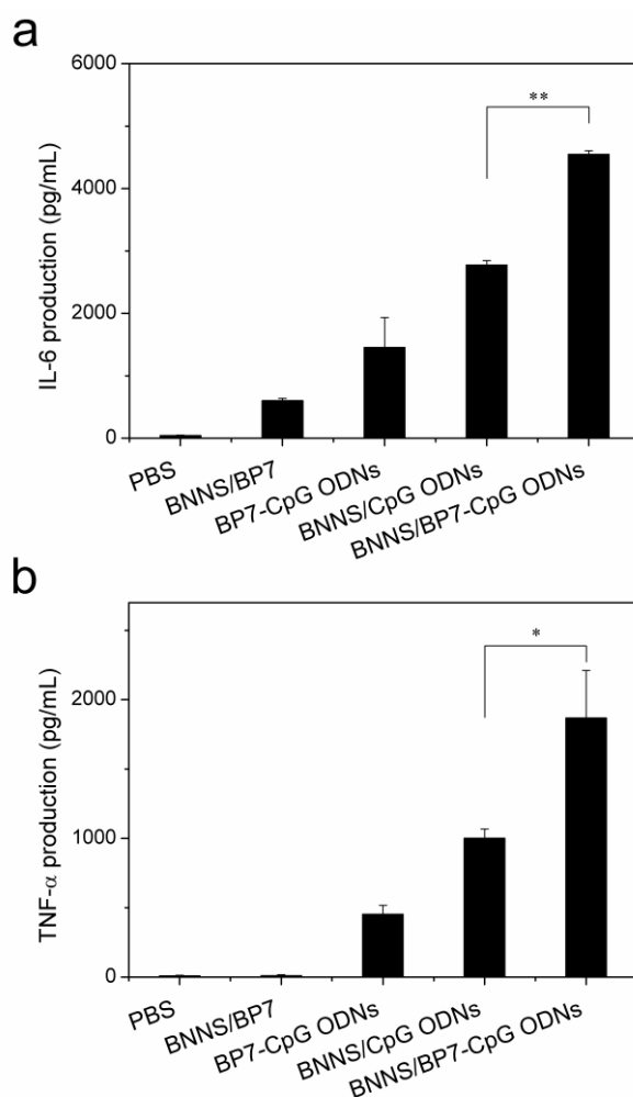
Figure 2.18 Cytokine induction in PBMCs stimulated by BP7-CpG ODNs conjugate-loaded BNNS. Loaded BNNS (87 \mu g/mL) or a corresponding concentration of free BP7-CpG ODNs conjugate (1 \mu g/mL) was incubated with PBMCs for 8h (TNF- \alpha ) and 24h (IL-6) respectively. (a) IL-6 production. (b) TNF- \alpha production. Data are presented as mean \pm SD (n = 3); *p < 0.05, **p < 0.01.
