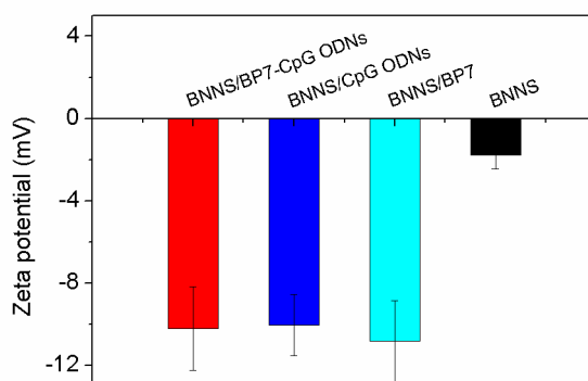
Figure 2.17 Zeta potentials of BNNS, BNNS/BP7, BNNS/CpG ODNs, BNNS/BP7–CpG ODNs complexes in TBS buffer (pH 7.4). Data presented as mean \pm SD (n =6).
