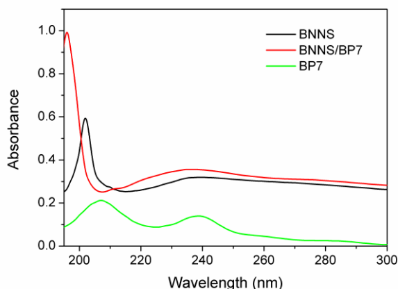
Figure 2.11 UV/vis absorption spectra of BNNS, BP7, and the BNNS/BP7 complex.
