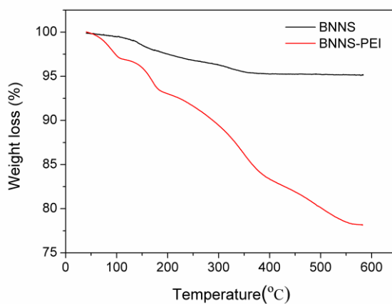
Figure 3. 3. Thermal gravimetric analysis of the BNNS and BNNS-PEI complexes.
