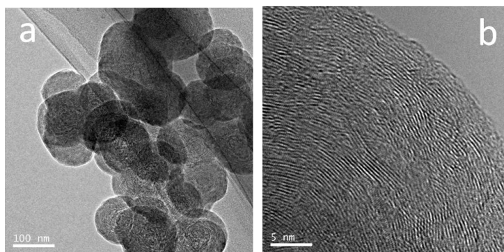
Figure 1.7 Typical transmission electron microscopy image of the BNNS. (a) Low-resolution image. (b) High-resolution image.
