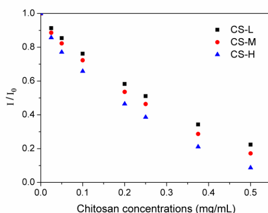
Figure 4.9 The plot of I/I_0 vs. [CS] for fluorescence quenching curves of CpG ODNs-EB by the CS of different MW. [CS], the concentrations of the chitosan. I_0 , fluorescence intensity in the absence of CS, I , fluorescence intensity in the presence of CS.
