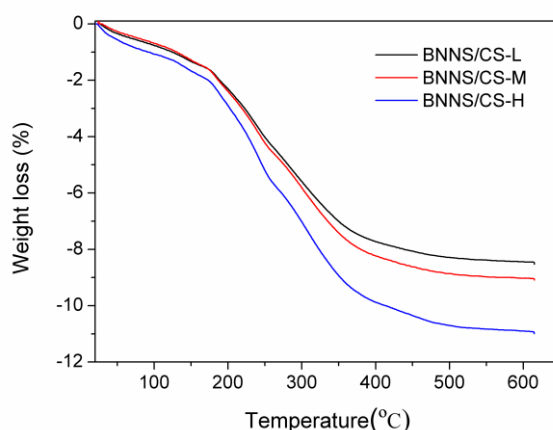
Figure 4.6 Thermogravimetric analysis curves of BNNS coated with CS.
