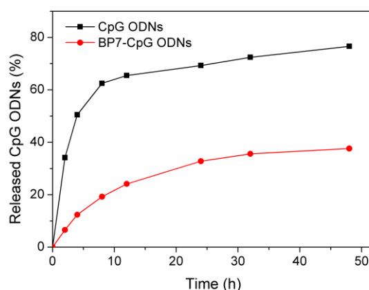
Figure 2.16 Release profile of CpG ODNs and the BP7–CpG ODNs conjugate loaded on BNNS at pH 5.
