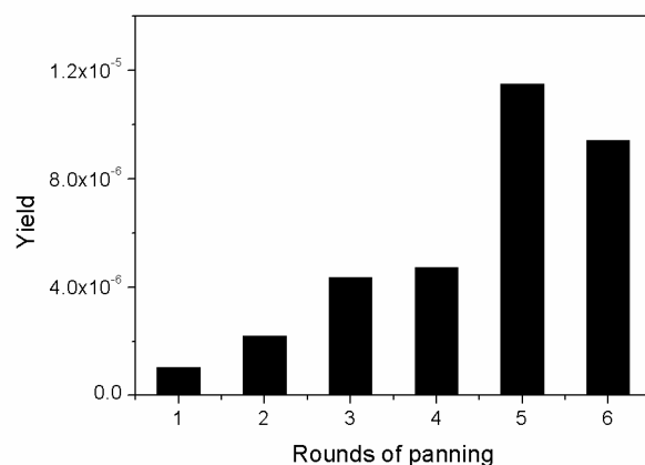
Figure 2.3 Yield (output phages /input phages) against the rounds of panning.
