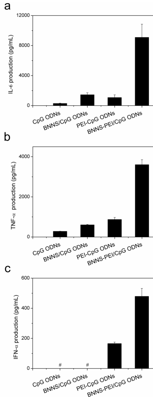
Figure 3.8 Cytokine induction from PBMCs stimulated by CpG ODNs loaded on BNNS and BNNS-PEI complexes. Loaded BNNS or BNNS/PEI complexes (50 \mu g/mL). (a) IL-6 production. (b) TNF- \alpha production. (c) IFN- \alpha production. Data are presented as mean \pm SD (n = 3). The symbol # means not detectable (below detection limit).
