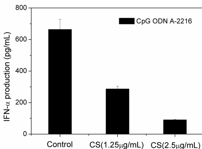
Figure 4.10 Suppressive effect of CS on IFN- \alpha induction from PBMCs by class A CpG ODNs 2216. PBMCs were treated with CS for 4 h first, and then stimulated with class A CpG ODNs 2216. After 24 h, supernatants were collected and tested for IFN- \alpha secretion by ELISA. Data are presented as mean \pm SD (n = 3).
