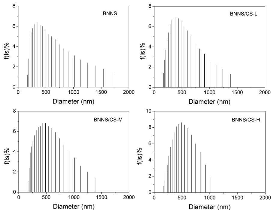
Figure 4.3 Size distributions of BNNS coated with CS of different molecular weights measured by DLS.
