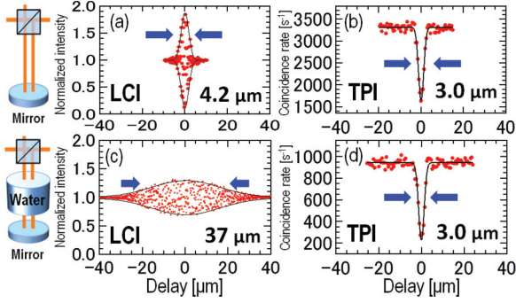
FIG. 4. (Color online) Experimental LCI and TPI interferograms for the Gaussian shaped spectrum: The 4.2- \mu\text{m} LCI (a) and 3.0- \mu\text{m} TPI (b) widths without any media and the broadened 37- \mu\text{m} LCI (c) and unchanged 3.0- \mu\text{m} TPI (d) widths using 25 mm of water as a dispersive media. The integration time is 1 s per point in panels (a)–(d).
