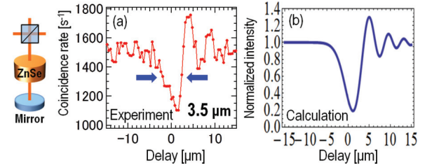
FIG. 6. (Color online) The experimental TPI interferogram with a 5-mm-thick ZnSe plate as a highly dispersive media (a) and a theoretical plot considering the third-order dispersion (b). The integration time is 1 s per point in panel (a).
