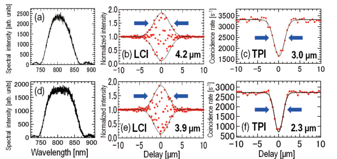
FIG. 3. (Color online) Experimental LCI and TPI interferograms for two spectral shapes: For the Gaussian shaped spectrum (a), the 4.2- \mu\text{m} LCI (b) and the 3.0- \mu\text{m} TPI (c) widths show a resolution enhancement factor R_e of 1.4; for the trapezoidal shaped spectrum (d), the 3.9- \mu\text{m} LCI (e) and the 2.3- \mu\text{m} TPI (f) widths show a value of 1.7 for R_e . The experimental data (red dots) and Gaussian fit curves (black solid line) are plotted. The integration time is 1 s per point in panels (b), (c), (e), and (f).
