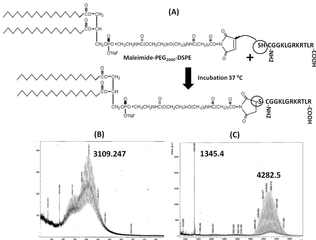
Figure 3.1: Conjugation of KLGR peptide with Maleimide-PEG 2000 -DSPE. (A) Synthesis of KLGR-PEG 2000 -DSPE by coupling of thiol group of the cysteine residue of KLGR peptide (calculated MW: 1340) with Maleimide-PEG 2000 -DSPE (calculated MW: 2936). Maleimide-PEG 2000 -DSPE and the KLGR peptide (molar ratio 1:1.2) were dissolved in water at 37 °C and allowed to react for 24 h. MALDI-TOF MS spectra of (B) Maleimide-PEG 2000 -DSPE and (C) KLGR-PEG 2000 -DSPE, which confirmed that the conjugation was successful, as evidenced by the molecular shifts of free KLGR peptide from 1345.4 (observed MW) to 4282.5 (observed MW) which is the sum of the individually calculated MW of KLGR peptide and Maleimide-PEG 2000 -DSPE.
