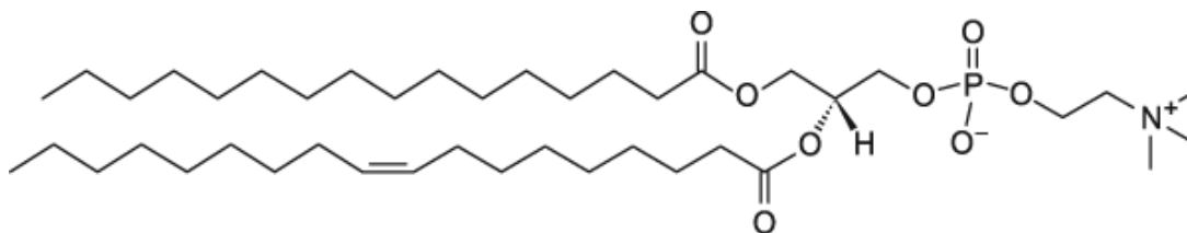
Egg phosphatidylcholine (EPC)
