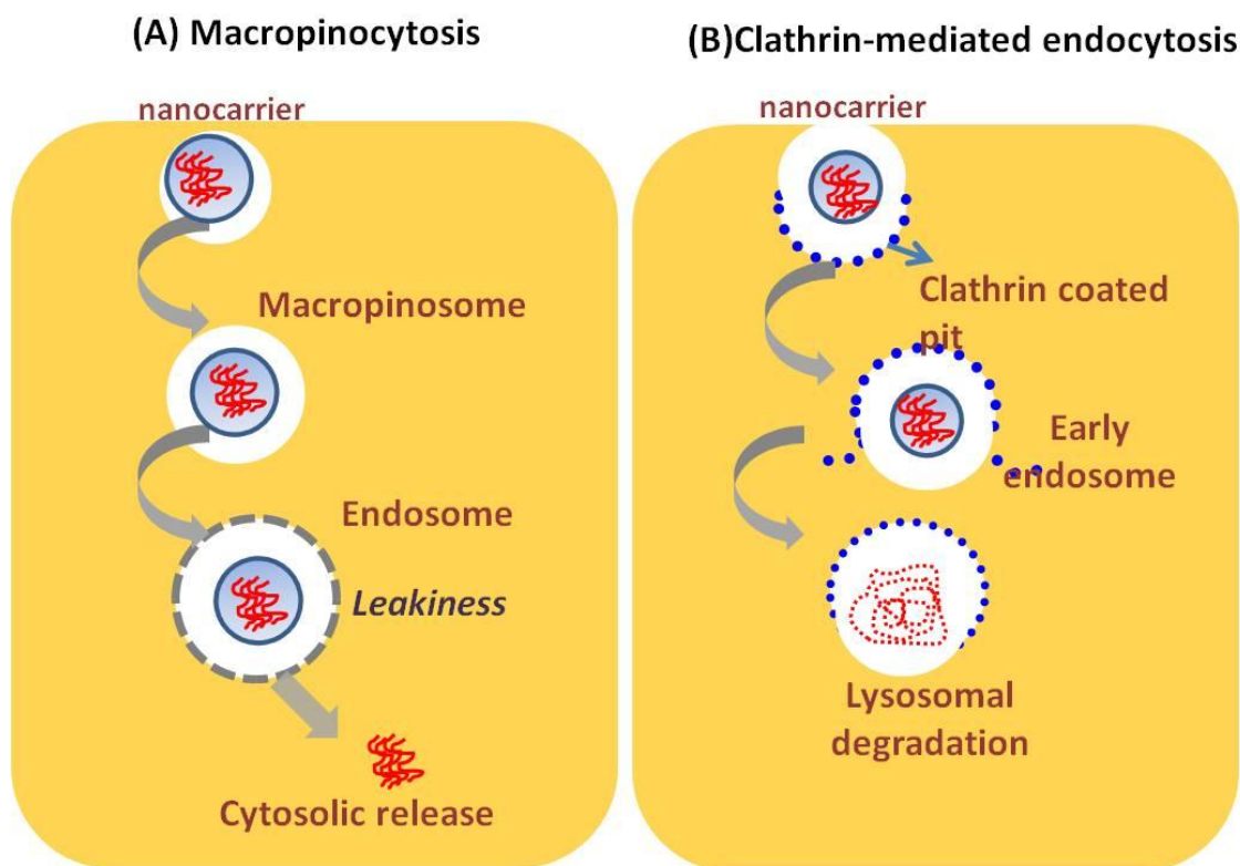
Figure 3.12: Graphical representation of (A) Macropinocytosis and (B) Clathrin-mediated endocytosis
