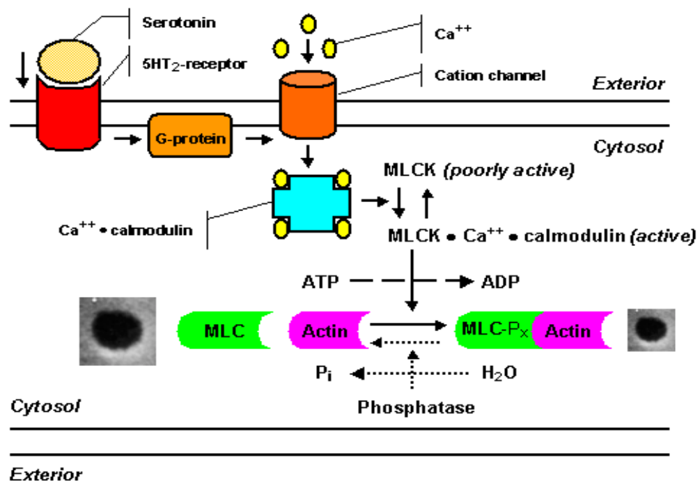
Figure 1.4: Scheme of the serotonin signal pathway showing the steps in fenestral contraction and relaxation [21].
