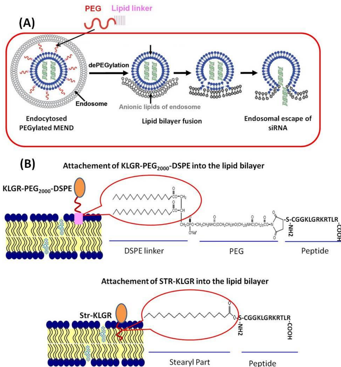
Figure 3.11: (A) Shematic representation of Endosomal escape. (B) Schematic representation of the attachment of KLGR-PEG and STR-KLGR at the surface of lipid bilayer of MEND
