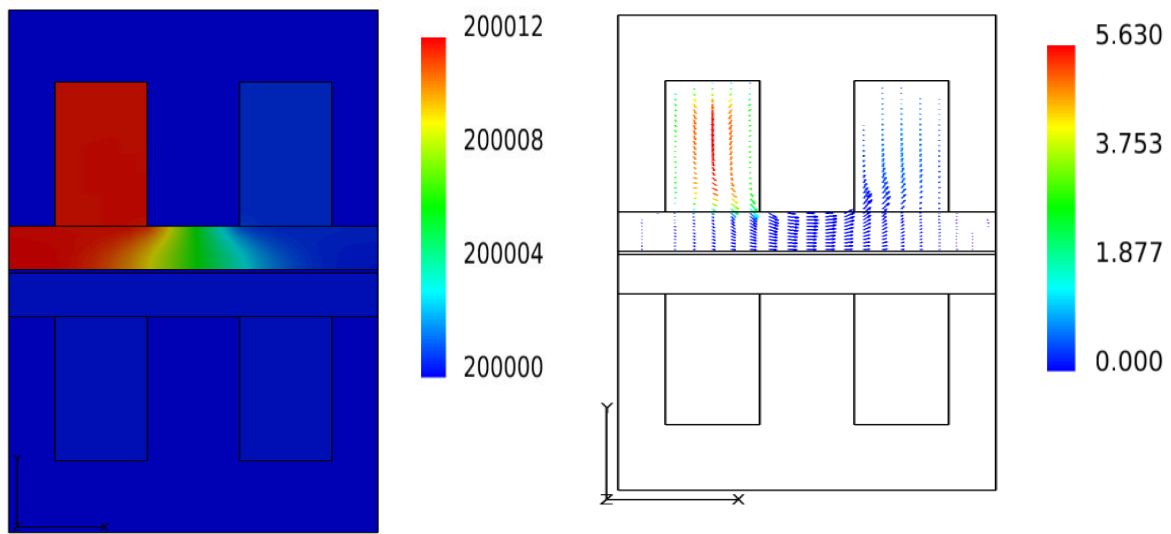
Fig. 4.7: Distribution of pressure (Pa) and velocity ( \text{m s}^{-1} ) in the gas channel and the GDL on the x - y plane at the middle cross section of the cell (at z = 2 \text{ mm} ).
