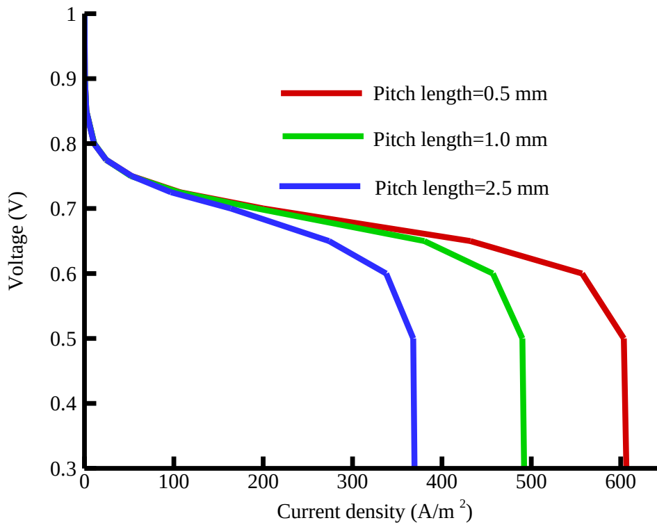
Fig. 4.5: Polarization curve for various gas channel pitch length with Case1
