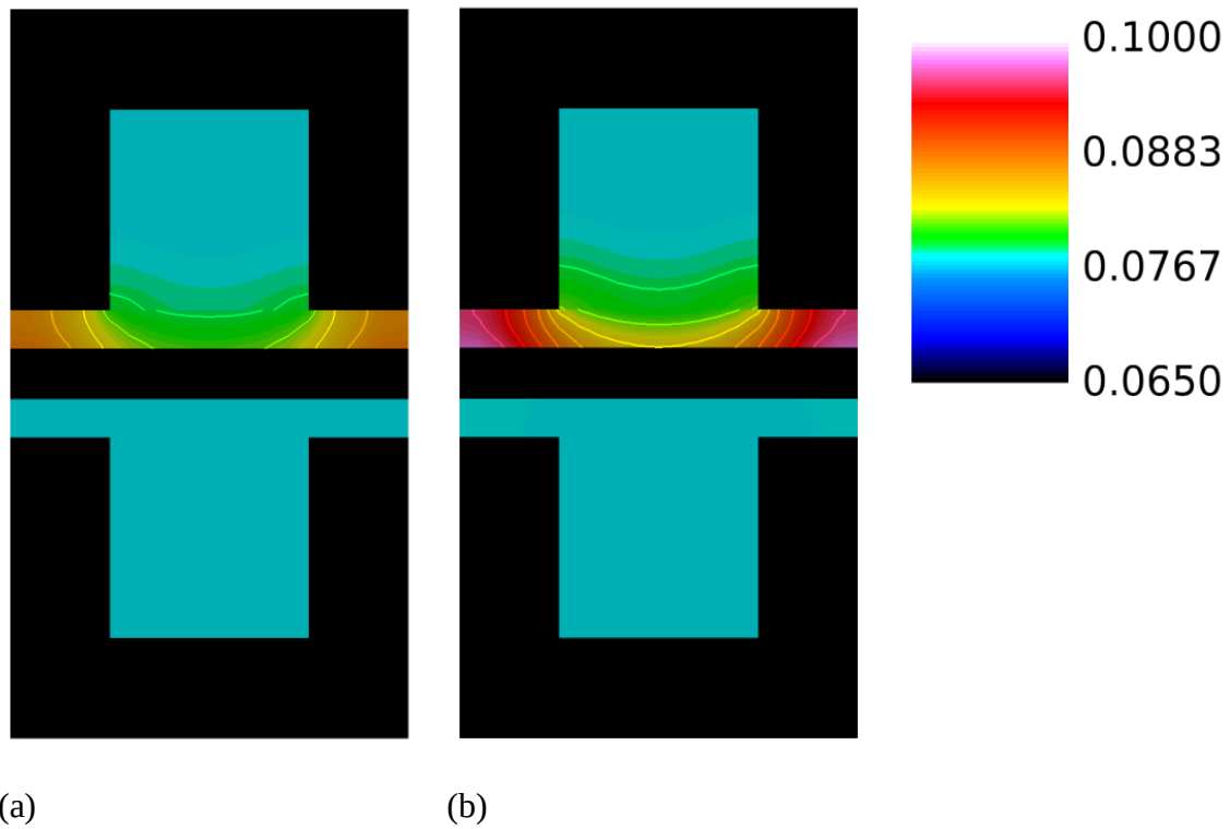
Fig. 5.7. Water concentration distribution in the gas channel and the gas diffusion layer (both anode and cathode sides) at a relative humidity of 40% and current densities of (a) 0.1 A/cm 2 and (b) 0.2 A/cm 2
