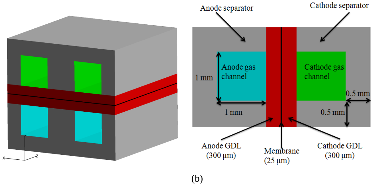
(a) Fig. 4.1: (a) Schematic view of a PEFC (b) Half Cross sectional view of a computational domain with a pitch length of 1 mm
