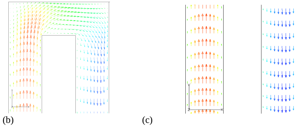
Fig. 3.3: (a) Velocity ( \text{m s}^{-1} ) distribution at the mid-plane of the gas channel (b) Velocity ( \text{m s}^{-1} ) at the corner of U-turn (c) at the middle of the channel
