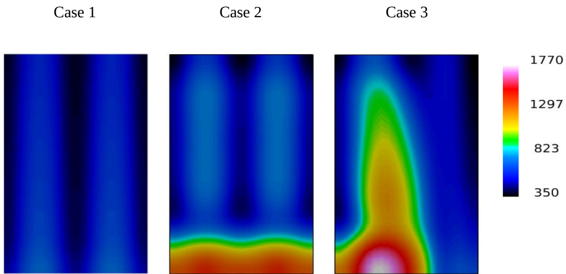
Fig. 4.10: The current density ( \text{A}/\text{m}^2 ) distribution on the middle cross-section in the membrane for Case 1, Case 2, and Case 3
