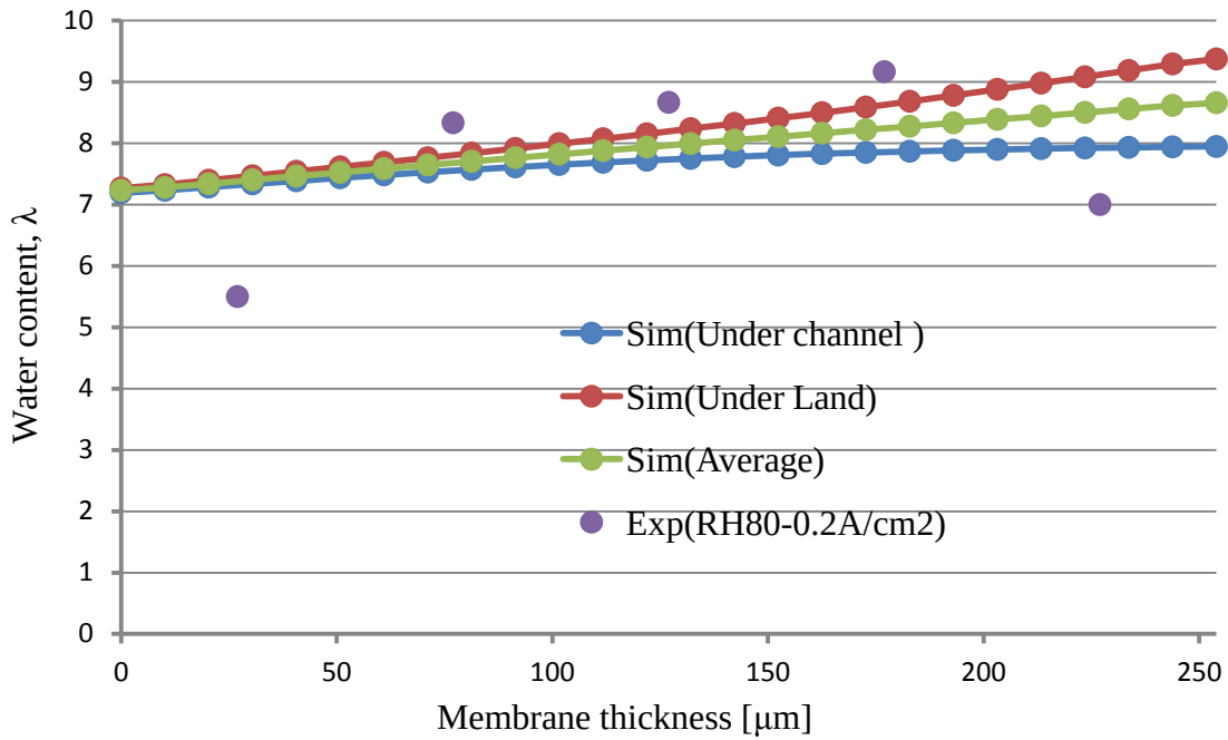
Fig. 5.15. Comparison of the experimental (Exp) and simulated (Sim) water content profiles in the membrane for a relative humidity of 80% and current densities of (a) 0.1 \text{ A/cm}^2 and (b) 0.2 \text{ A/cm}^2
