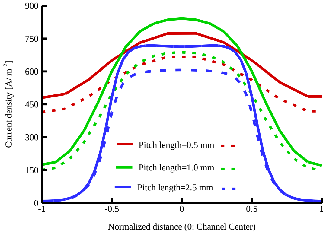
Fig. 4.4: The current density distribution along in-plane direction in the mid-length of the cell for various gas channel pitch lengths for Case 1 (dashed lines) and Case 2 (solid lines)
