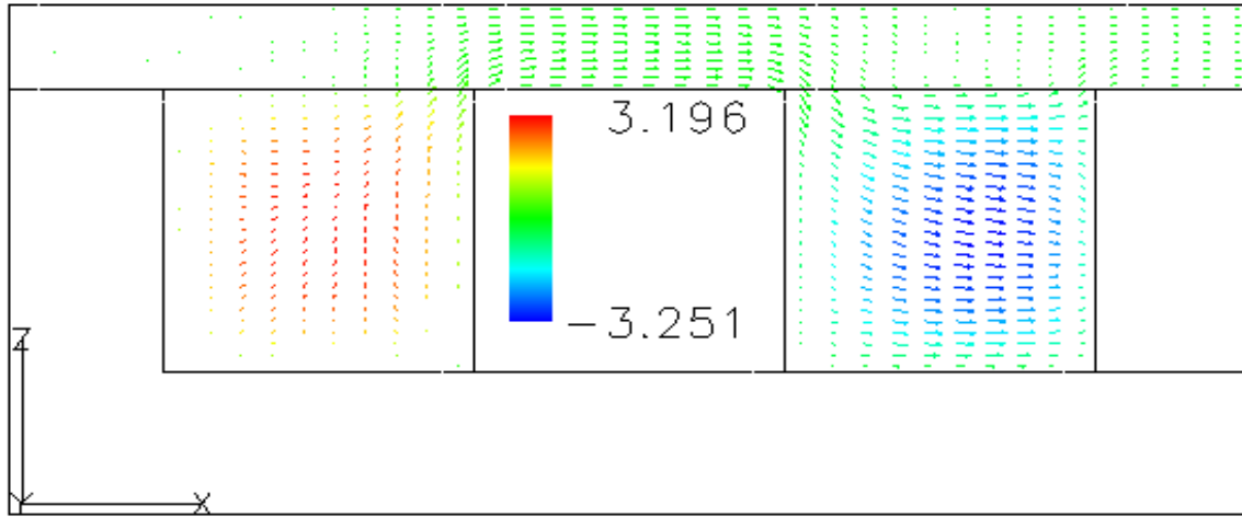
Fig. 3.5: Pressure (Pa) and velocity ( \text{m s}^{-1} ) distribution in the channel and GDL on the x-z plane at y=2 \text{ mm} with x=0 to x=4 \text{ mm}
