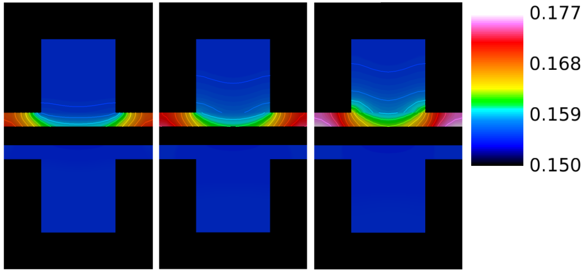
Fig. 5.13. Water concentration distributions (a) near to the inlet region (b) in the middle of the cell, and (c) near the outlet region for a high relative humidity (80%) and a current density of 0.1 \text{ A/cm}^2 .
