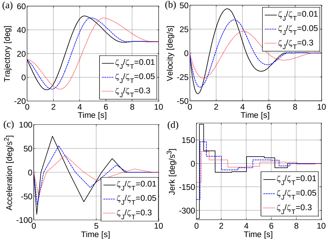
Fig. 2-20 Time responses of joint 2 for several kinds of \zeta_J/\zeta_T .
