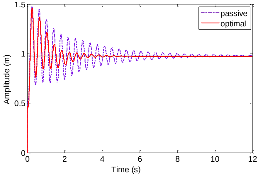
Fig. 4-10 Step responses of semi-active and passive suspensions.
