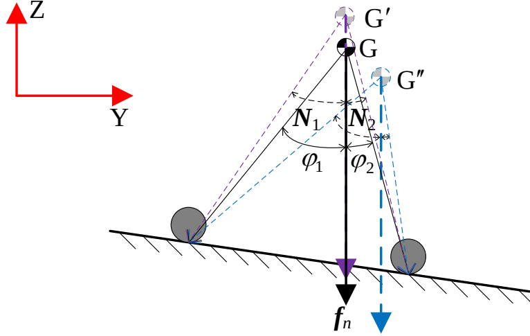
Fig. 4-3 Stability measure with a planar instance.
