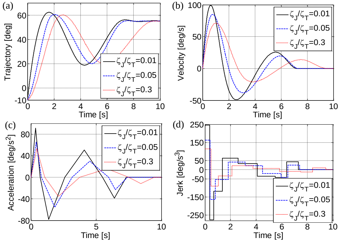
Fig. 2-18 Time responses of joint 0 for several kinds of \zeta_J/\zeta_T .
