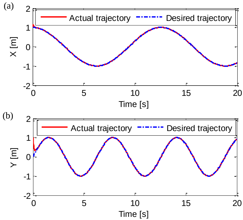
Fig. 3-5 Trajectory tracking of the robot. (a) In X direction, and (b) In Y direction.
