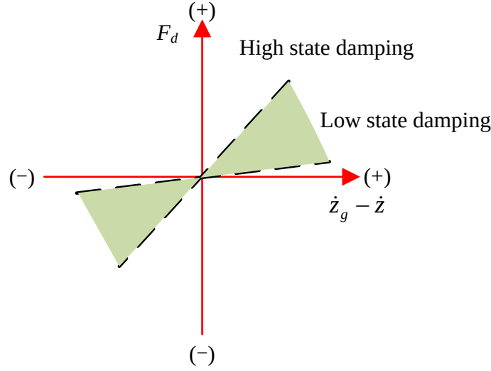
Fig. 4-6 Force-velocity characteristics of a continuously variable damper.
