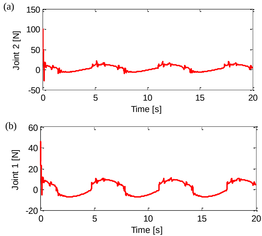
Fig. 3-15 Control input torque for each joint of the manipulator (case 2).
