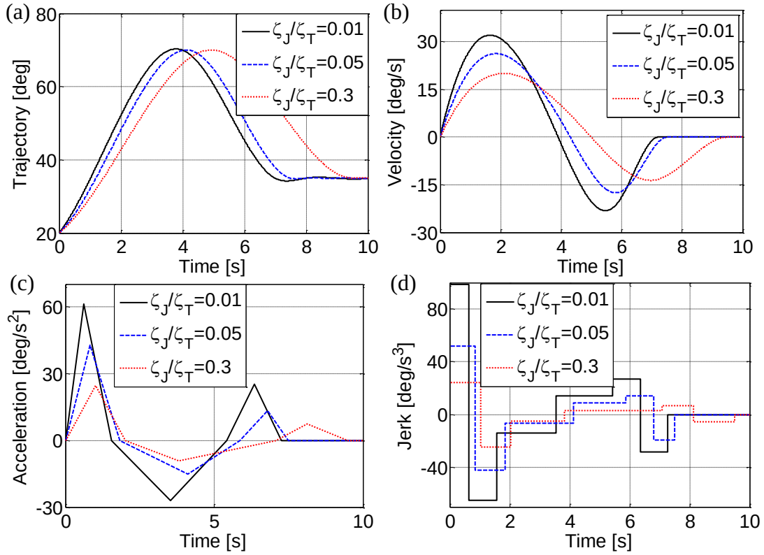
Fig. 2-19 Time responses of joint 1 for several kinds of \zeta_J/\zeta_T .
