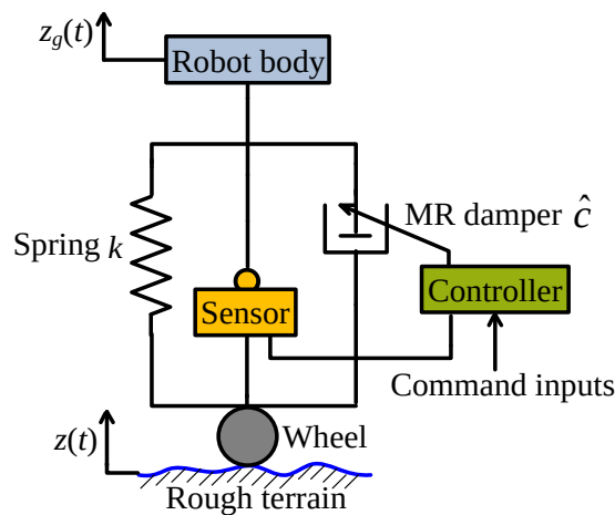
Fig. 4-5 Semi-active suspension system with a MR damper.
