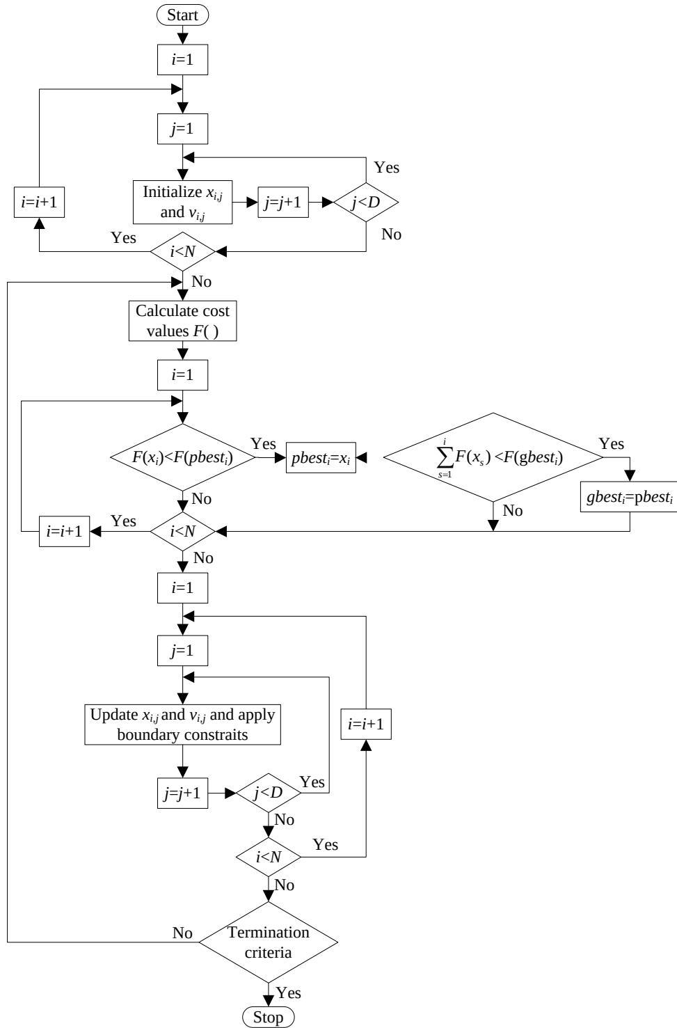
Fig. 4-7 Flow chart of the PSO algorithm.
