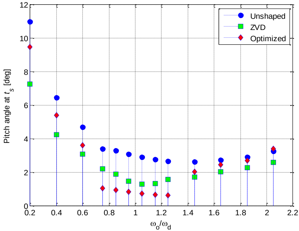
Fig. 2-10 Numerous trial results of pitch angle at settling time t_s vs \omega_o / \omega_d .
