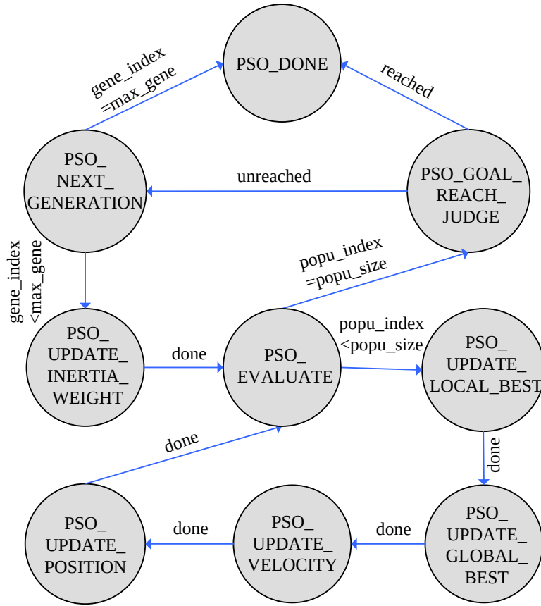
Fig. 2-2 Implementation of PSO based on a state machine.
