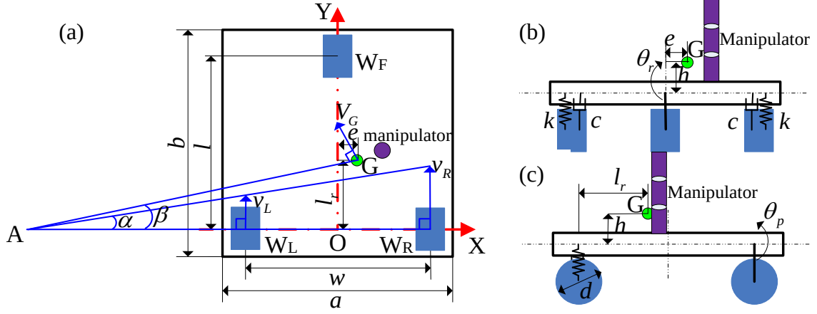
Fig. 2-5 Schematic drawings of suspended mobile robot with a manipulator.
