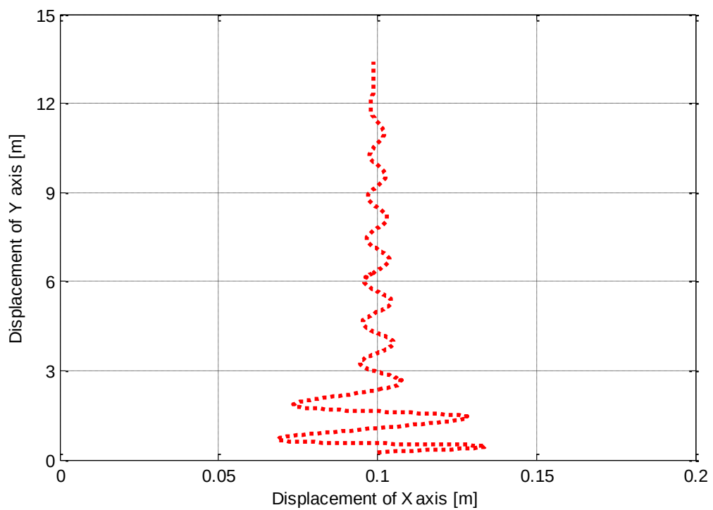
Fig. 2-15 Motion trace (projection on X-Y plane).
