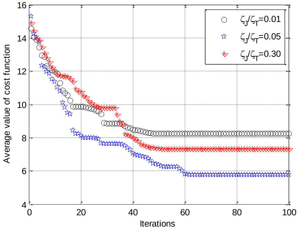
Fig. 2-21 Average value of cost function versus iterations for several kinds of \zeta_J/\zeta_T .
