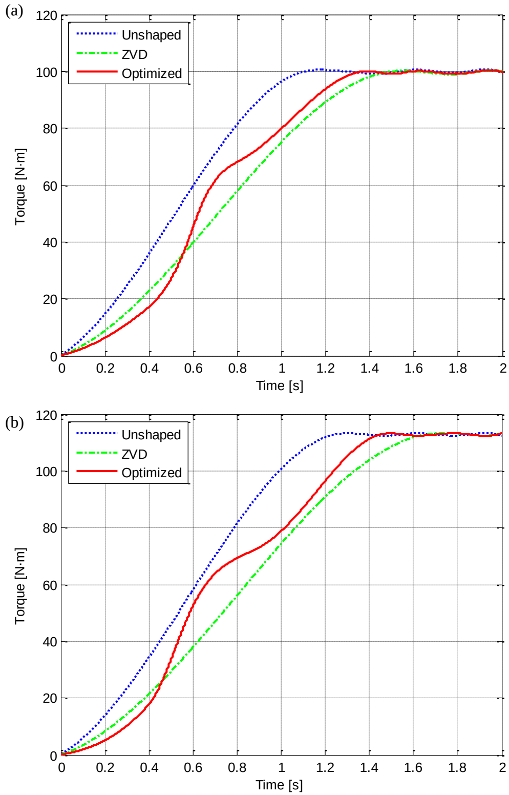
Fig. 2-7 Time history of control input torques.
