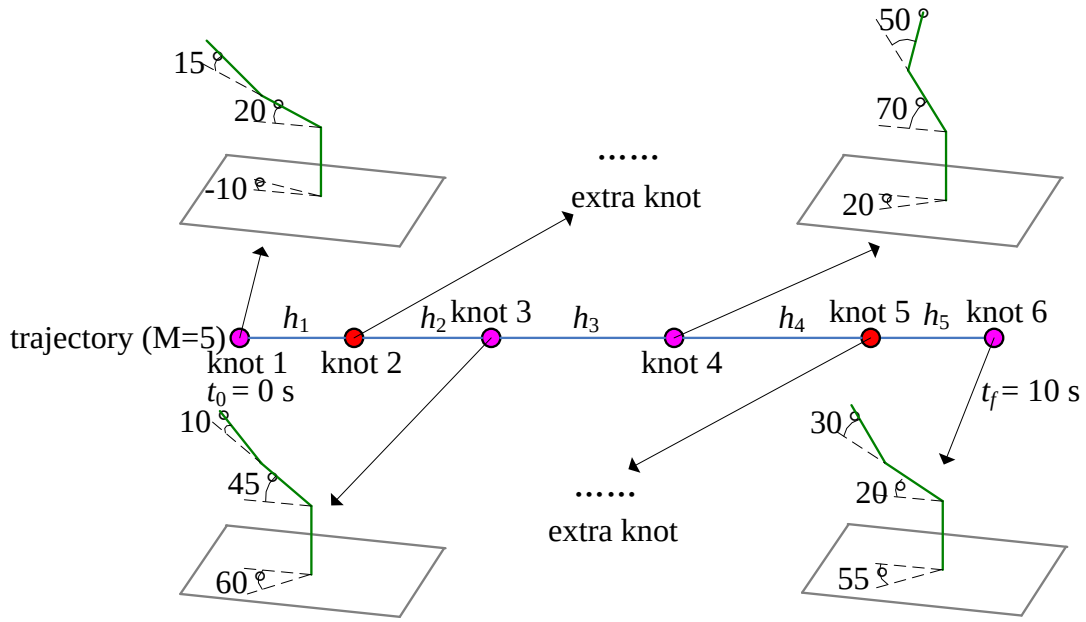
Fig. 2-17 Graphical representation of the trajectory with extra knots.
