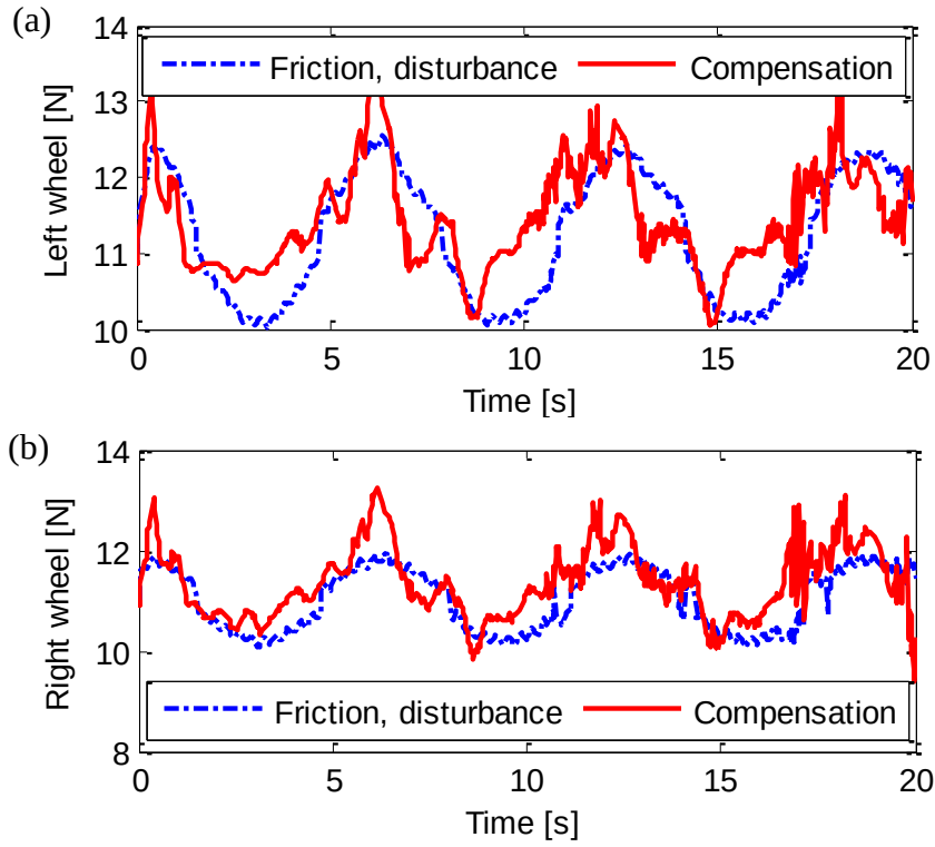
Fig. 3-16 Friction and disturbance for each wheel, and their compensation (case 2).
