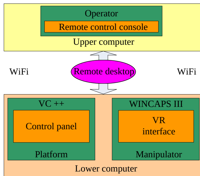
Fig. 5-7 Scheme of the proposed teleoperation system.
