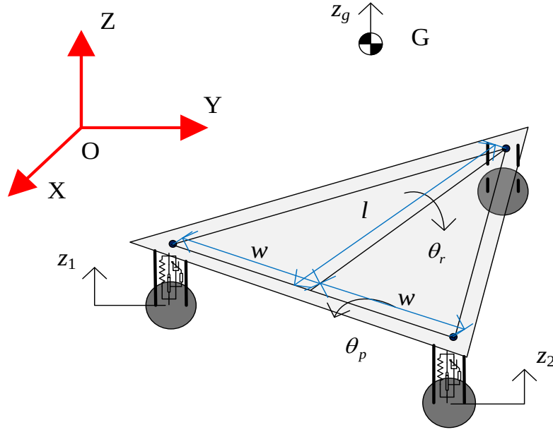
Fig. 4-2 Dynamic model of the robot with suspensions.
