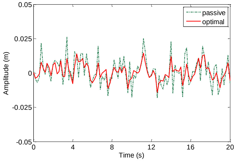
Fig. 4-13 Vibratory response of the robot in bounce motion.
