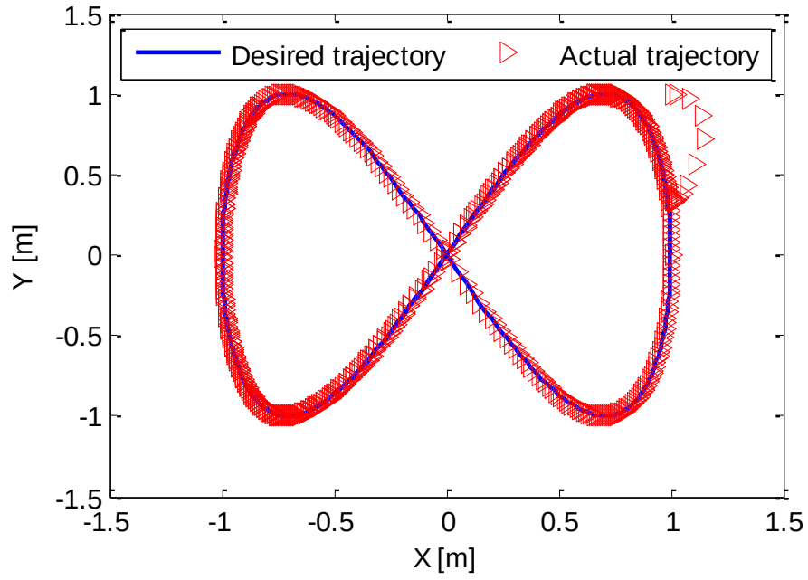
Fig. 3-4 Trajectory tracking of the robot in the absence of sliding.
