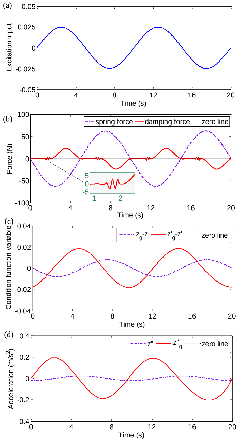
Fig. 4-9 Response of semi-active suspension. (a) sinusoidal input, (b) spring and damping forces, (c) condition function variables, and (d) accelerations.
