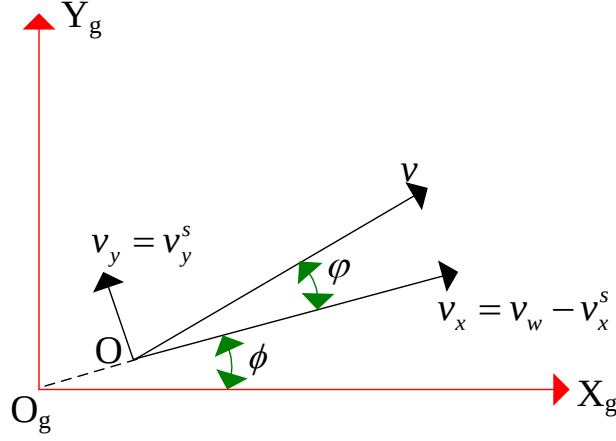
Fig. 3-3 Graphical representation of the parameters of robotic platform.
