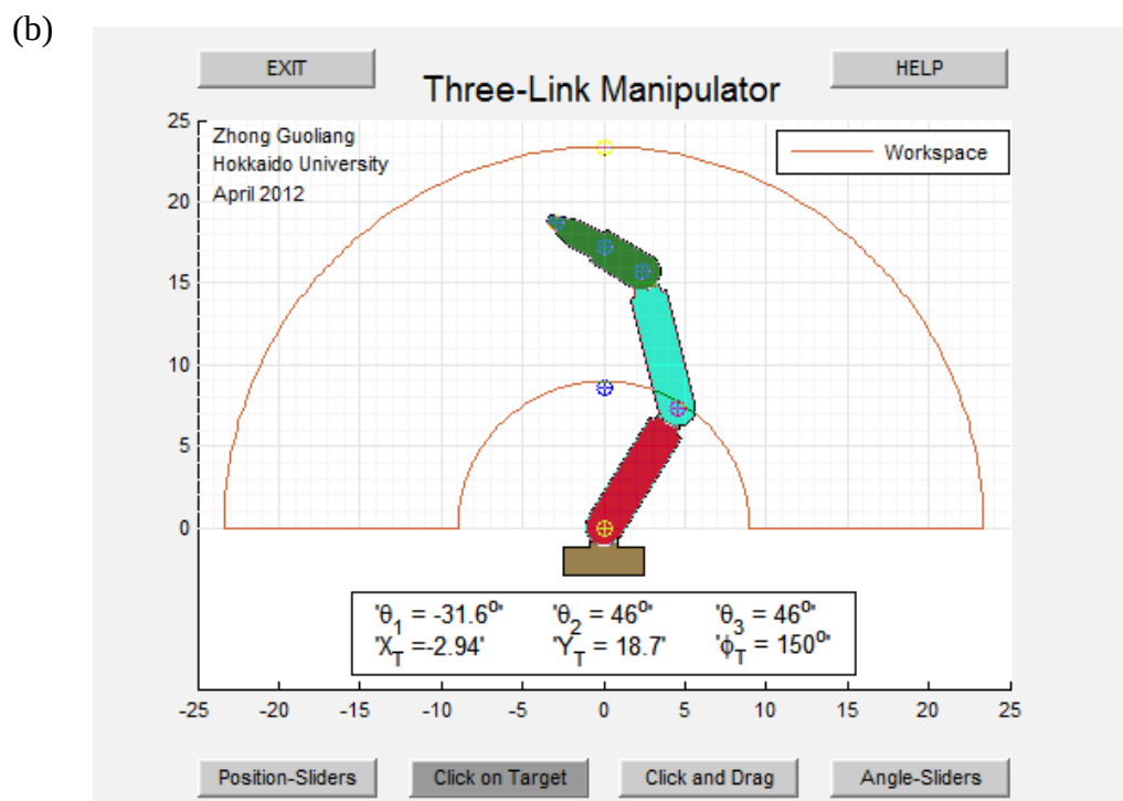
Fig. 5-6 Kinematics simulation of 3-link planar manipulator.
