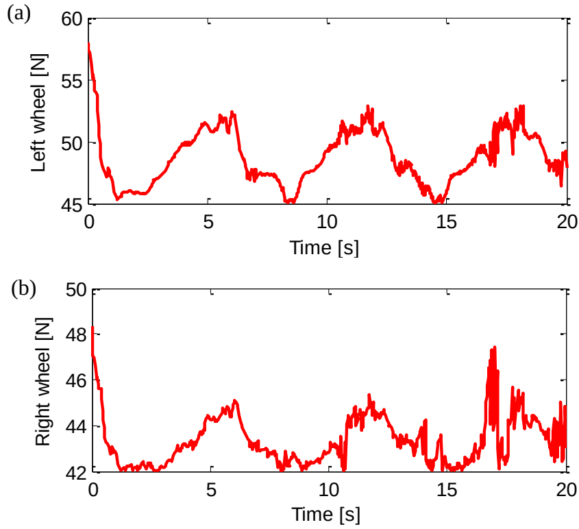
Fig. 3-17 Control input torque for each wheel (case 2).
