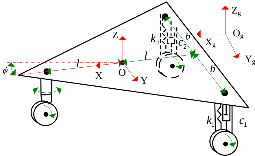
Fig. 3-2 Configuration of the robotic platform.
