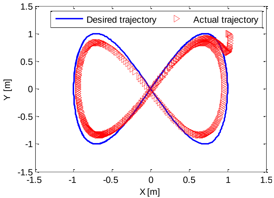
Fig. 3-7 Trajectory tracking of the robot in the presence of sliding.
