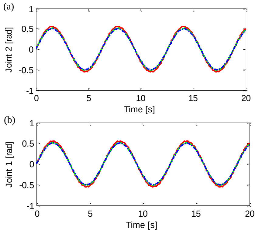
Fig. 3-10 Trajectory tracking of manipulator for cases 1 (—) and 2 (---). (a) Joint 2, and (b) Joint 1, desired trajectory (- · -).
