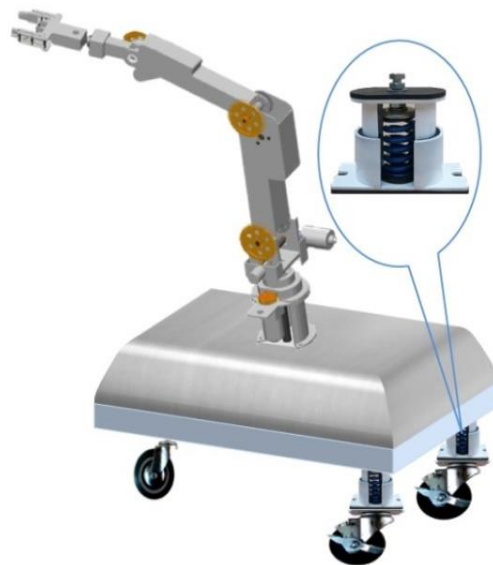
Fig. 2-1 Picture of suspended mobile robot with a manipulator.
