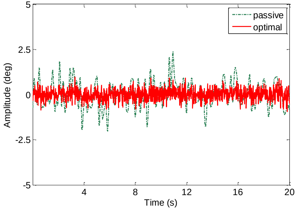
Fig. 4-15 Vibratory response of the robot in roll motion.
