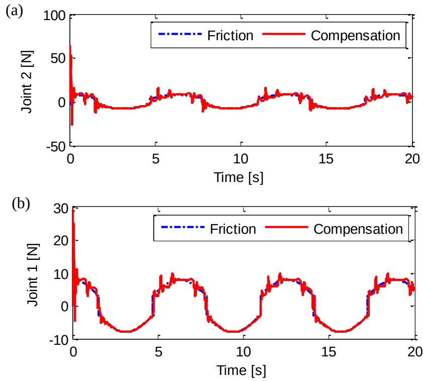
Fig. 3-14 Friction and its compensation for the manipulator (case 2).
