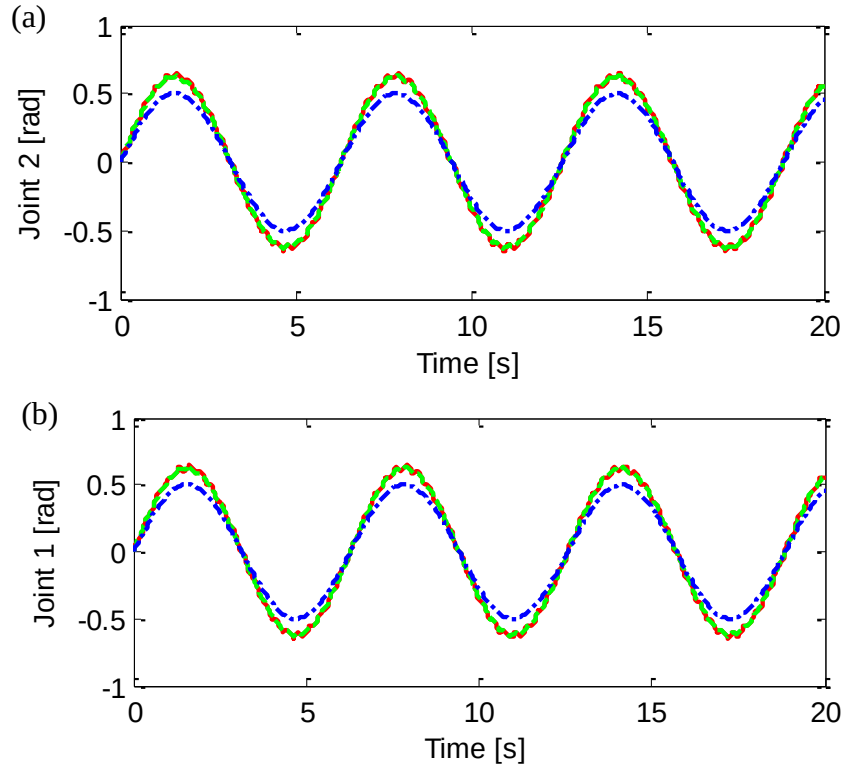
Fig. 3-11 Trajectory tracking of manipulator for cases 3 (—) and 4 (---). (a) Joint 2, and (b) Joint 1, desired trajectory (· · ·).
