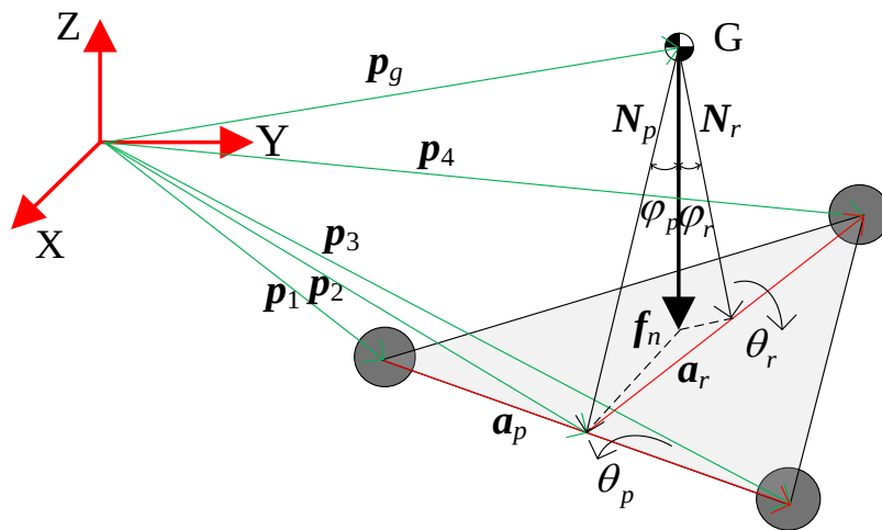
Fig. 4-4 Schematic diagram of stability measure.
