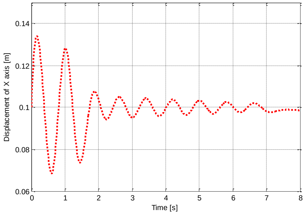
Fig. 2-14 Displacement of X axis (projection on T-X plane).
