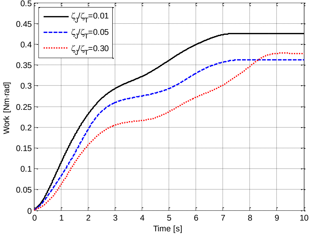
Fig. 2-22 Time history of control energy for several kinds of \zeta_J/\zeta_T .
