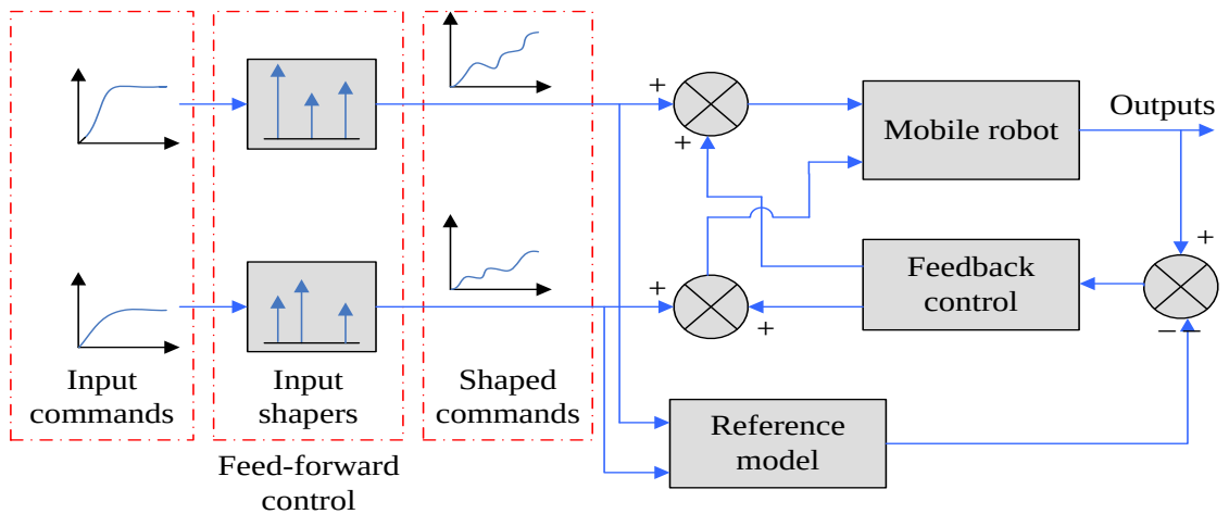
Fig. 2-6 Control scheme of the suspended mobile robot with a static manipulator.
