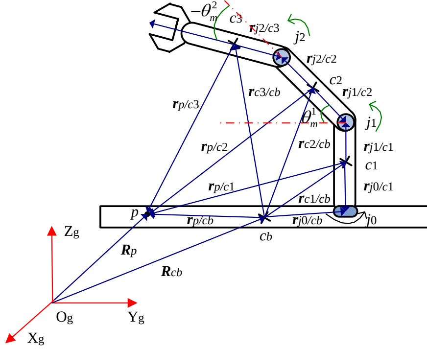
Fig. 2-16 Vector diagram of the suspended mobile robot with a dynamic manipulator for DPM concept.
