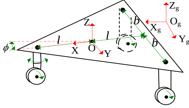
Fig. 5-5 Configuration of the robotic platform.
