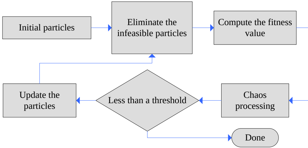
Fig. 2-4 Flow chart of PSO with chaos method.
