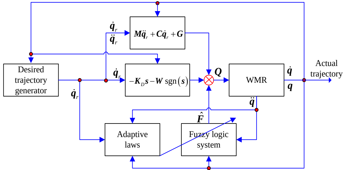
Fig. 3-8 Structure of the control scheme.
