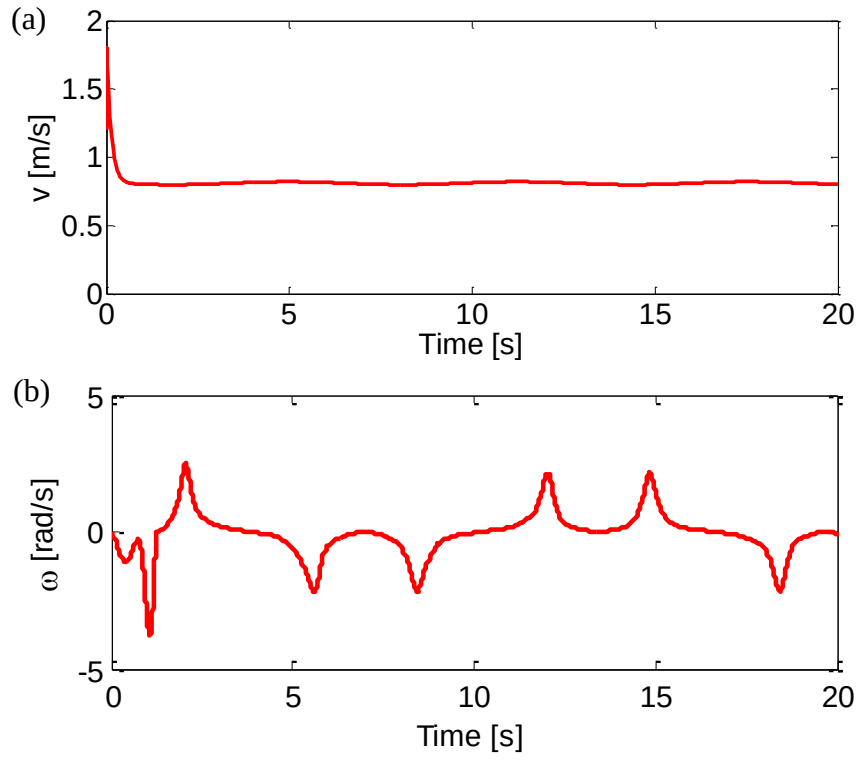
Fig. 3-6 Control inputs for the robot.
