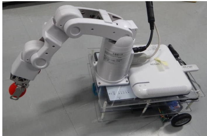
Fig. 4-1 Mobile robot system.
