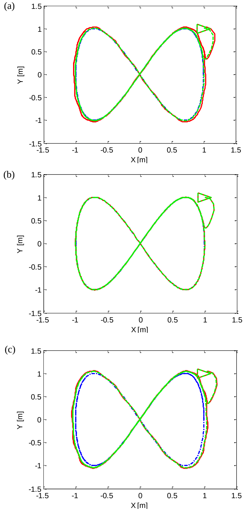
Fig. 3-13 Trajectory tracking of mobile platform for every case.
