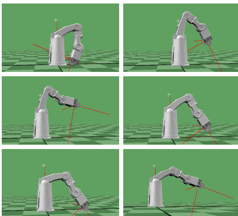
Fig. 5-12 Motion of the virtual manipulator when it grasps the ping-pong ball.
