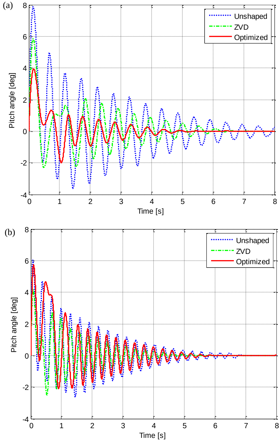
Fig. 2-9 Time responses of suspended mobile platform in pitch direction.
