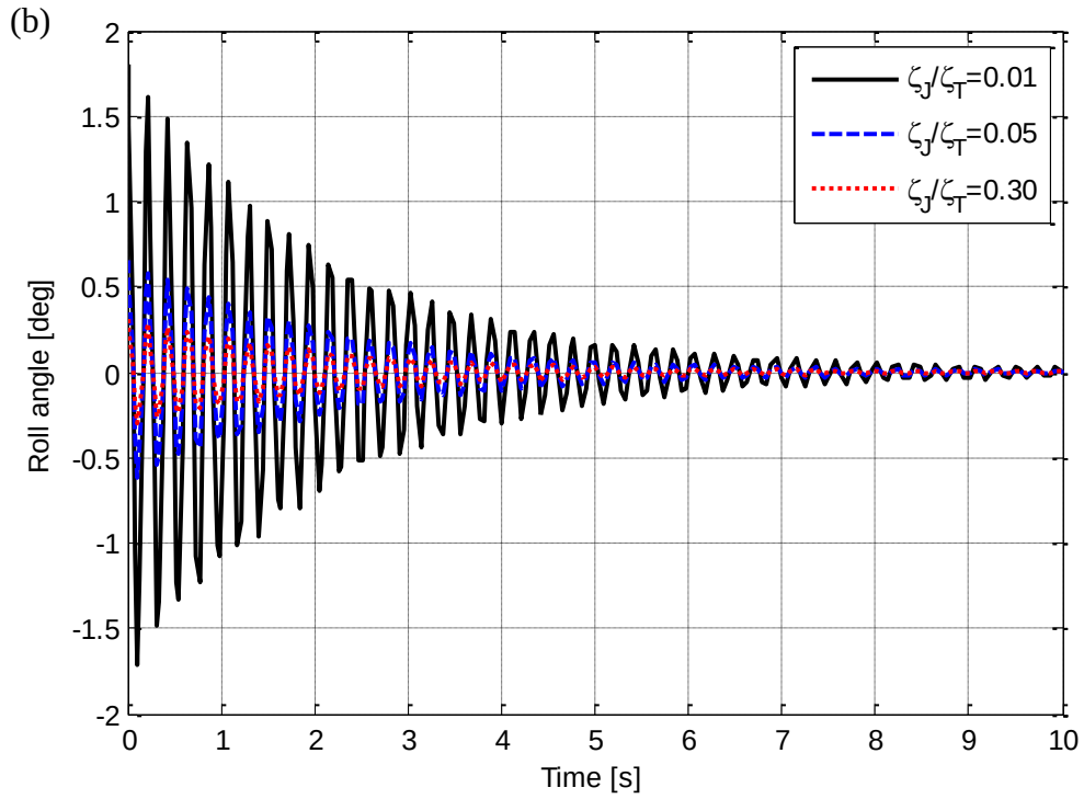
Fig. 2-23 Time responses of suspended mobile platform for several kinds of \zeta_J/\zeta_T .
