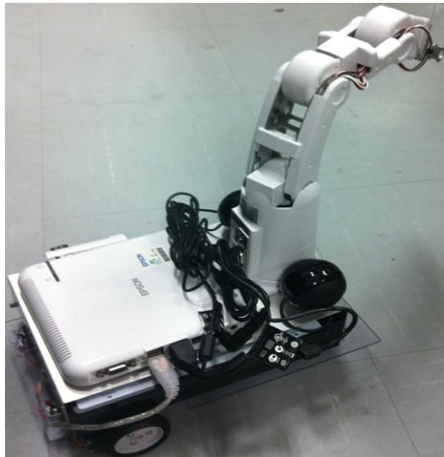
Fig. 3-1 Mobile manipulator system.
