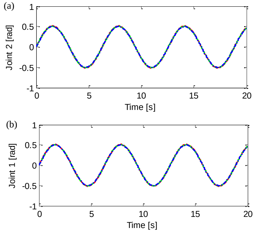
Fig. 3-12 Trajectory tracking of manipulator for cases 5 (—) and 6 (---). (a) Joint 2, and (b) Joint 1, desired trajectory (- · -).
