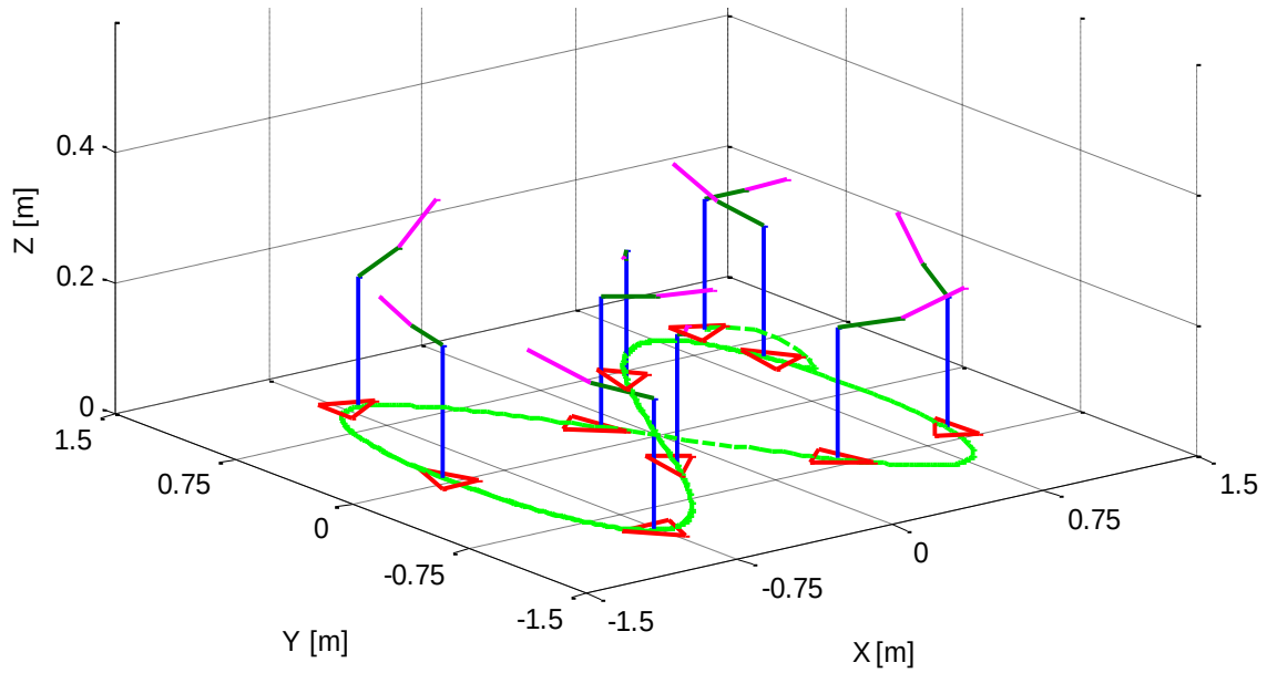
Fig. 3-9 Desired trajectories of manipulator and platform in 3D space.
