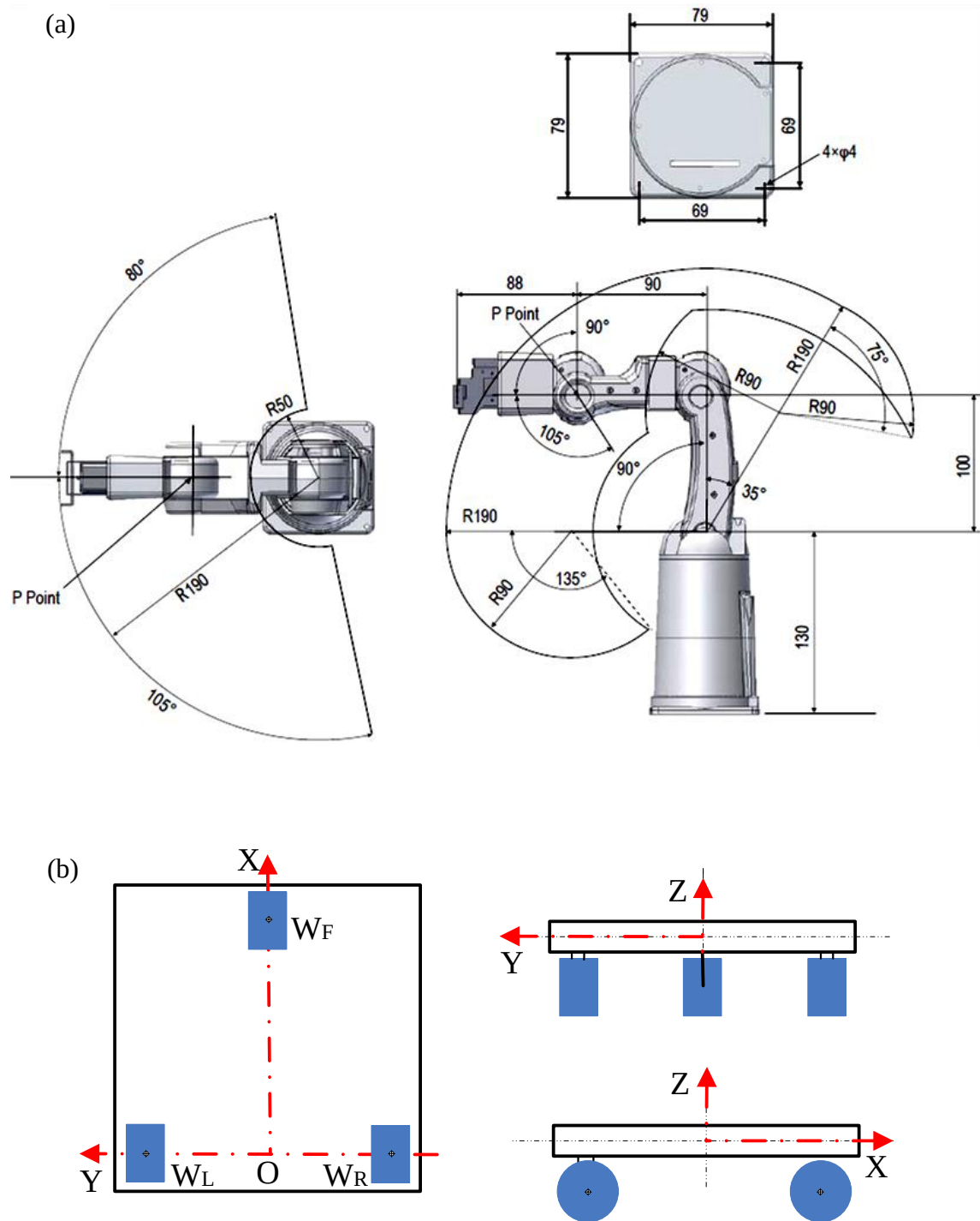
Fig. 5-3 Schematic diagram of the robot system.
