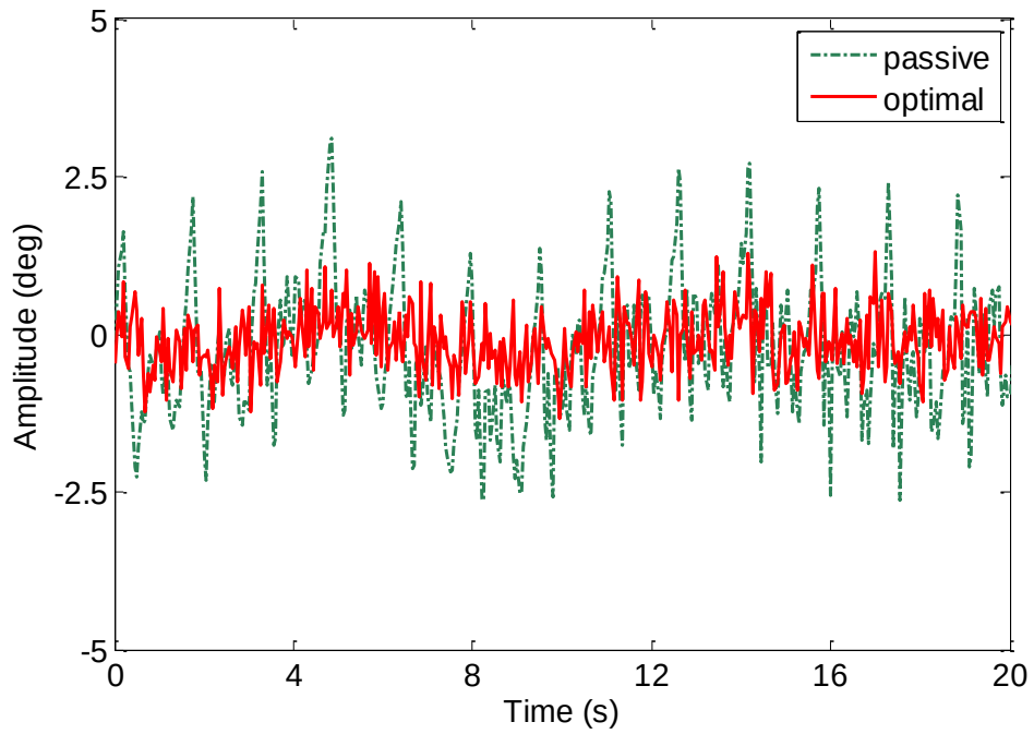
Fig. 4-14 Vibratory response of the robot in pitch motion.
