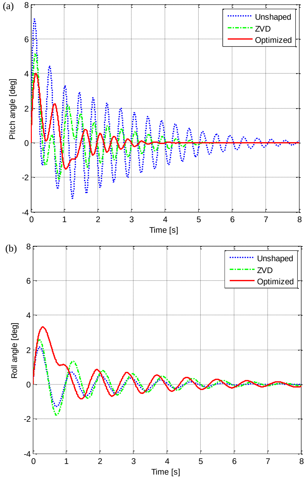
Fig. 2-8 Time responses of suspended mobile platform when \omega_o = \omega_d .
