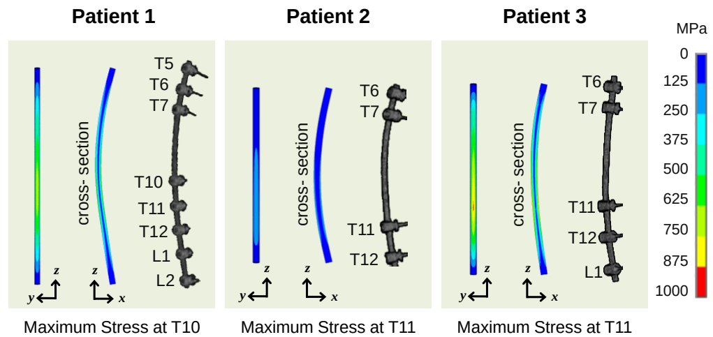
Figure 3.6 von Mises stress distribution of the deformed implant rod after the surgical treatment.
