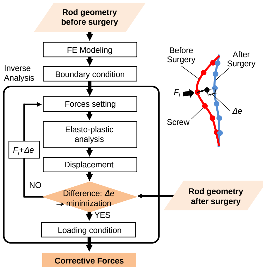
Figure 5.2 Procedure for corrective force analysis using FEA.
