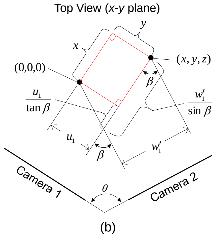
Figure 4.1 Three-dimensional reconstruction from different views. (a) Projection of points in image plane of each camera at different views (b) Geometric relation of points when viewed from the top.
