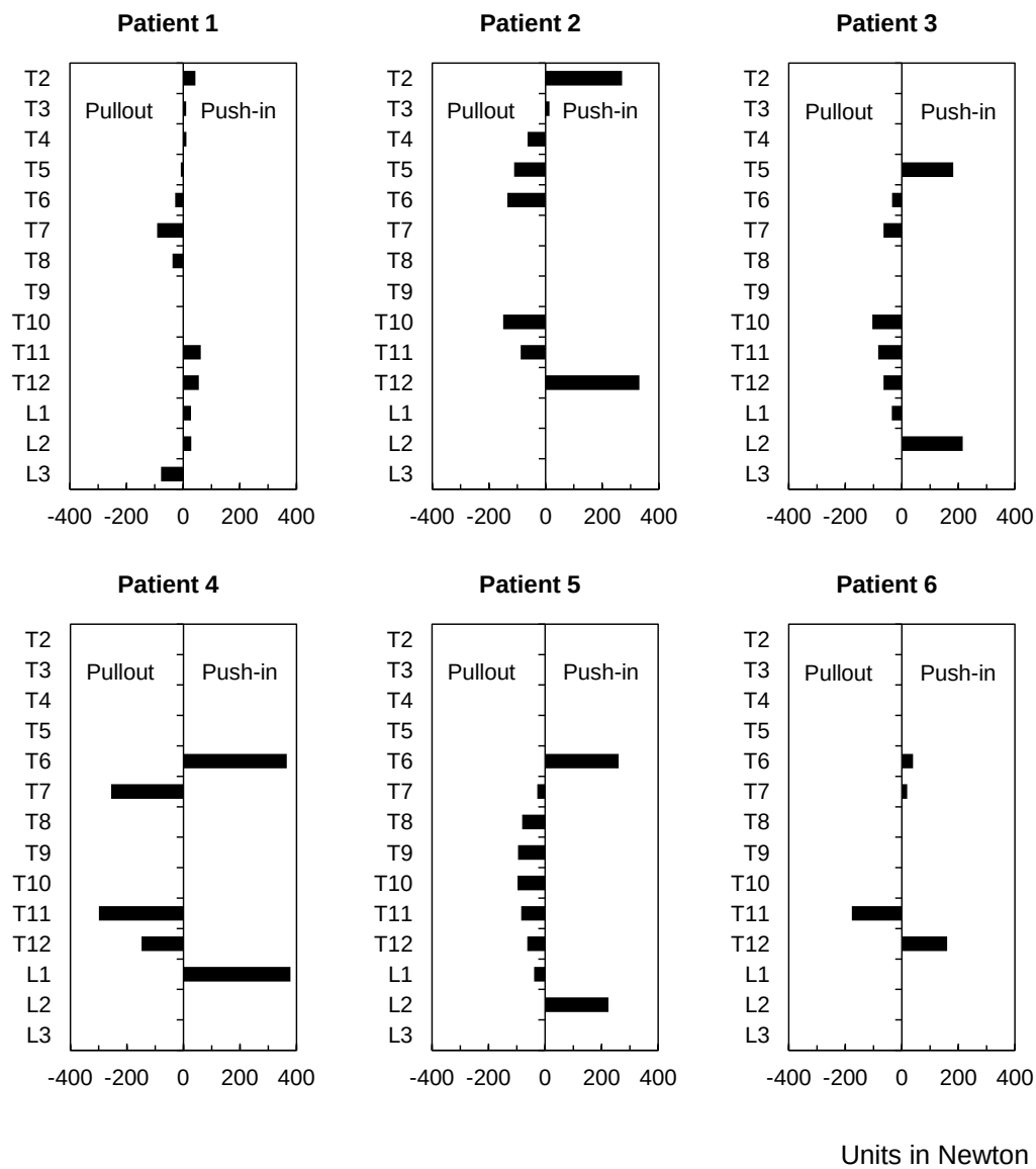
Figure 5.8 Pullout and push-in forces acting at the vertebra of each patient.
