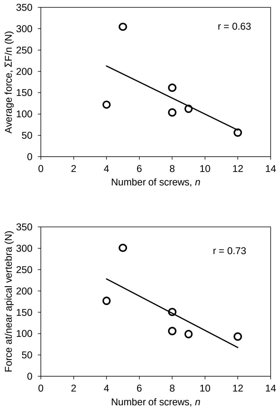
Figure 5.6 Relationships between the number of screws and magnitude of forces. Number of screws vs. average force (top). Number of screws vs. force at/near apical vertebra (bottom).
