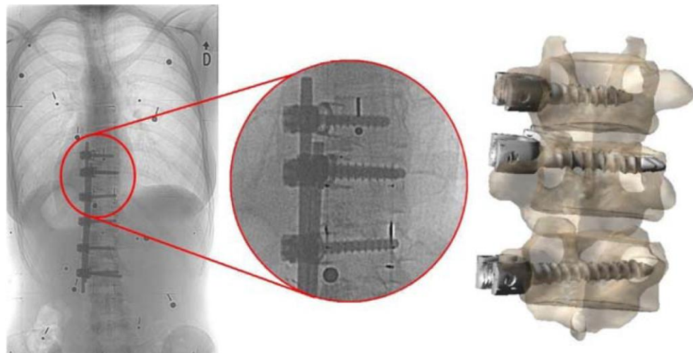
Figure 1.4 X-ray showing fixation of scoliosis deformity by implant rods and screws (left). Finite element model of the spine and implants to analyze the distribution of corrective forces using various instrumentation strategies (right) (Desroches et al., 2007).
