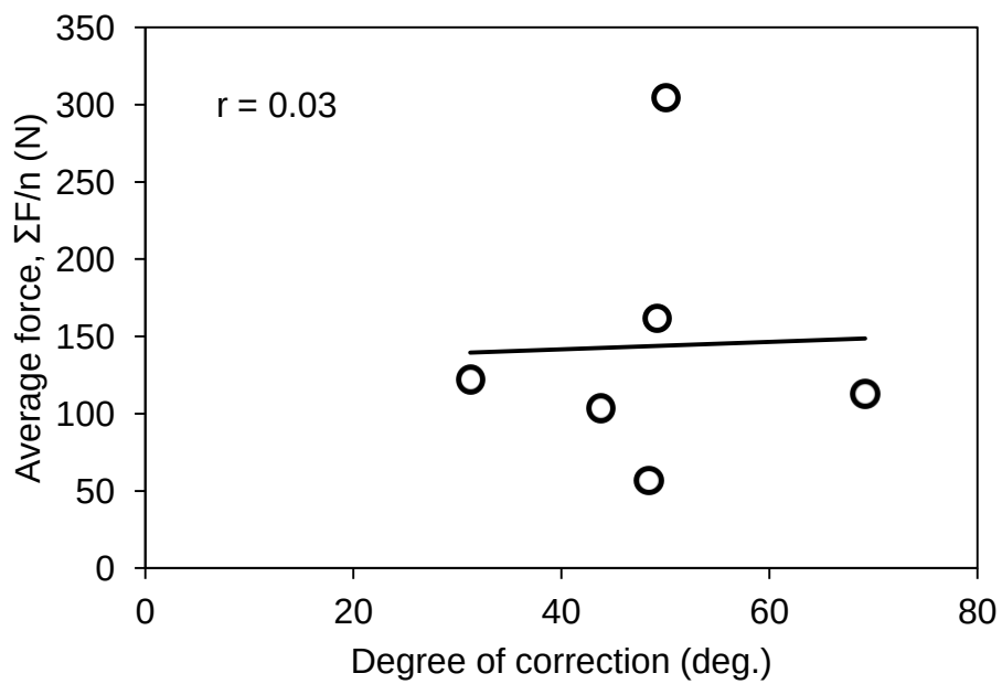
Figure 5.5 Relationship between the degree of correction and average force.
