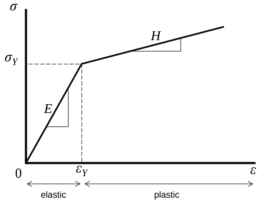
Figure 3.4 Bilinear elasto-plastic material model.
