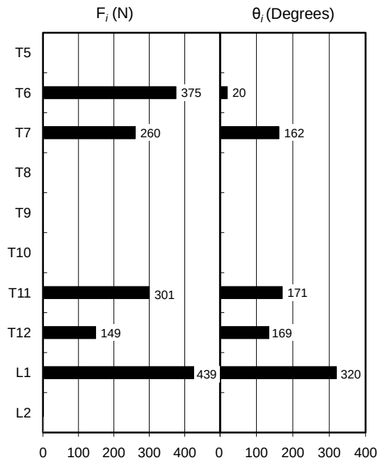
Figure 3.5 Magnitude of the three-dimensional corrective forces acting at each screw calculated from implant rod deformation.
