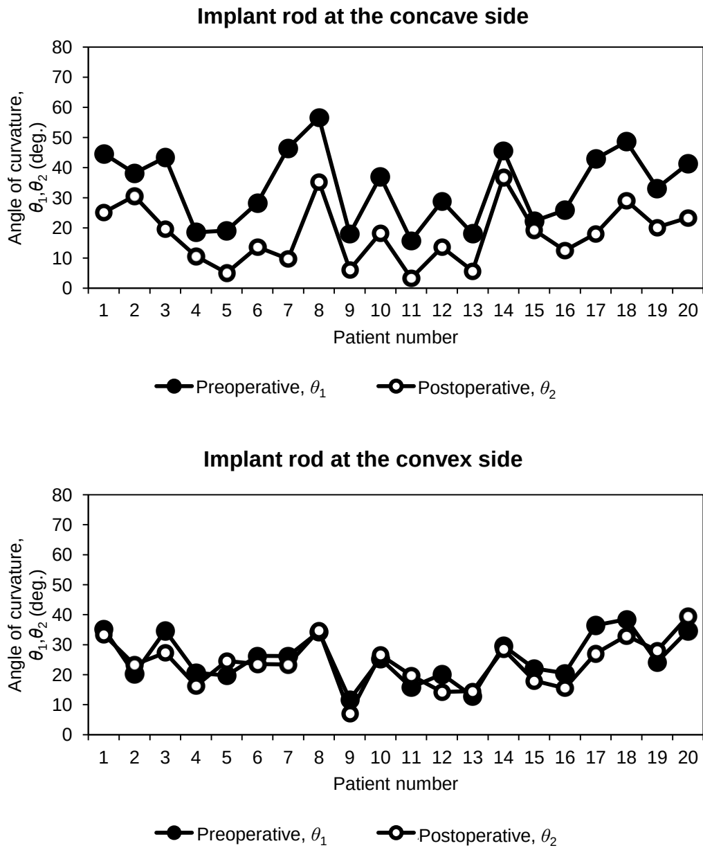
Figure 6.2 Preoperative and postoperative implant rod angle of curvature at the concave and convex side of deformity.
