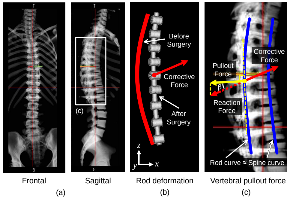
Figure 5.1 (a) Postoperative radiograph of operated scoliotic spine. (b) Corrective force acting at the screw of deformed rod. (c) Pullout force computed from the reaction force of corrective force.
