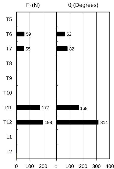
Figure 3.5 Magnitude of the three-dimensional corrective forces acting at each screw calculated from implant rod deformation.
