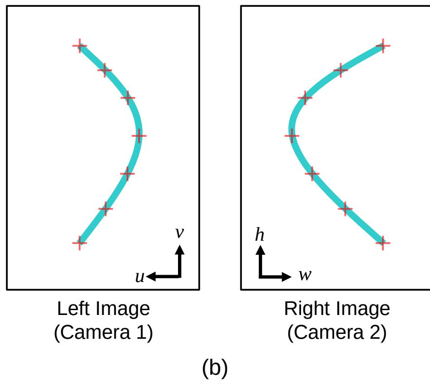
Figure 4.2 (a) Curved implant rod in space projected at different views. (b) Selected points (arbitrary) from inferior to superior endpoint in left and right images of rod for quintic polynomial curve fitting.
