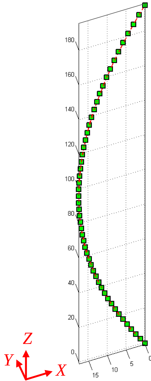
Figure 4.5 Typical reconstructed three-dimensional geometry of spinal rod using dual-camera system. It can be seen that the distance of points in y-axis is almost zero. This is in agreement with the actual spinal rod geometry.
