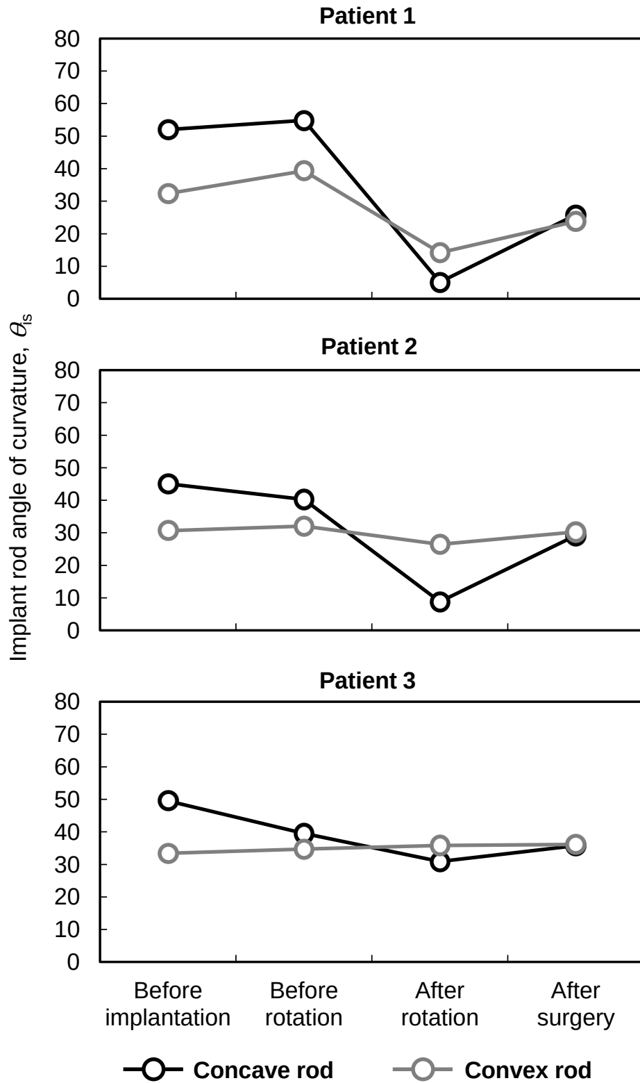
Figure 7.5 Implant rod angle of curvature of each patient.
