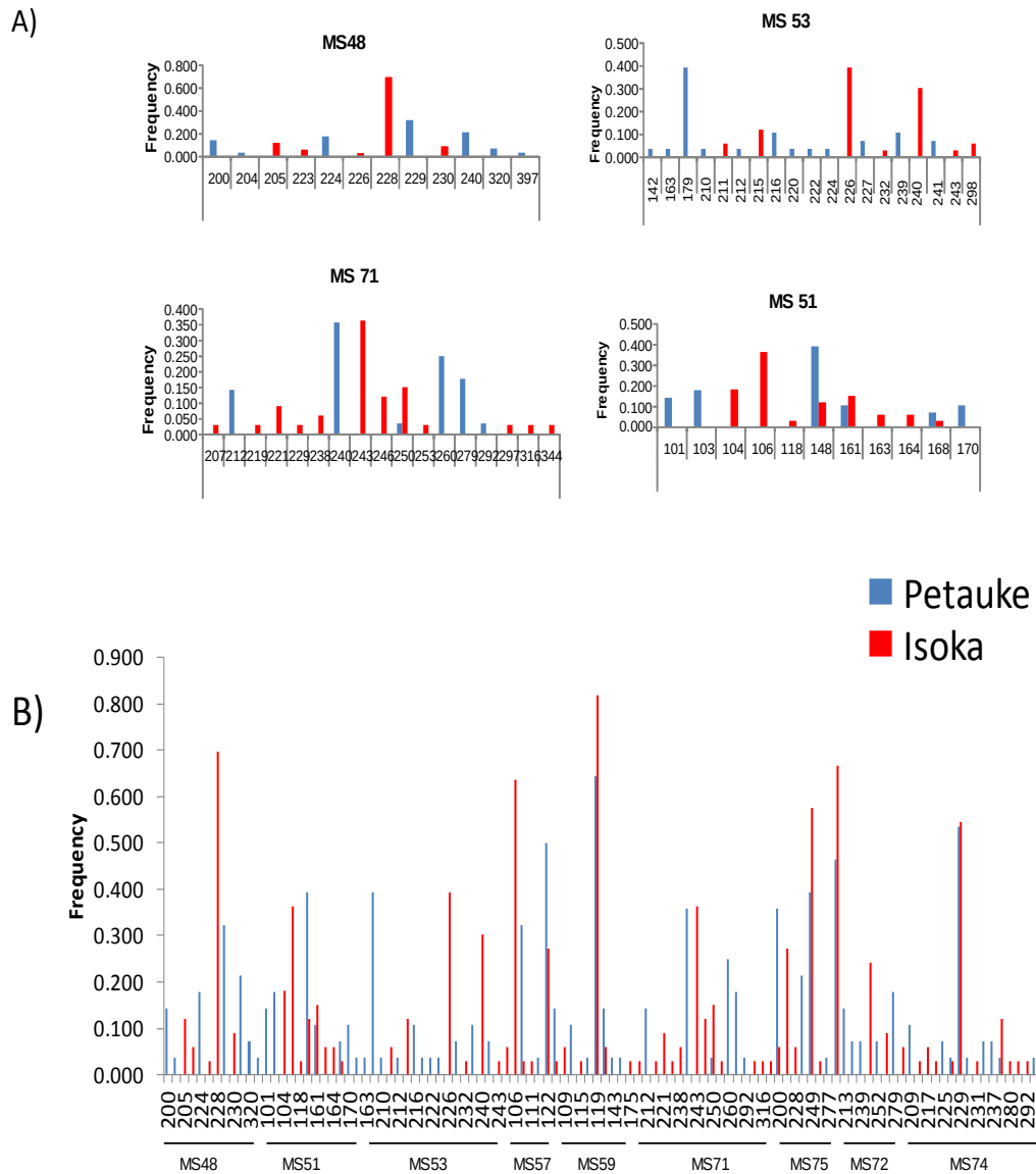
Figure 3 The allele frequencies of alleles in field populations of Theileria parva from Petauke and Isoka districts of Zambia. The frequency of each predominant allele in the samples from the Petauke and Isoka populations was calculated and presented in the form of histograms. (A) The results for MS48 and MS53 show the presence of unique alleles and the absence of shared alleles. The remaining loci generally show a greater proportion of unique alleles as compared to shared alleles, as represented by MS71 and MS51. (B) The overall allele frequency in both populations shows a greater number of unique alleles and a reduced number of shared alleles. Multi-locus genotype (MLG) data was used to generate the histograms. The frequency of each predominant allele was calculated as a proportion of the total of each marker.
