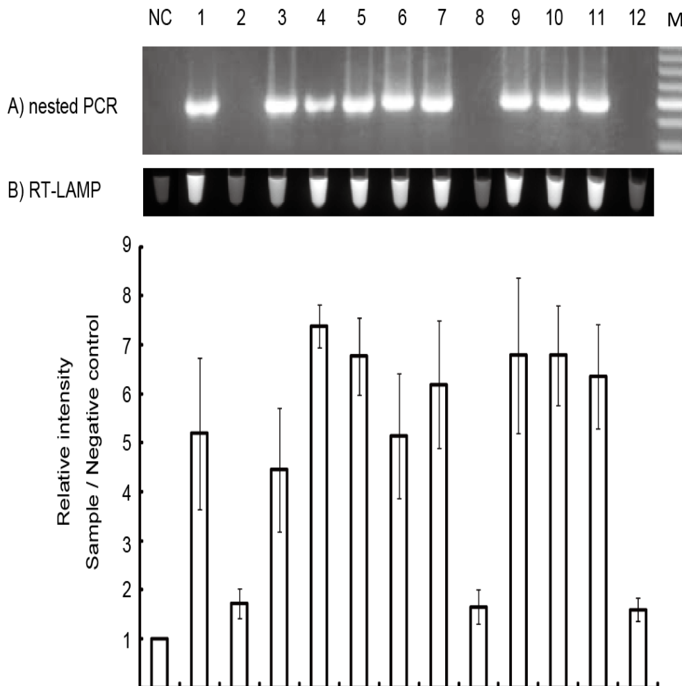
Figure 7 (A) Nested PCR results showing positive reactions for samples 1, 3–7, and 9–11. (B) (upper panel) Visual RT-LAMP results showing fluorescence in positive reaction tubes 1, 3–7, and 9–11. (middle panel) A bar graph indicating the relative fluorescence intensity of the RT-LAMP reaction assay. The relative fluorescent intensity of the examined samples was calculated as follows: The intensity of the examined sample was divided by the average intensity of samples without the RNA template. The 2-fold increase in signal intensity compared to that of the negative control represents the threshold of this assay. The relative fluorescence intensities were measured using the VersaDoc MP 4000 imaging system (Bio-Rad Laboratories, USA). (lower panel) Gel electrophoresis showing similar band patterns of the RT-LAMP reaction. 1–12 represents rabies clinical samples, M: the 100 bp molecular marker, NC: the negative control.
