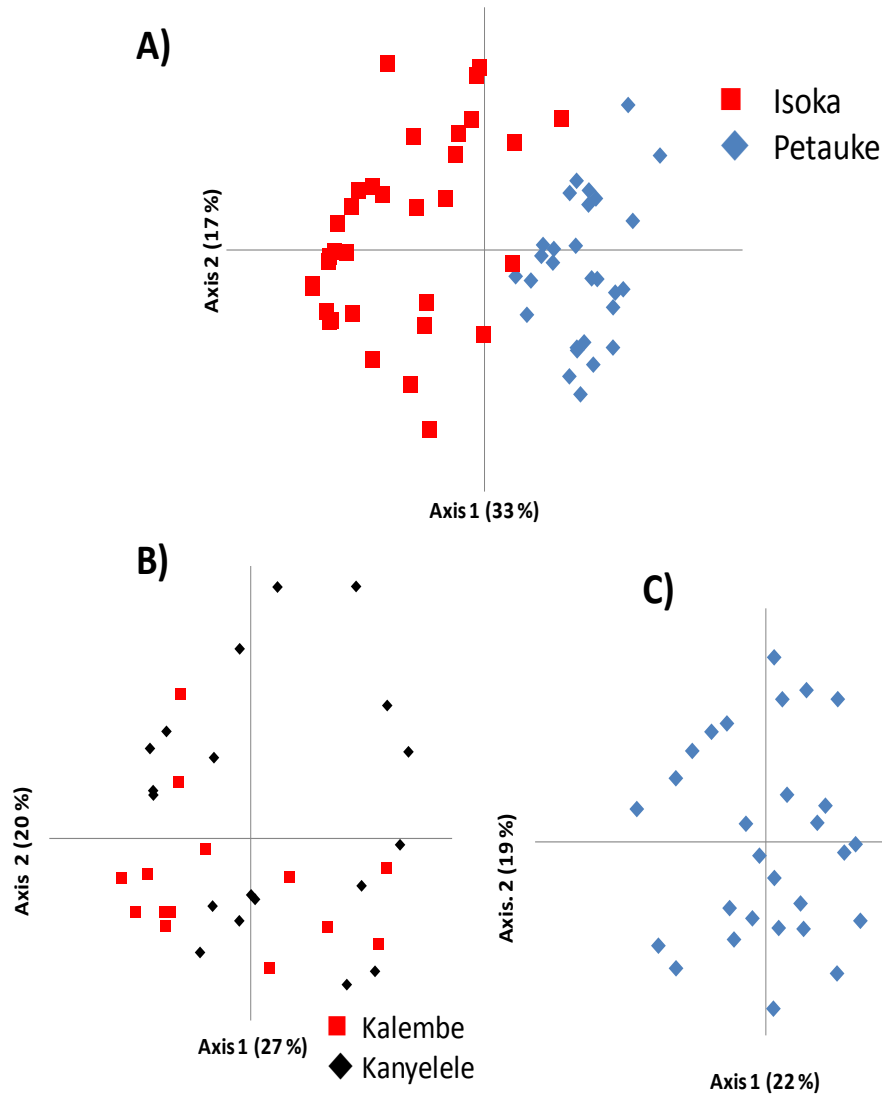
Figure 4 Principal component analysis (PCA) of T. parva populations from Petauke and Isoka districts of Zambia. The proportion of variation in the population dataset explained by each axis is shown in parentheses. PCA was performed using multi-locus genotype data from Petauke and Isoka districts. (A) Geographical sub-structuring between populations from Petauke and Isoka districts. (B) Homogenous population from Isoka district with the Kanyebele population showing more diversity by occupying all 4 quadrants while the Kalembe population occupies only 3 quadrants. (C) Saukani population from Petauke district.
