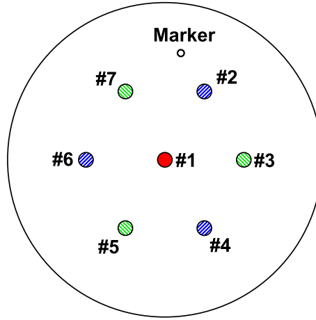
Fig. 2.17: Schematic cross-section of the designed heterogeneous MCF.
