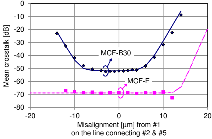
Fig. 7.6: Relationships between the misalignment and the mean crosstalk. Marks: the measured values, lines: the calculated values.
