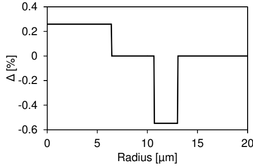
Fig. 5.1: A design profile of relative refractive index difference \Delta . A refractive index of the cladding was taken as the reference of the relative refractive index difference \Delta .
