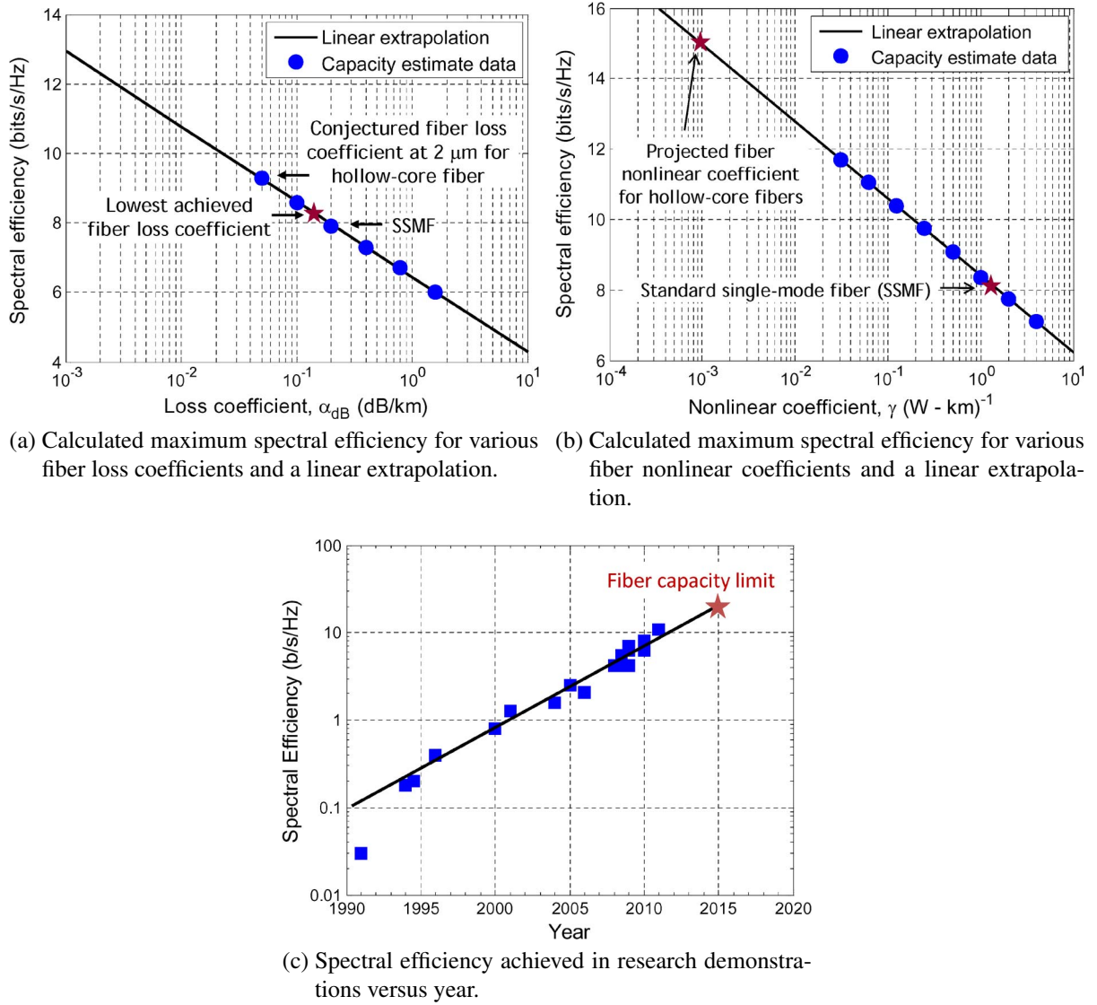
Fig. 1.4: Calculated limit of spectral efficiency. (Reproduced from Ref. [3] © 2012 IEEE.)
