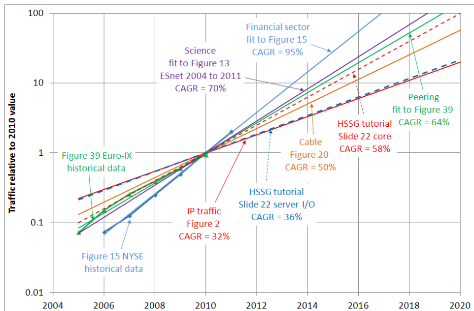
Fig. 1.1: Relative traffic increase normalized to 2010. (Reproduced from Ref. [1] © 2012 IEEE.)
