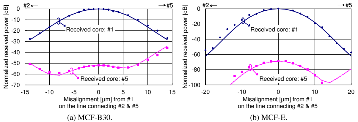
Fig. 7.5: Powers received from each of Core 1 and Core 5 with the input-end misalignment, which is shown in Fig. 7.1. Marks: the measured values, lines: the calculated values shown in Figs. 7.3c and 7.3d.
