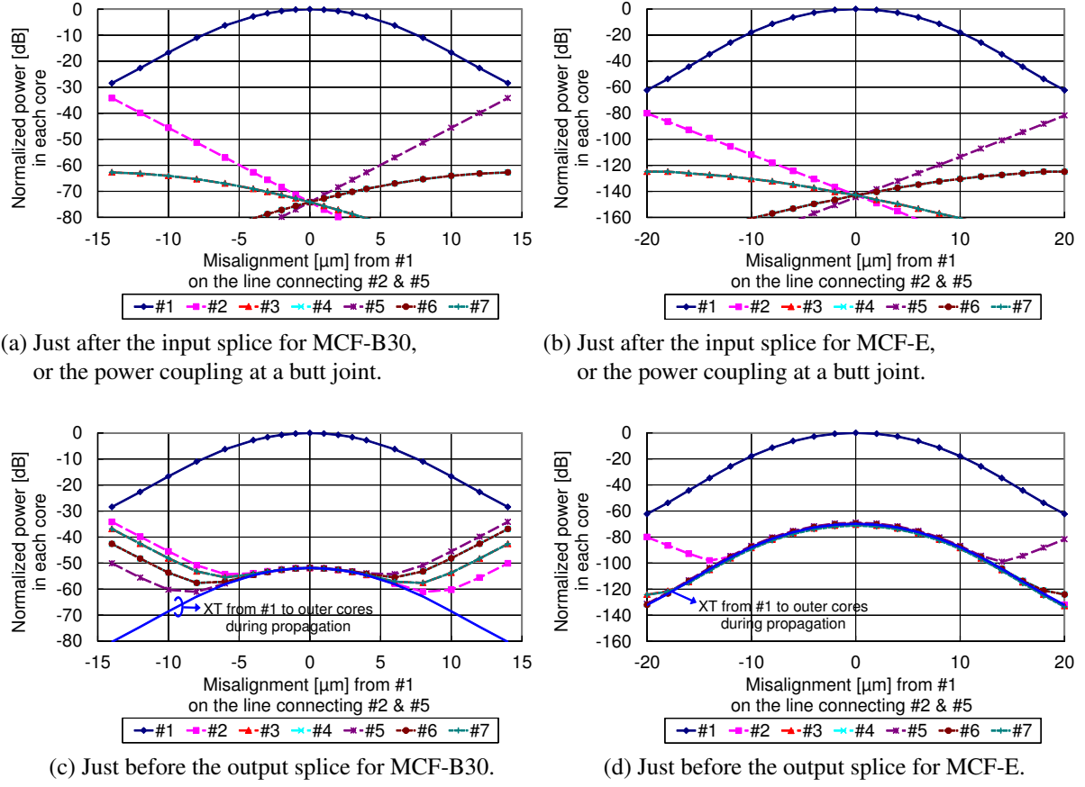
Fig. 7.3: Calculated power in each core of the MCFs with the misaligned excitations. Note that the scales are different between the left and the right graphs
