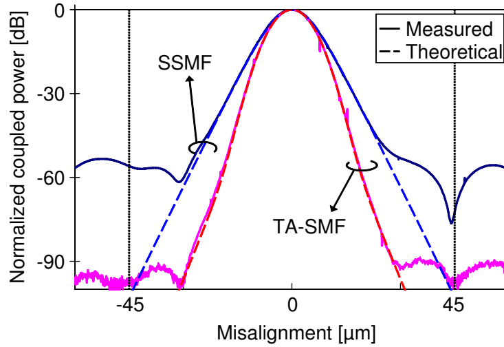
Fig. 3.10: Normalized power coupled at a butt joint between two single-core SMFs at 1550 nm.
