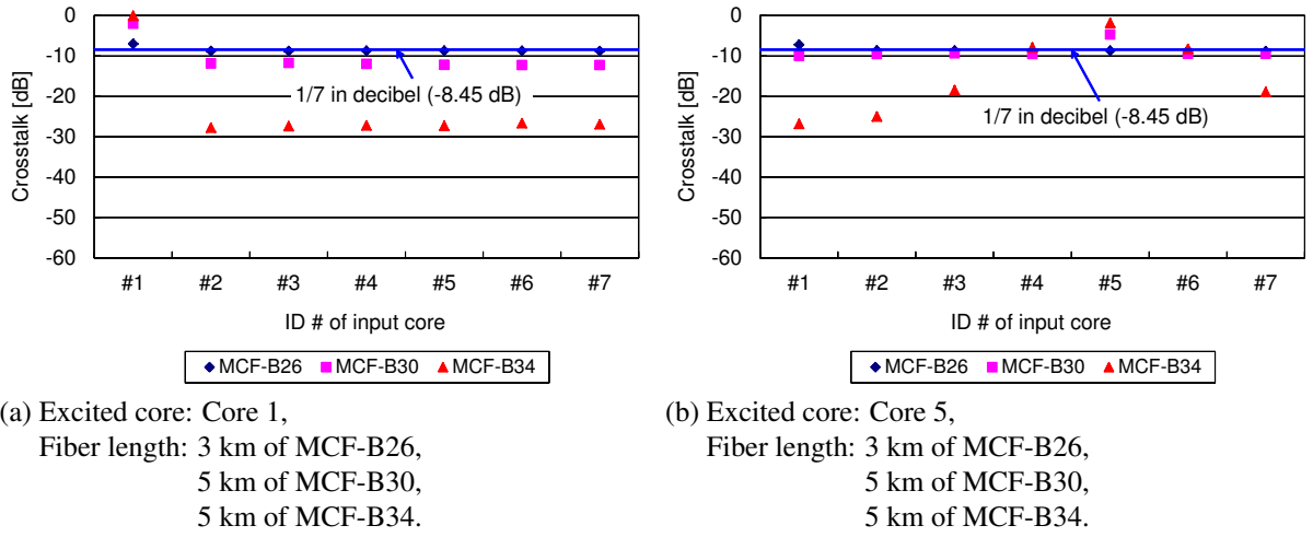
Fig. 2.11: Crosstalk of MCF-B wound on 140-mm-radius bobbin, measured at \lambda = 1550 nm.
