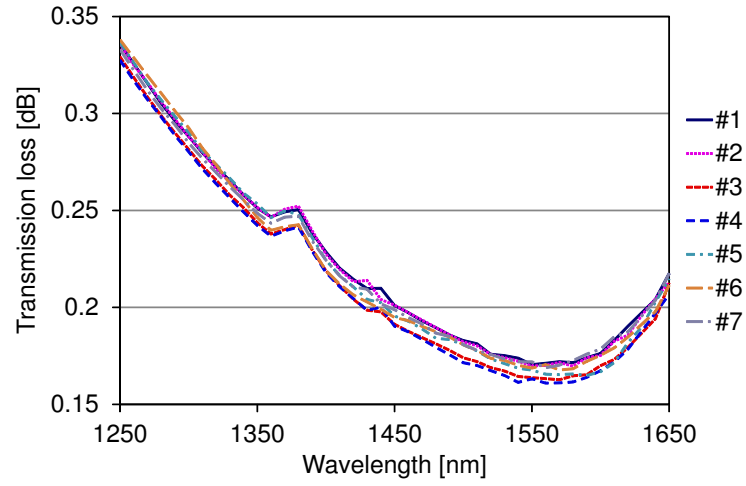
Fig. 5.4: Transmission loss spectra of the individual cores of MCF-F.
