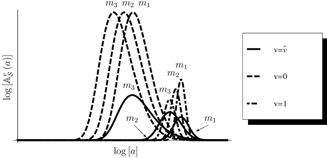
Figure 9: Transition of the mature age distribution. Whenever m becomes large ( m_1 < m_2 < m_3 ), the mature age distributions of every utilization behavior are shifted to younger ages than those under smaller m as in [11]. If the fittest species is a generalist, the change in distribution becomes extreme. Then, the age distribution is provided by Appendix I. We chose \phi(y) = Ry^l / (x_c^l + y^l) as the fertility rate function. This function has a unique m with respect to x , and the optimal body size, x_{opt}^* , is obtained by calculating the derivative of (\log [\phi(x_{opt}^*)] / \log [x_{opt}^*/x])' = 0 with respect to x_{opt}^* . We substitute the RHS of that equality into x of the distribution. Then, we obtain this figure by changing x_{opt}^* . Then, m becomes inversely proportional to x_{opt}^* in this fertility function. Parameters are R = 10 , x_c = 1.0 , l = 2 , x_{opt}^* = 1.1, 1.3, 1.5 , with the others being the same as in Fig. 8.
