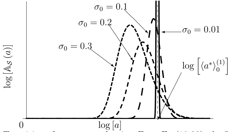
Figure 4: Transition of mature age density. From Eq.(10.22), the figure shows a transition of mature age density \mathbb{A}_{\mathcal{S}}(a) with respect to \sigma_0 in a double logarithmic plot. Increases in \sigma_0 yield many individuals whose maturities are fast and a few individuals with slow maturity. In other words, higher stochasticity leads to many individuals with short life spans. Parameters are \gamma = 0.1 , \mu_0 = 0.04 , x = 0.43 , x^* = 0.9 and \sigma_0 = \{0.01, 0.1, 0.2, 0.3\} .
