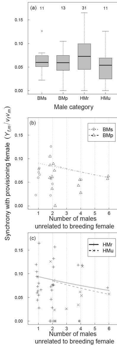
Figure 2.3. Synchrony between males and the breeding female characterized by ratio of perceived ( Y_{f,m}/v_f ) to actual male provisioning rate ( v_m ). The ratio is low because the synchronous visits/h was divided by hourly visit rates of both males and the breeding female rather than just one of them. This was done to control for the visit rate of both individuals in each dyad. (a) Box plot shows median, interquartile range and approximate 2.5–97.5 percentiles of observed data. Circles represent outliers. The numbers at the top denote the sample size for each male category. (b-c) Relationships between patterns of synchrony and the numbers of males in the breeding unit that were unrelated to the breeding female for breeding (b) and non-breeding (c) males. Non-significant trend lines predicted by median estimates of the latent space model cover ranges of the number of unrelated males observed for each category. Acronyms for male category are provided in Fig. 2.1 legend. Data points are jittered along x axis. Vertical grey dotted lines show the true positions of values on the x-axis.
