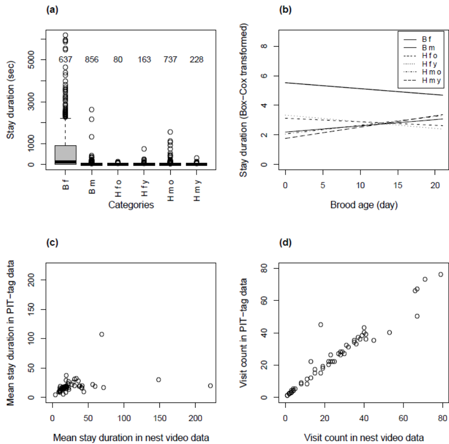
Figure 1.2. (a) Differences in stay duration across different categories: breeding males: median = 13 s, IQR = 5 -24 s; adult helper females: median = 16 s, IQR = 11 -24 s; younger helper females: median = 15 s, IQR = 7 -22; adult helper males: median = 15, IQR = 8 -24 s; younger helper males: median = 15, IQR = 6 -23 s; for median and IQR for breeding females see text). (b) Estimated effects of brood age and category differences (GLMM, see Table 1.1). Stay duration of breeding females are always higher than others regardless of how old their nestlings are even though they stay for shorter duration when nestlings become older. f: female, m: male, B: breeder, h: helper, a: adult, y: yearling and juvenile. (c) Correlation of mean stay duration, and (d) the number of visits per individual per breeding attempt (both N = 60 ). Breeding females are not included in (c) and (d).
