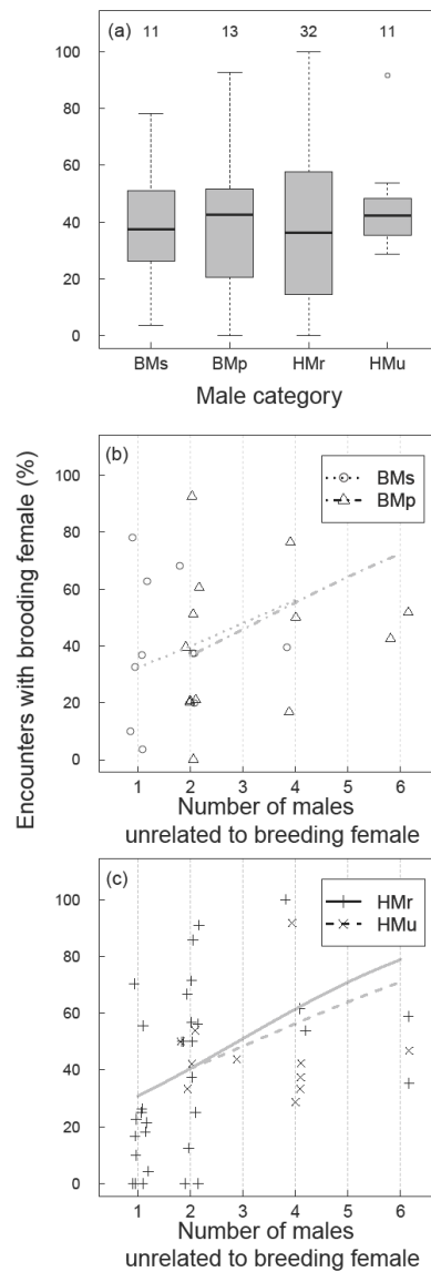
Figure 2.2. Probability of encounter with the breeding female on the nest. (a) Box plot shows median, interquartile range and approximate 2.5–97.5 percentiles of observed data. Circles represent outliers. The numbers at the top denote the sample size for each category. (b-c) Relationships between the encounter probability and the number of unrelated males within a breeding unit for either breeding (b) or helper males (c). Non-significant trend lines predicted by median estimates of the generalized linear mixed model cover ranges of the number of unrelated males observed for each category. Acronyms for male category are provided in Fig. 2.1 legend. Data points are jittered along x axis. Vertical grey dotted lines show the true positions of values on the x-axis.
