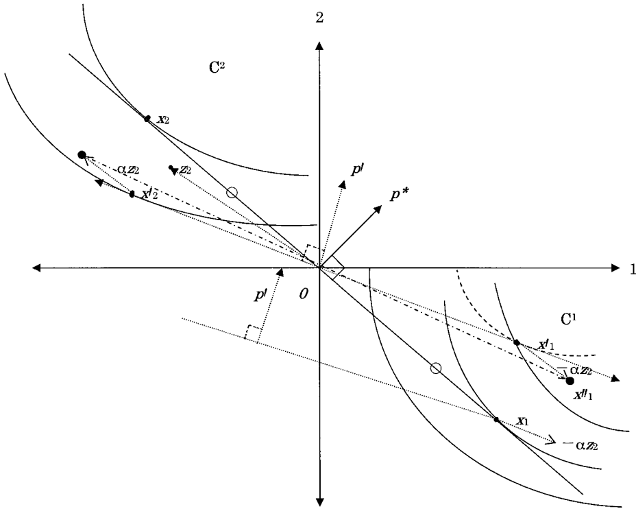
Figure 3 . An Illustration of Lemma 6
