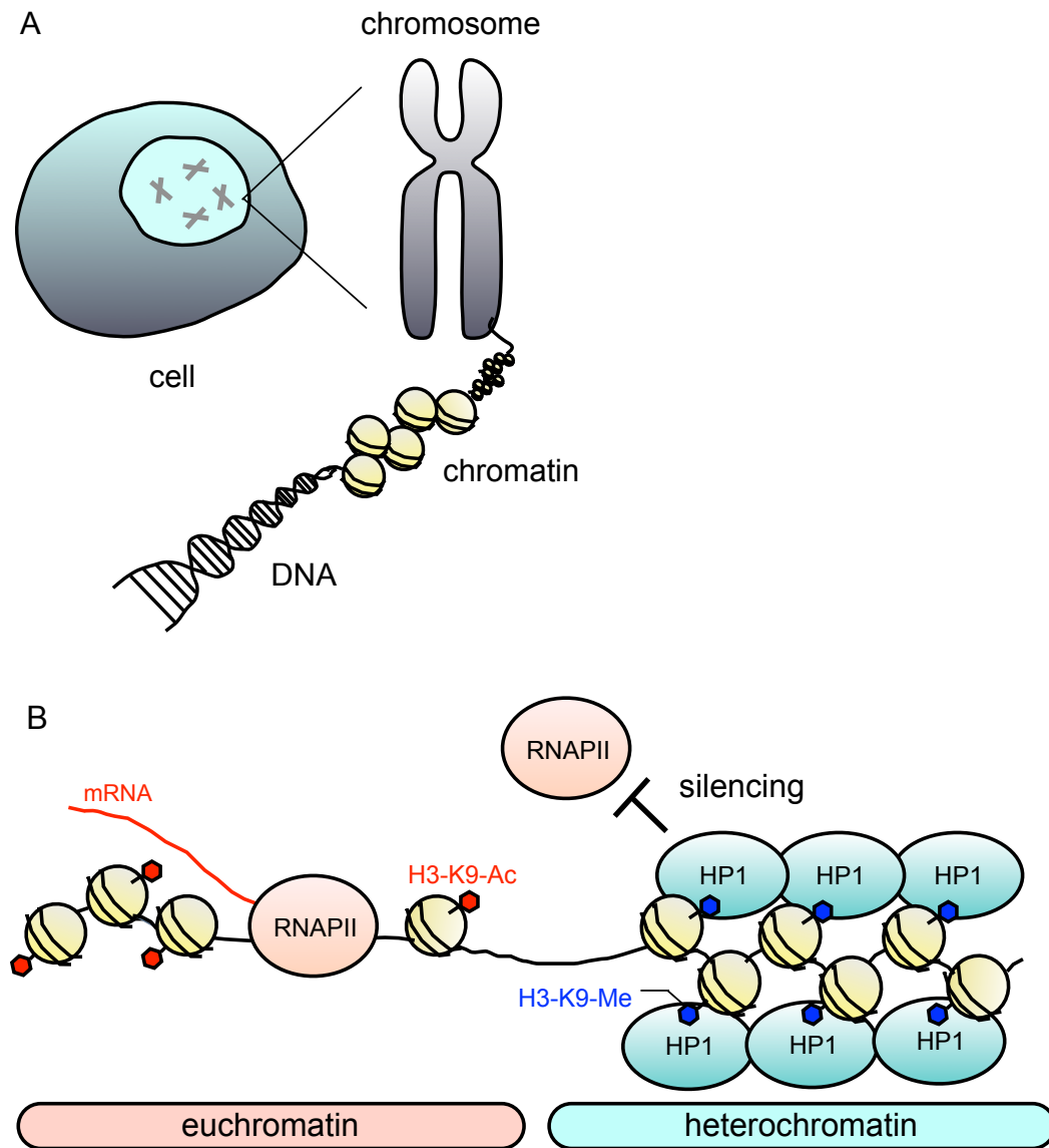
Figure 1. Chromatin Structure
