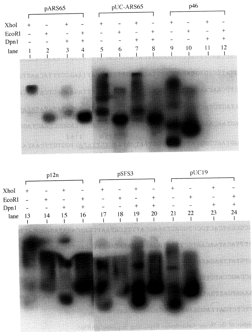
Fig. 3. Southern Blot Analysis of Plasmids Replicated in the Established Cell Lines Total DNAs were extracted from the established cell lines, digested with EcoRI or XhoI with or without DpnI, and subjected to Southern blot analysis. Hybridization was carried out with a 32 P-labeled pUC19 probe.
