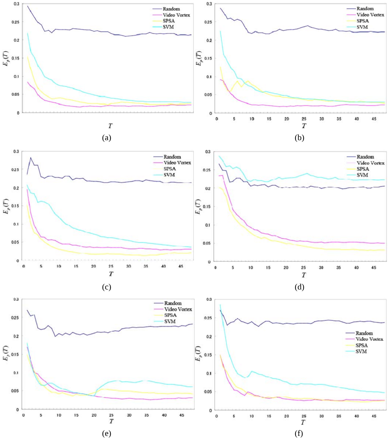
Fig. 3. Relationship between the criterion of “the law of proximity” and the retrieval iteration: (a) – (f) correspond to the results of tests 1-6. Note that Video Vortex, Random, SVM and SPSA respectively represent the proposed system, the random content views and the previously reported two methods (Bruno, Moenne-Loccoz, Marchand-Maillet, 2008), (Sudha, Shalabh, Basavaraja, Sridhar, 2008).
