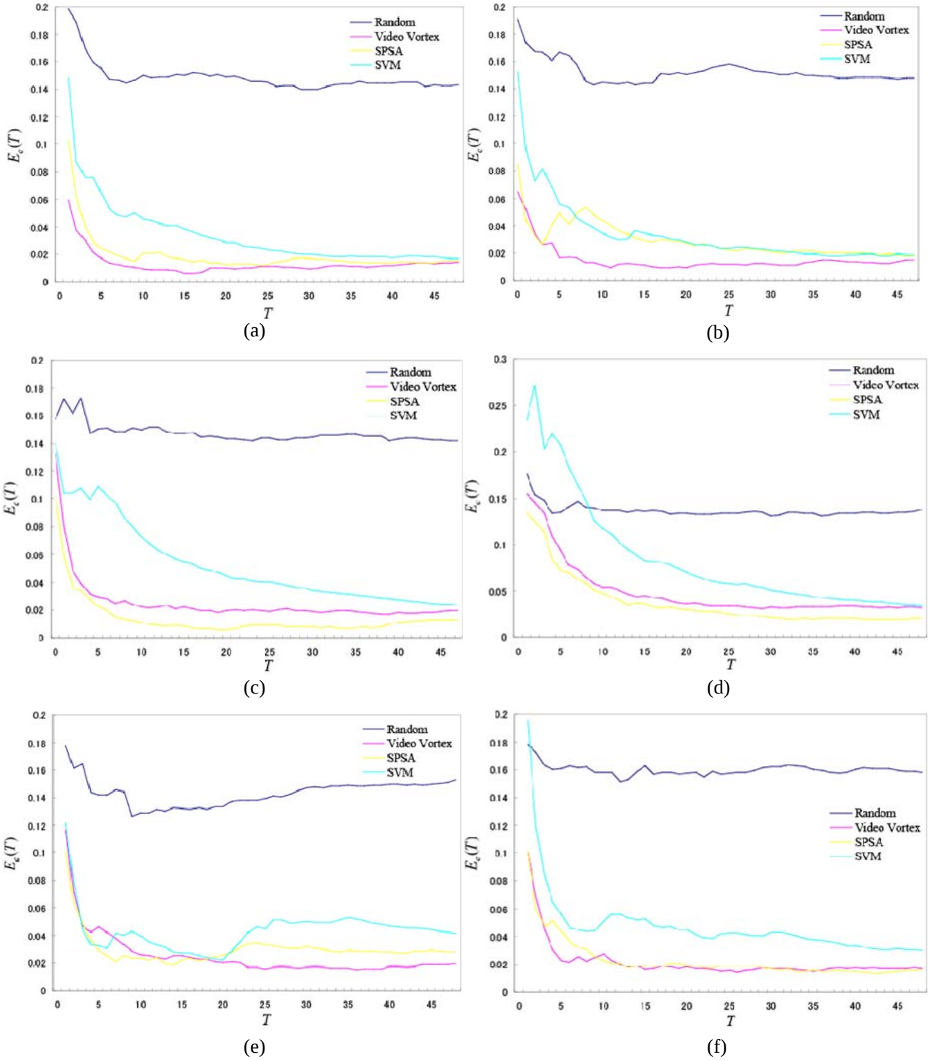
Fig. 4. Relationship between the criterion of “the law of good continuation” and the retrieval iteration: (a) – (f) correspond to the results of tests 1-6. Note that Video Vortex, Random, SVM and SPSA respectively represent the proposed system, the random content views and the previously reported two methods (Bruno, Moenne-Loccoz, Marchand-Maillet, 2008), (Sudha, Shalabh, Basavaraja, Sridhar, 2008).
