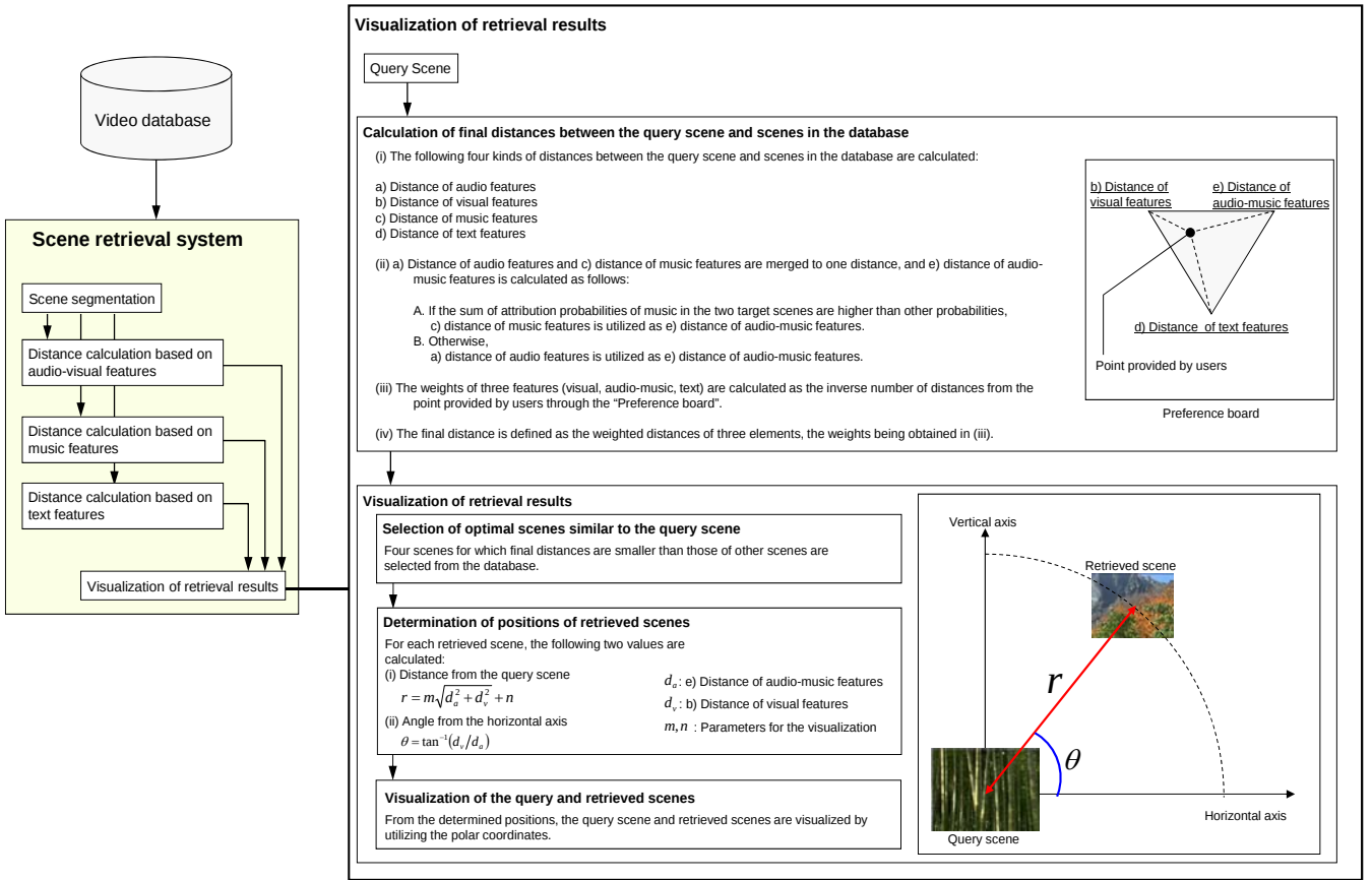
Fig. 2. Specific procedures for visualization of retrieval results. The visualization step is broadly composed of two schemes, "Calculation of final distances between the query scene and scenes in the database" and "Visualization of retrieval results". In the first scheme, the final distance is determined from the results obtained by the Preference board. In the second scheme, the scenes are shown on the basis of the final distance calculated in the first scheme and distances of audio-music and visual features.
