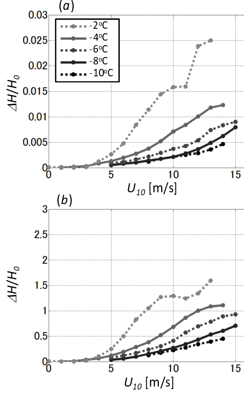
Figure 12: Relationship between fraction of heat flux difference and wind speed in (a) case 2 and (b) case 5. Each plot represents a different air-sea temperature difference ( T_a - T_s ).
