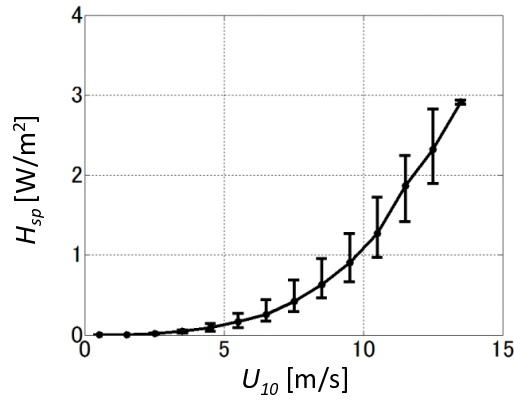
Figure 11: Latent heat flux of spray evaporation additionally given on the ocean surface as a boundary condition in case 2.
