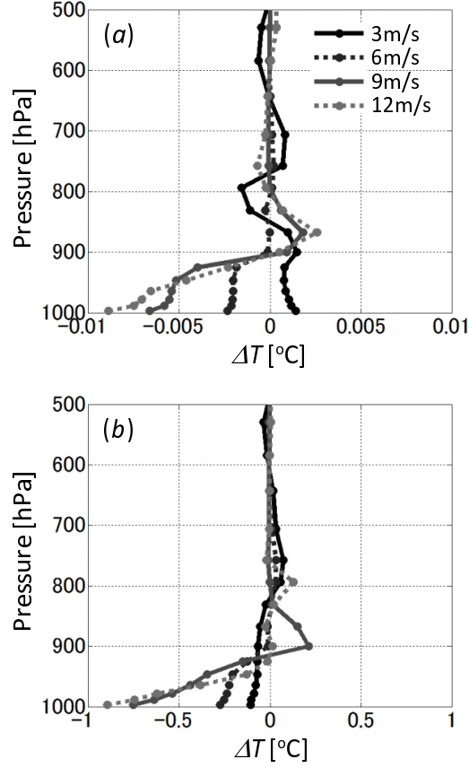
Figure 8: Vertical profiles of mean temperature difference over the target area in (a) case 2 and (b) case 5. Each plot represents a 10-m wind speed.
