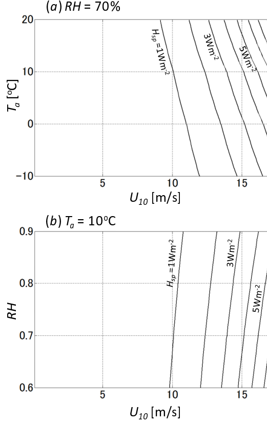
Figure 1: Contour of the spray latent heat calculated by the present method with various meteorological conditions with (a) constant humidity and (b) constant air temperature.
