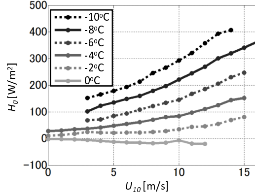
Figure 10: Total heat flux through the ocean surface in case 1. Each plot represents a different air-sea temperature difference ( T_a - T_s ).
