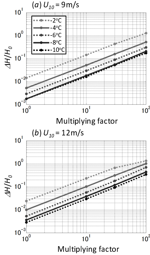
Figure 13: Relationship between the multiplying factor of SGF and fraction of heat flux difference with (a) U_{10} = 9 \text{ ms}^{-1} and (b) U_{10} = 12 \text{ ms}^{-1} . Each plot represents a different air-sea temperature difference ( T_a - T_s ).
