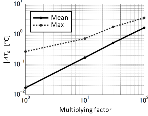
Figure 7: Relationship between the multiplying factor of SGF and mean/maximum temperature difference during 0 \leq t \leq 12 hr that appeared over the target area in cases 2–5.
