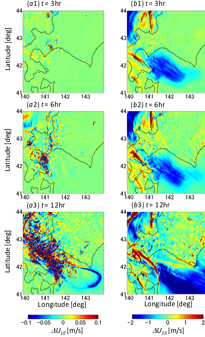
Figure 9: Distributions of difference in 10-m wind speed in (a) case 2 and (b) case 5 at t = 3, 6 , and 12 hr.
