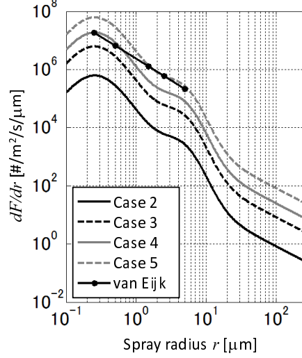
Figure 4: Spray source function given in case 2–5 when U_{10} = 8.4 \text{ ms}^{-1} (based on Gong, 2003) and a source function by van Eijk et al. (2011).
