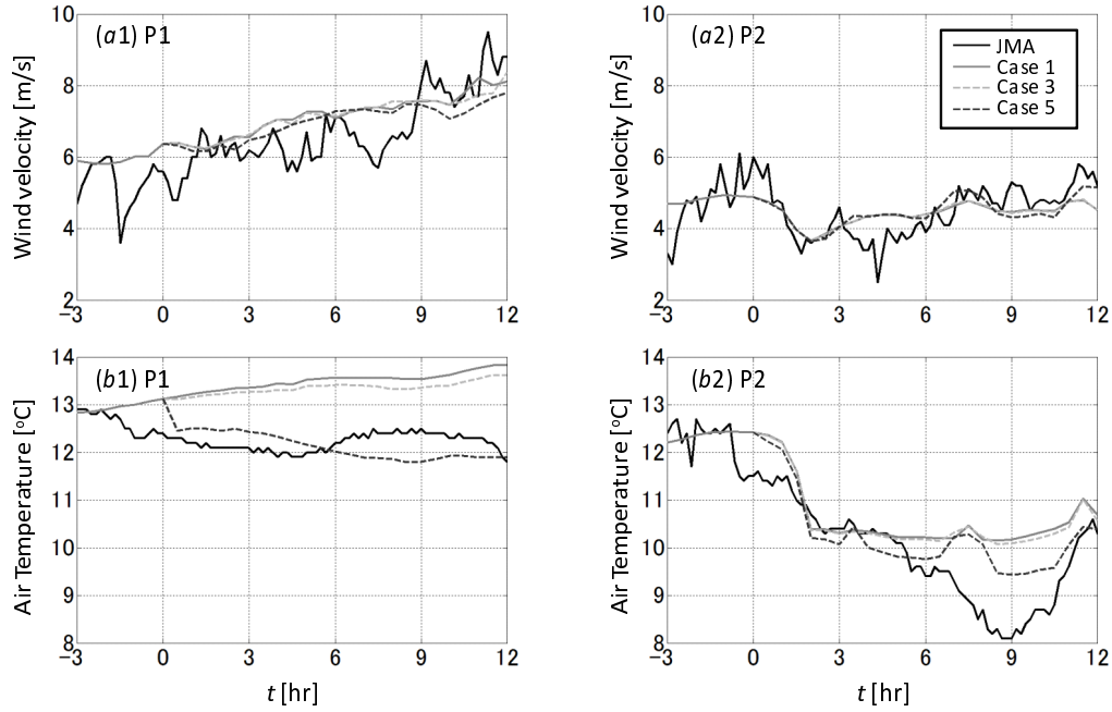
Figure 14: Comparison of the present results with observational data for (a) wind speed and (b) air temperature at the locations (1) P1, (2) P2 and (3) P3.
