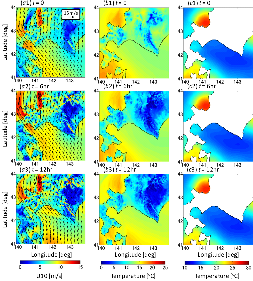
Figure 5: Distributions of (a) wind velocity U_{10} , (b) air temperature near the surface T_a and (c) sea surface temperature T_s at t = 0, 6 and 12 hr in case 1.
