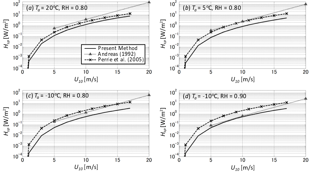
Figure 2: Comparison of the latent heat of sea spray estimated by the present method, the method of Andreas (1992) and the method of Perrie et al. (2005) under the conditions of the air pressure p = 1000 hPa and (a) T_a = 20^\circ\text{C} , RH = 80\% , (b) T_a = 5^\circ\text{C} , RH = 80\% , (c) T_a = -10^\circ\text{C} , RH = 80\% and (d) T_a = -10^\circ\text{C} , RH = 90\% .
