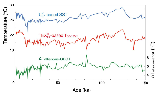
Fig. 5. \text{TEX}_{86}^{\text{H}} -derived temperatures at 30–125 m ( T_{30-125\text{m}} ), \text{U}_{37}^{\text{K'}} -derived SST (this study), and the difference between \text{U}_{37}^{\text{K'}} -derived SST and T at 30–125 m ( \Delta T_{\text{alkenone-GDGT}} ) in core MD97-2151.
