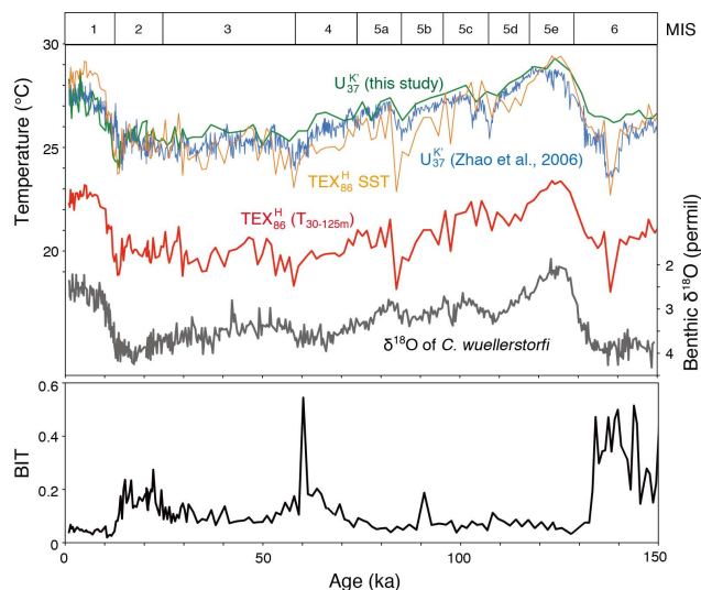
Fig. 4. \text{TEX}_{86}^{\text{H}} -derived SST (this study), \text{TEX}_{86}^{\text{H}} -derived temperature at 30\text{--}125\text{ m} ( T_{30-125\text{m}} ; this study), U_{37}^{K'} -derived SST (Zhao et al., 2006 and this study), \delta^{18}\text{O} of Cibicoides wuellerstorfi (Zhao et al., 2006), and the BIT index value (this study) in core MD97-2151. The analytical errors of \text{TEX}_{86}^{\text{H}} -derived SST, T_{30-125\text{m}} , U_{37}^{K'} -derived SST are 0.45\text{ }^\circ\text{C} , 0.36\text{ }^\circ\text{C} , and 0.24\text{ }^\circ\text{C} , respectively.
