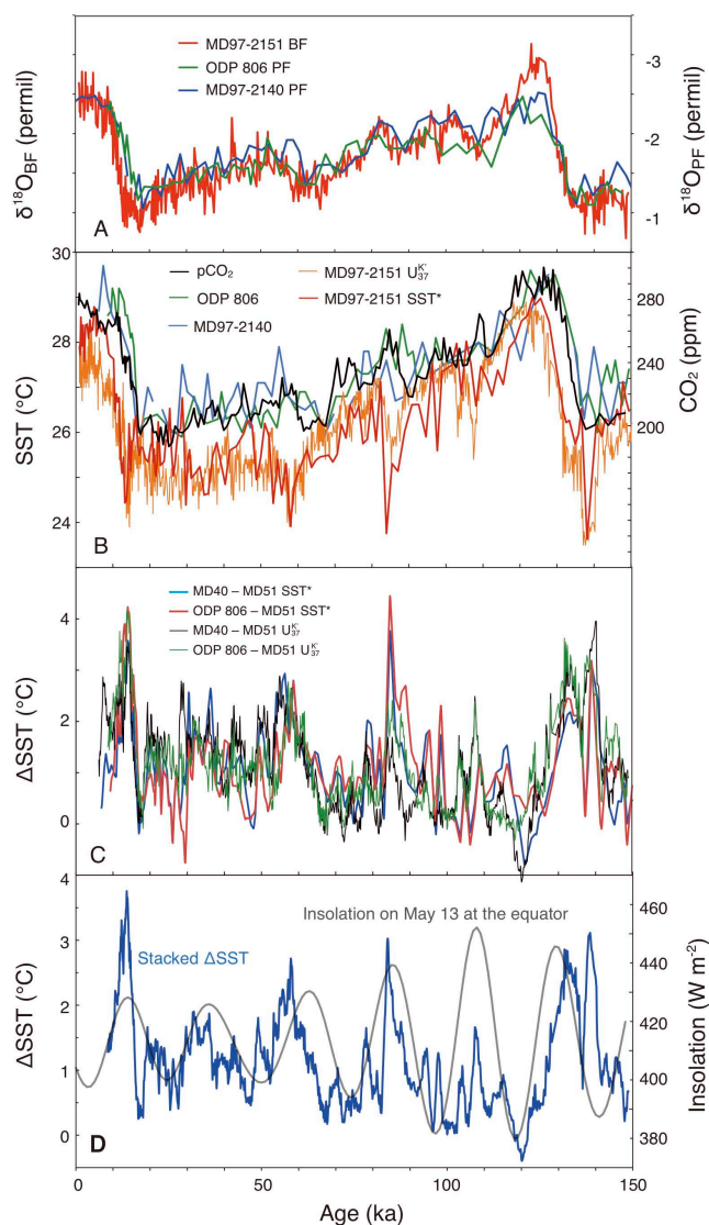
Fig. 6. (A) \delta^{18}\text{O} of benthic foraminifera (BF) in core MD97-2151 (Zhao et al., 2006) and of planktonic foraminifera (PF) in ODP 806 (Lea et al., 2000) and core MD97-2140 (de Garidel-Thoron et al., 2005). (B) \text{TEX}_{86}^{\text{H}} -derived SSTs* and \text{U}_{37}^{\text{K'}} -derived SSTs in core MD97-2151, Mg/Ca-derived SSTs in core MD97-2140 (de Garidel-Thoron et al., 2005), and ODP 806 (Lea et al., 2000), and \text{CO}_2 concentrations from Dome Fuji (Kawamura et al., 2007). (C) Temperature differences ( \Delta\text{SSTs} ) between the central Western Pacific Warm Pool region (MD97-2140 and ODP 806) and Site MD97-2151 in the southern South China Sea. (D) The stacked \Delta\text{SST} . The insolation on May 13 at the equator is shown for comparison. Temperatures were calculated from \text{U}_{37}^{\text{K'}} using an equation based on the core-top calibration (Pelejero and Grimalt, 1997). \text{SST}^* [^{\circ}\text{C}] = T_{30-125\text{m}} [^{\circ}\text{C}] + 5.6 . The analytical error of Mg/Ca-derived SST is 0.5 °C (de Garidel-Thoron et al., 2005).
