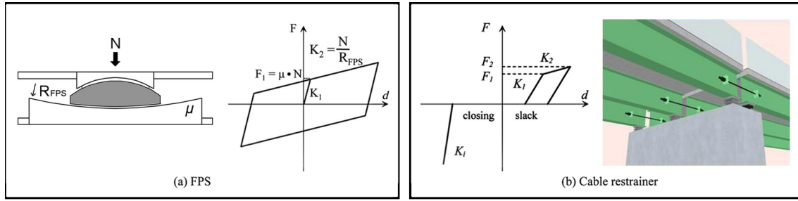
Figure 2: Analytical model of FPS and cable restrainers.
