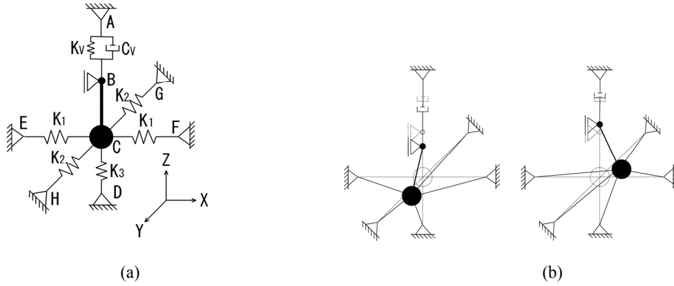
Figure 1: MD-TMD model; (a) components of MD-TMD, (b) deformation of damper due to horizontal displacements of mass
