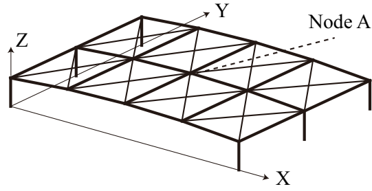
Figure 2: Latticed shell model
