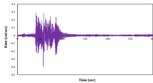
Figure 10 The vertical velocity response of point 2
