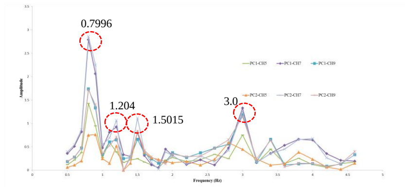
Figure 5 Spectra measured from different velocity meters
