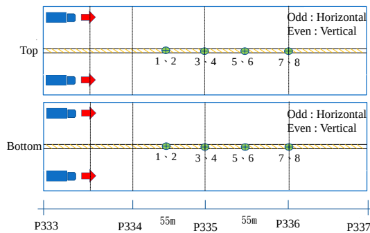
Figure 9 The instrumentation layout on both decks
