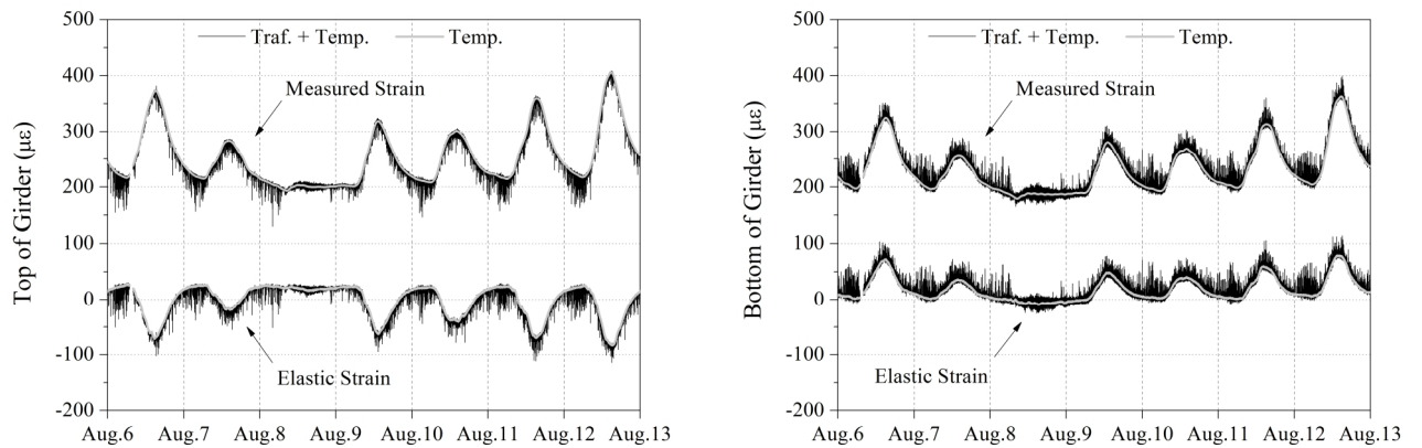
Figure 8: Strain at mid-span of girder
