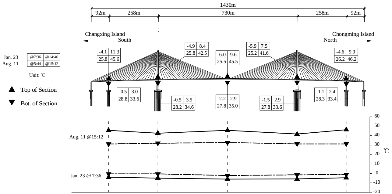
Figure 2: Longitudinal temperature distribution
