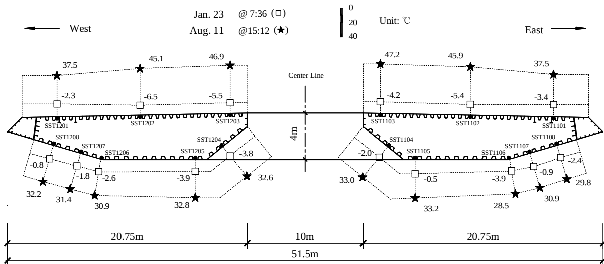
Figure 3: Temperature field at mid-span
