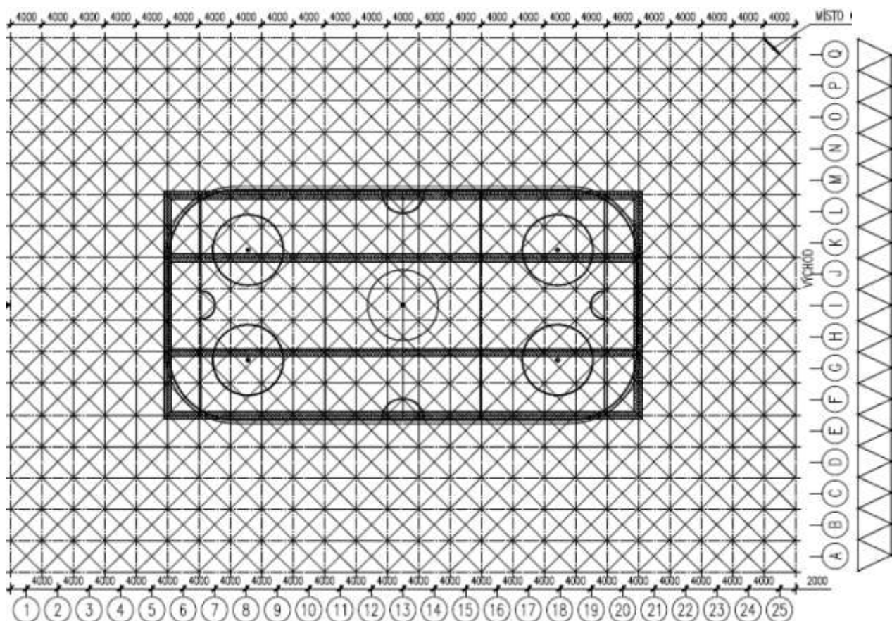
Figure 1: Winter sport stadium in Olomouc city – scheme of spatial truss grid of steel roof structure (plan and transverse section).
