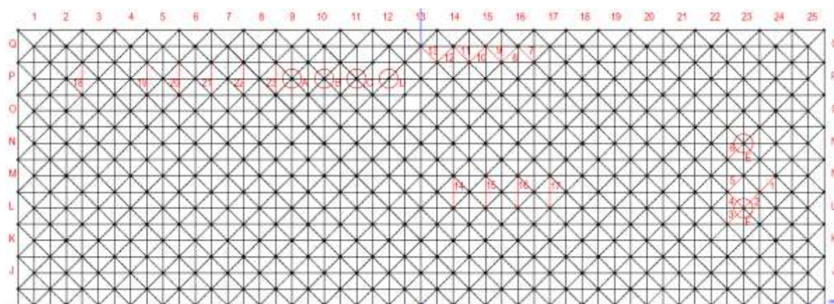
Figure 3: Localization of positions of verified tube members and spherical joints.
