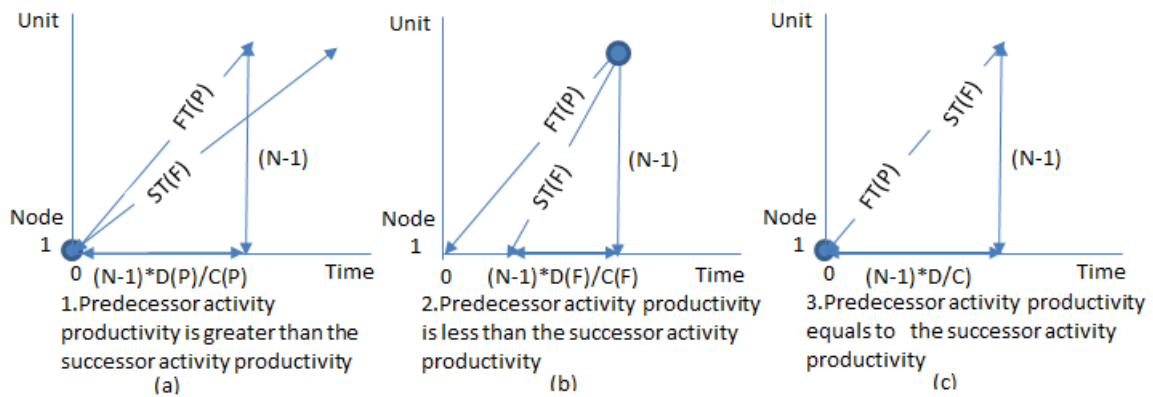
Figure 2: CPM/LOB scheduling sequence formula (FS).
