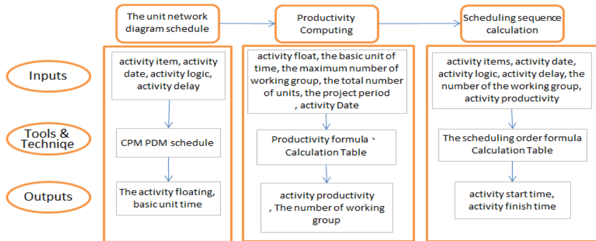
Figure 3: CPM/LOB scheduling calculation flowchart.
