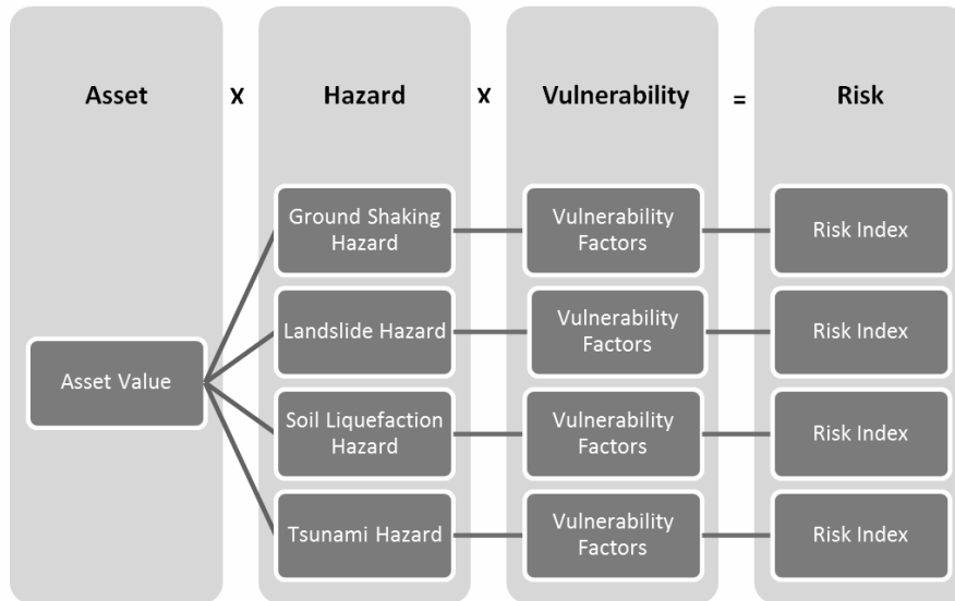
Figure 1: Seismic Risk Assessment Framework
