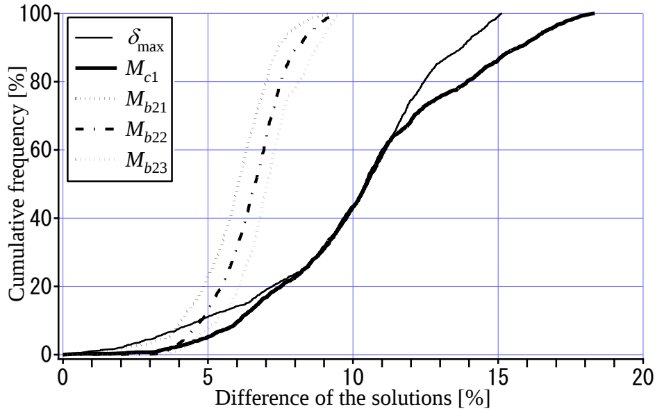
Figure 9: Cumulative frequency distribution of the differences of the FEM solutions and solutions of this calculation formula
