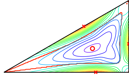
Figure 2: Contour of distribution of the principal bending moment
