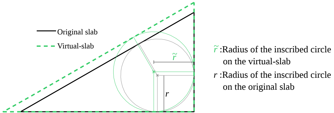
Figure 6: virtual-slab and its radius of the inscribed circle \tilde{r}
