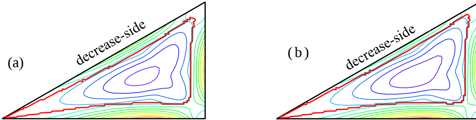
Figure 4: Contour of distribution of the M_A (a) decrease-ratio is 40 %; (b) decrease-ratio is 60 %
