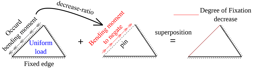
Figure 3: Process of calculate the solution when the degree of fixation decreases
