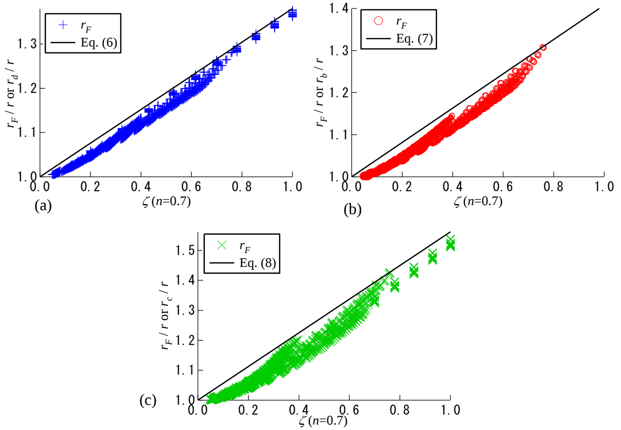
Figure 8: r_F and \tilde{r}_k (a): Case of \delta_{\max} (b): Case of M_{b2i} (c): Case of M_{c1}
