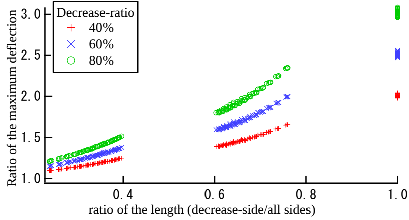
Figure 5: Ratios of the maximum deflections (case of the degree of fixation decrease to case of the fixed supported all edges)
