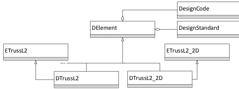
Figure 5: Class diagram of design elements.
