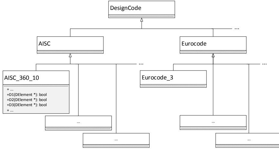
Figure 2: A class diagram for design codes.
