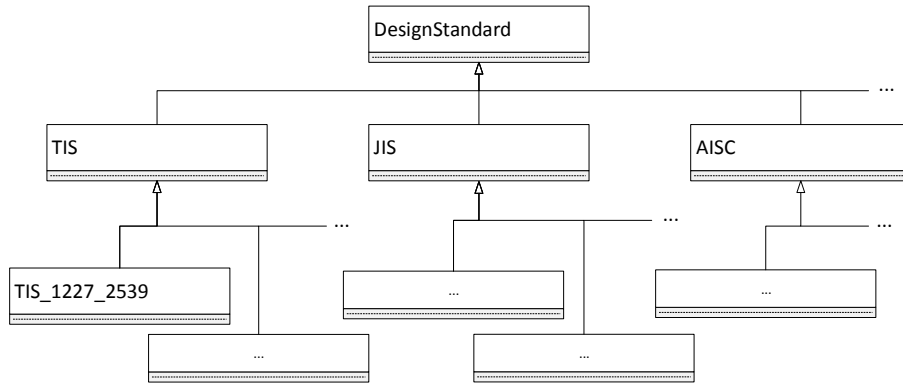
Figure 3: Class diagram for design standards.
