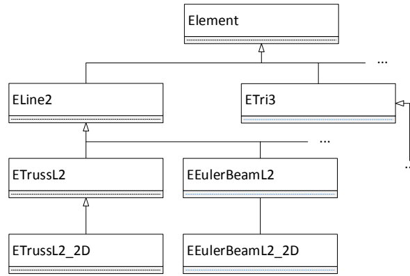
Figure 1: A class diagram for finite elements.
