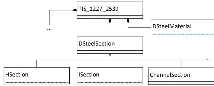
Figure 4: Class diagram of a Thai Industrial Standard.
