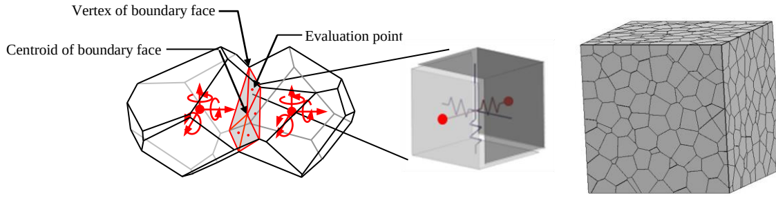
Figure 2: (a) Rigid-body-spring model and (b) Voronoi diagram
