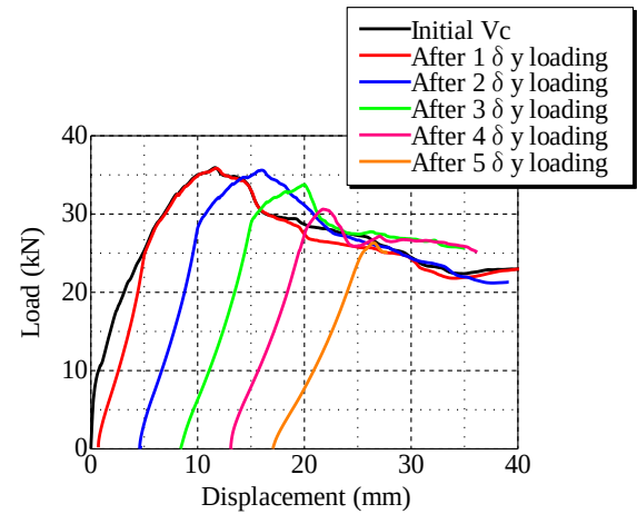
Figure 14: Load-displacement relationship
