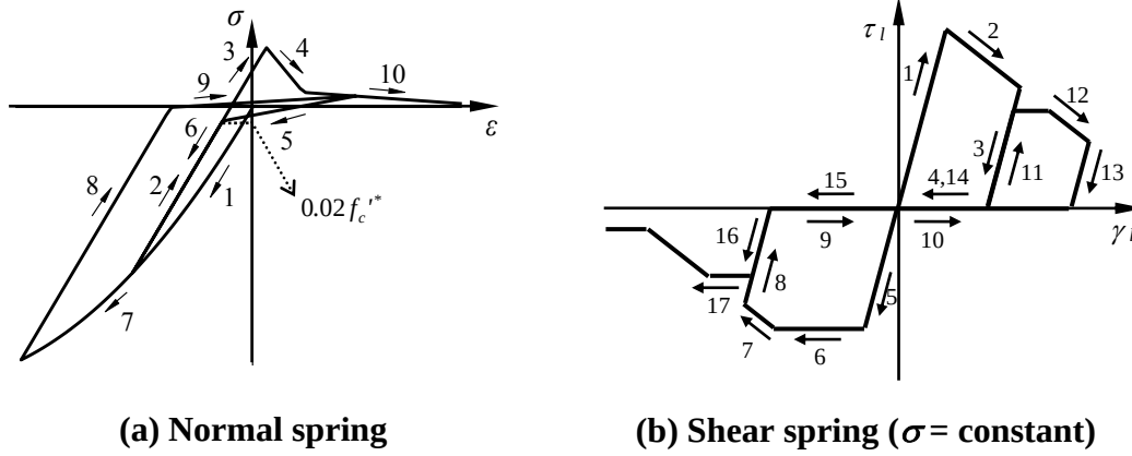
Figure 4: Hysteresis of stress – strain relation
