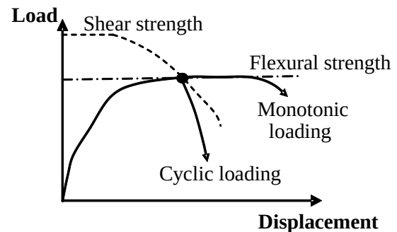
Figure 1: shear failure after flexural yielding
