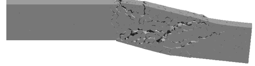
Figure 11: Deformation under cyclic loading at 20mm ( 4\delta_y )
