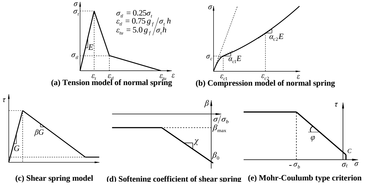
Figure 3: Constitutive model for concrete
