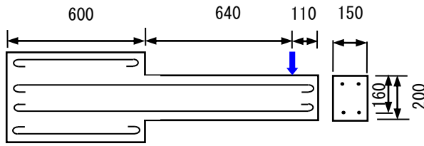
Figure 7: Dimension of specimen
