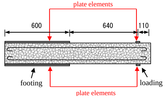
Figure 8: Analytical model
