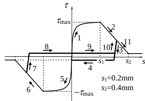
Figure 6: Bond - slip relationship
