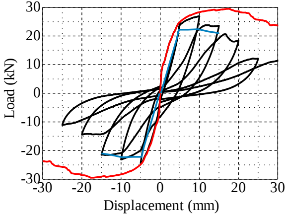
Figure 9: Load-displacement relationship
