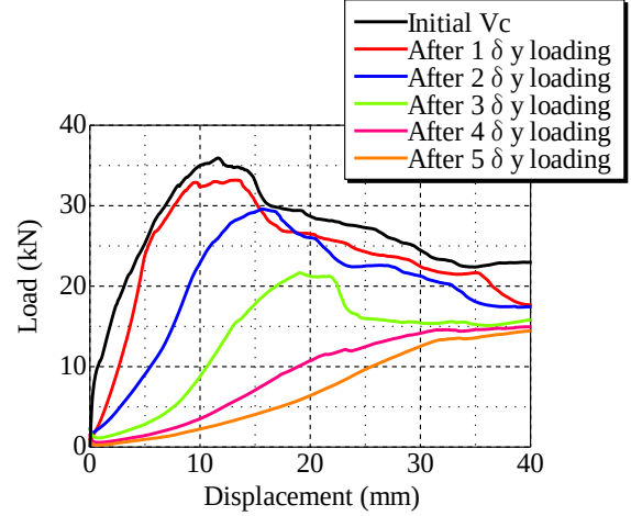
Figure 13: Load-displacement relationship
