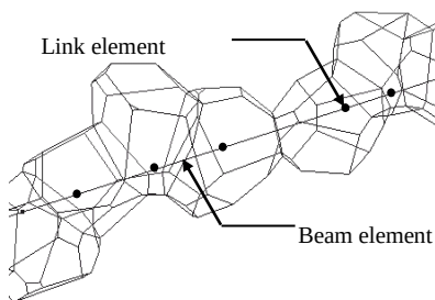
Figure 5: Reinforcement models
