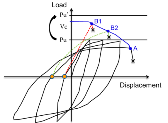
Figure 12: Concept of method
