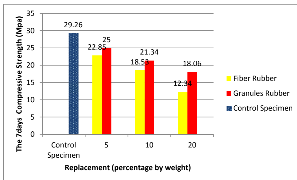
Figure 2: Results of 7-day compressive strength test.
