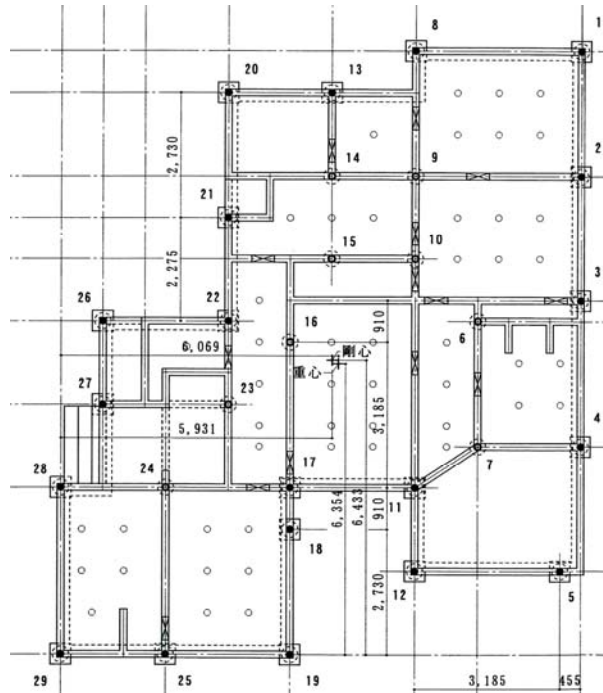
Figure 3: Real drawing plan of a pile foundation layout example.
