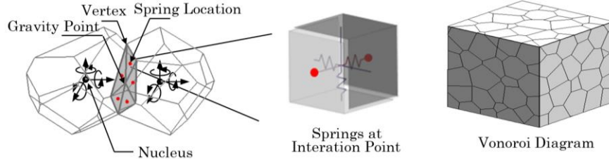
Figure 1: Concept of Rigid-Body Springs Model & Beam Model
