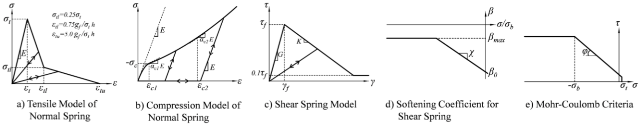
Figure 2: Constitutive Law of Each Spring's in 3D-RBSM
