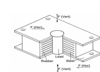
Fig.3: LRB device
