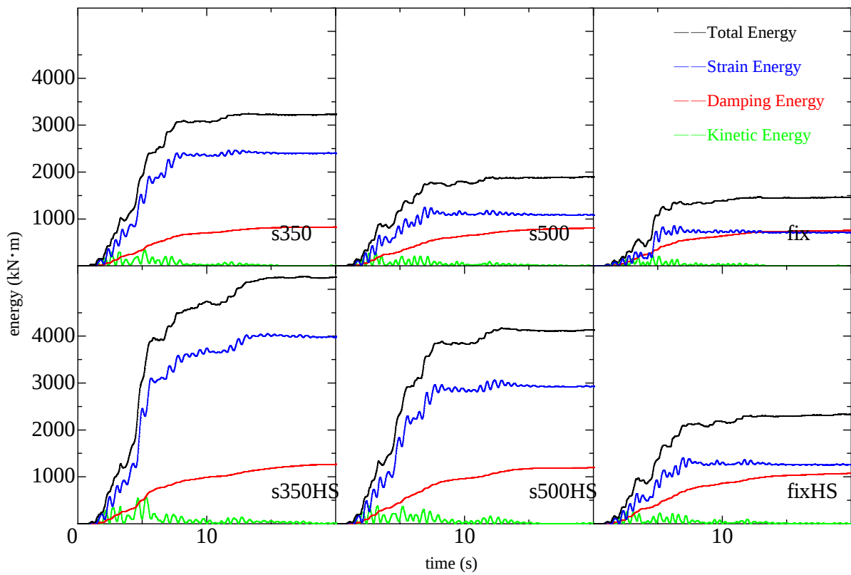
Fig.7: Energy-Time History
