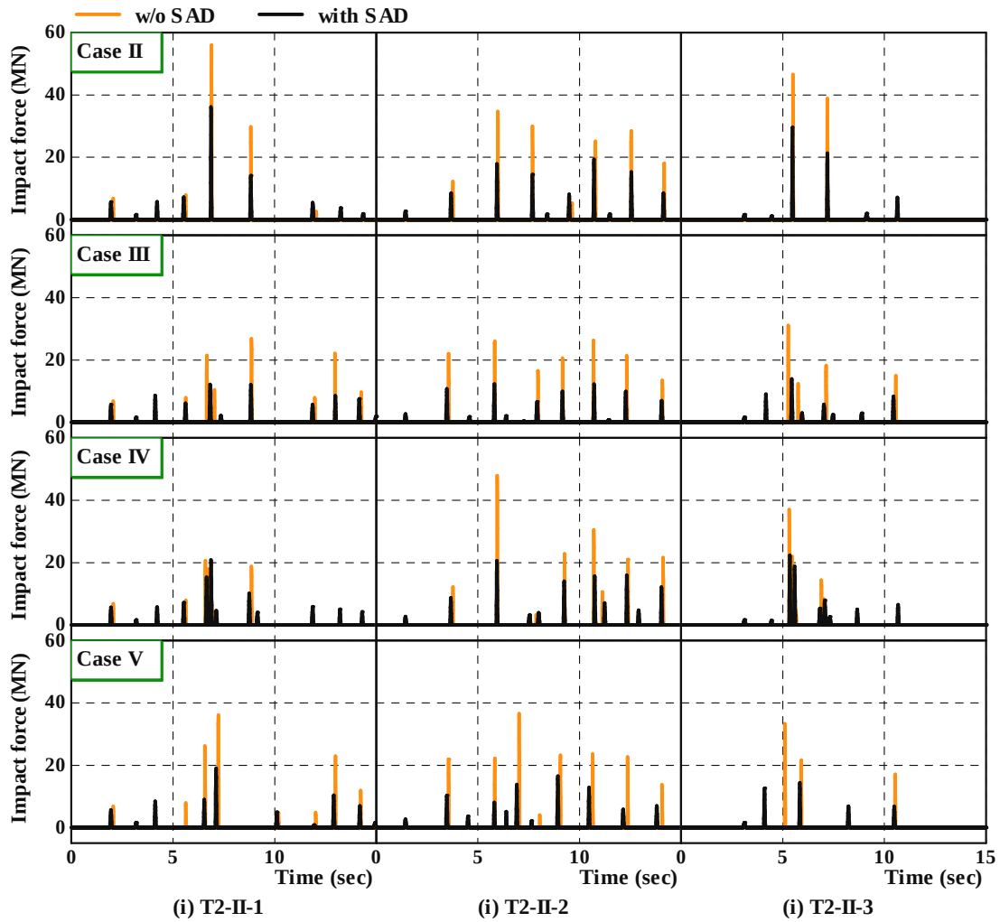
Figure 7 Impact force time history response with/without SAD
