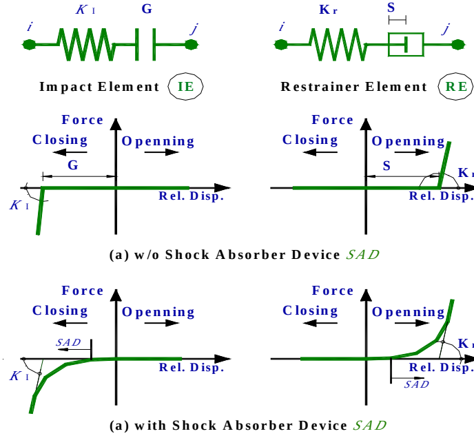
Figure 4 Pounding, restrainers and shock absorber device (SAD) analysis models
