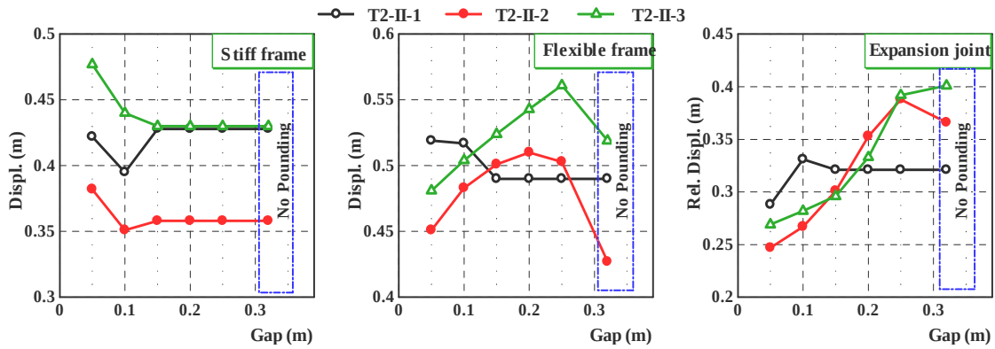
Figure 5 Variation of displacement peak response at expansion joint with gap size
