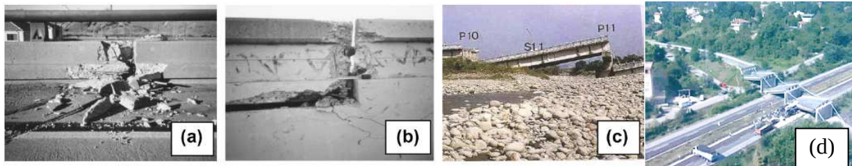
Figure 1 Typical seismic induced earthquake damages (a and b) pounding damage, (c and d) unseating damage
