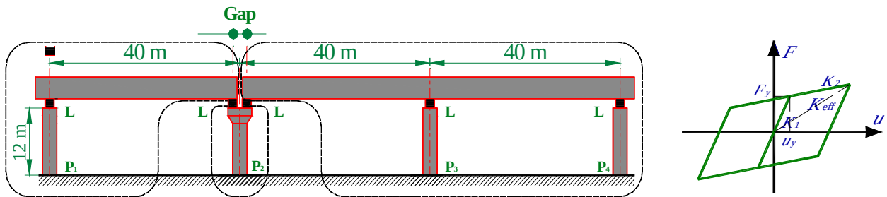
Figure 2 Base isolated bridge model with LRB bearings (L)
