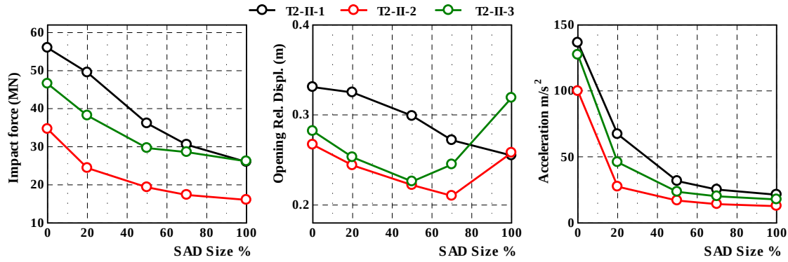
Figure 8 Peak responses variation with SAD size
