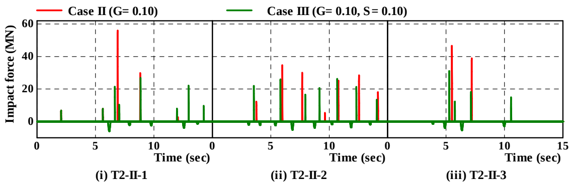
Figure 6 Impact force time history at expansion joint
