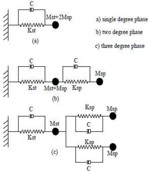
Figure 2: Analytical models.
