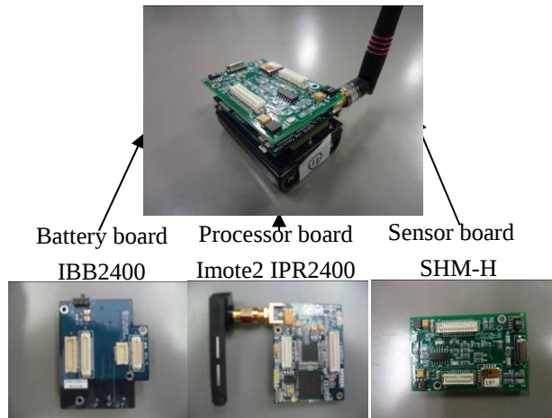
Figure 1: Imote2 smart sensor
