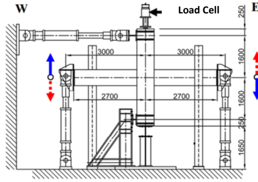
Figure 1: Testing system for beam-column joints of internal column
