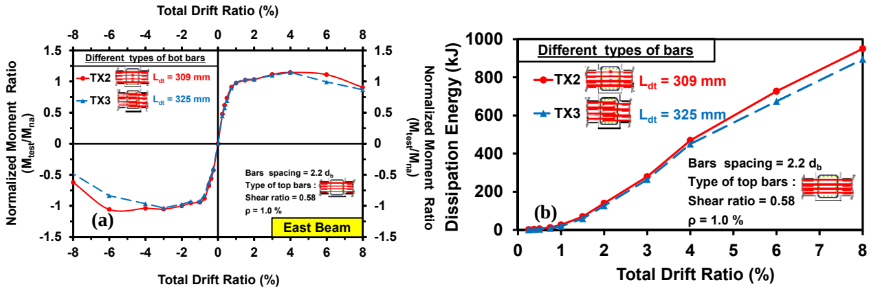
Figure 5: Comparison of envelope line and energy dissipation of specimen TX2 and TX3 by different connection types in joints
