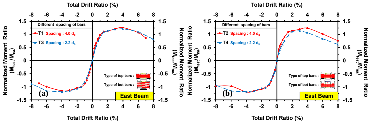
Figure 8: Comparison of envelope line of specimen T1 & T3 and T2 & T4 at different clear spacing of T-headed bars
