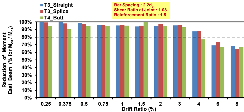
Figure 6: Comparison of reduction of moment in joints by different connection types in joints
