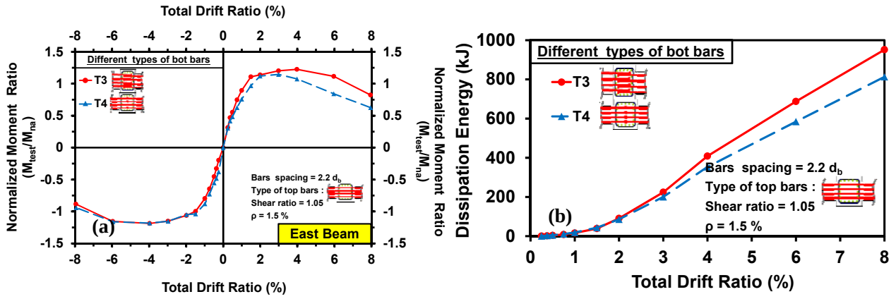
Figure 3: Comparison of envelope line and energy dissipation of specimen T3 and T4 by different connection types in joints
