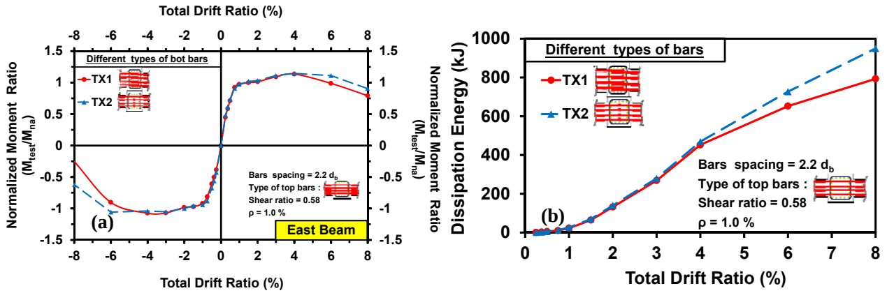
Figure 4: Comparison of envelope line and energy dissipation of specimen TX1 and TX2 by different connection types in joints
