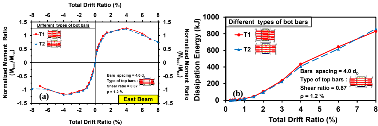
Figure 2: Comparison of envelope line and energy dissipation of specimen T1 and T2 by different connection types in joints
