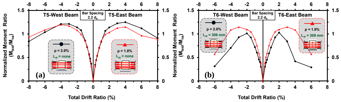
Figure 7: Comparison of reinforcement connection types of specimen T5 and T6 under different designs of reinforcement ratio
