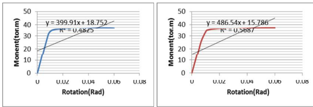
(a) WFP2-T specimen
