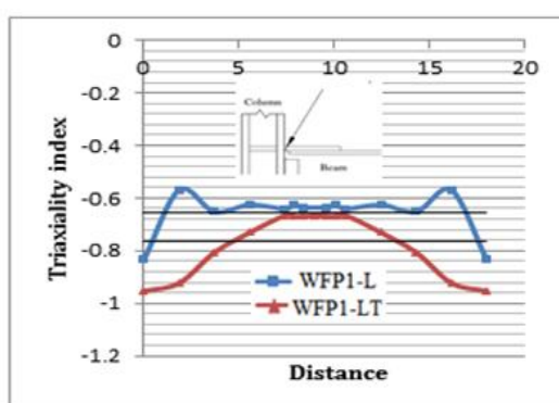
Fig6. Distribution of the Triaxiality index at the junction of beam to column at 2.0% rad story drift
