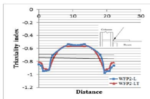
Fig 8 .Distribution of the Triaxiality index at the junction of beam to column at 2.0% rad story drift
