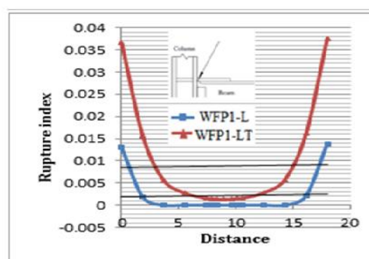
Fig7. Distribution of the Rupture index at the junction of beam to column at 2.0% rad story drift
