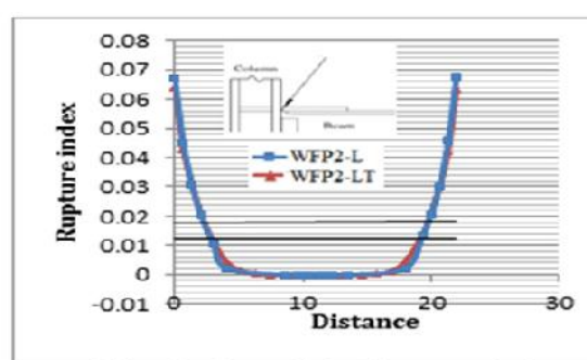
Fig 9 .Distribution of the Rupture index at the junction of beam to column at 2.0% rad story drift
