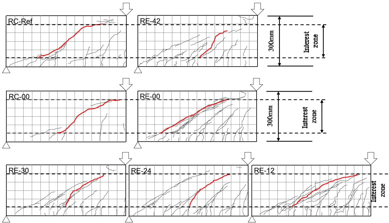
Figure 6: Cracking behavior at the peak load
