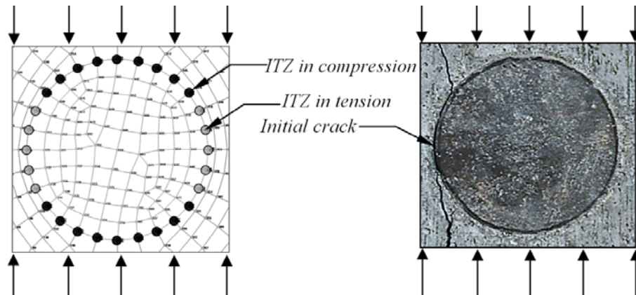
Figure 5: Initial Failure of Specimens.
