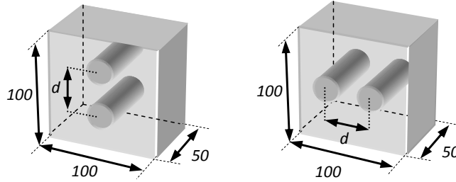
Figure 2: Test Specimen and Aggregate Configuration.
