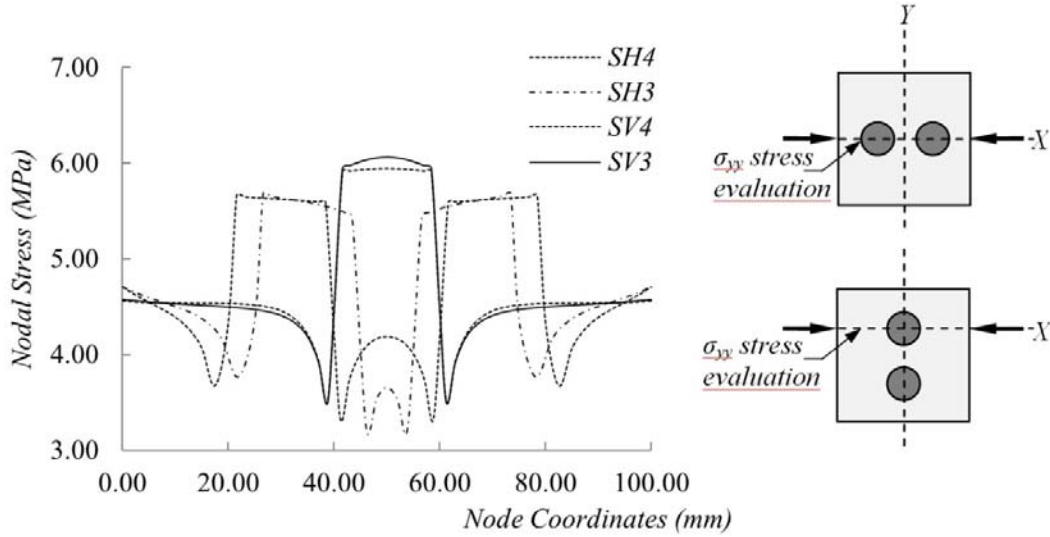
Figure 7: Stress Distribution at Mid-height.
