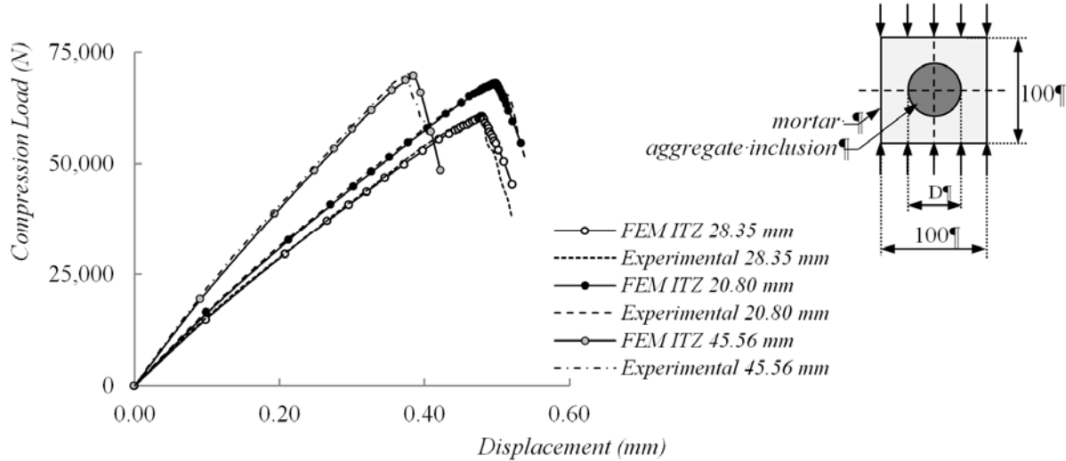
Figure 1: Validation of the FEM Program.
