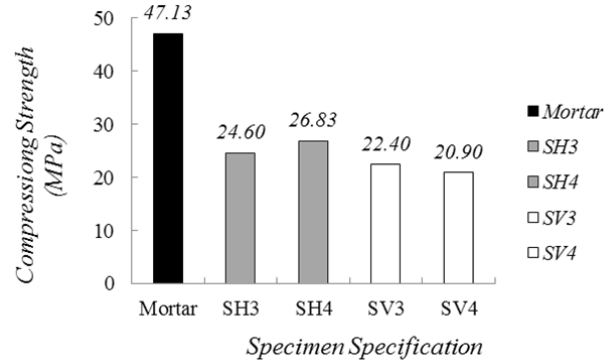
Figure 4: Ultimate Stress Comparison.
