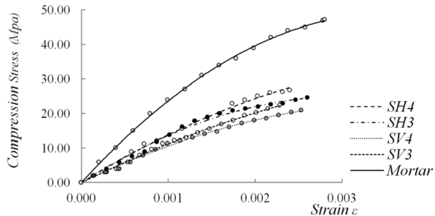
Figure 3: Stress-strain Response of Specimens.
