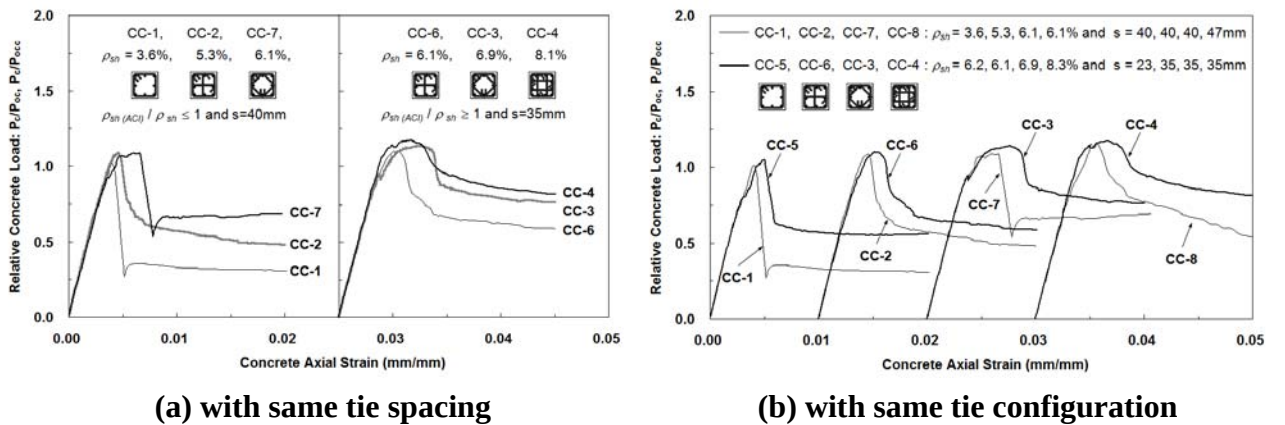
Figure 3: Effect of transverse reinforcement ratio.
