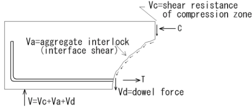
Figure 1: Shear transfer mechanism of slender beams
