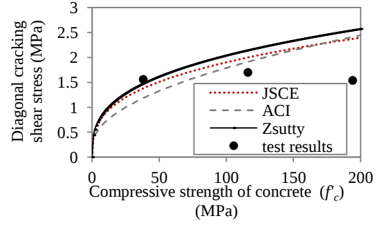
(b) Diagonal cracking shear stress of RC beams ( a/d=3.5 series)
