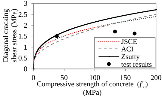
(a) Diagonal cracking shear stress of RC beams ( a/d=3.0 series)
