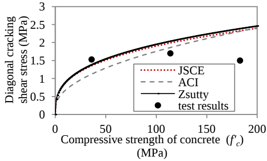
(c) Diagonal cracking shear stress of RC beams ( a/d=4.0 series)
