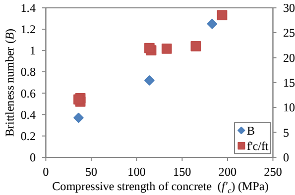
Figure 3: Brittleness of concrete
