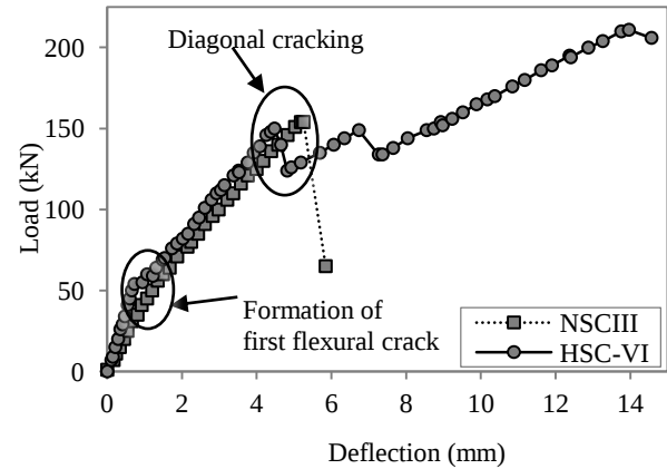
Figure 4: Comparison of load –deflection relationship of RC beams
