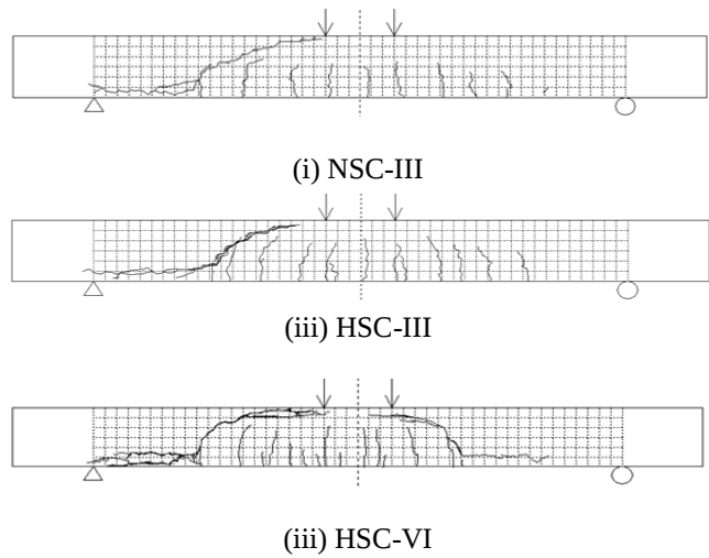
Figure 5: Beam crack pattern (just after failure, a/d=4.0 )
