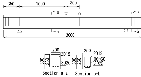
Figure 2: Details of RC beam (unit: mm)
