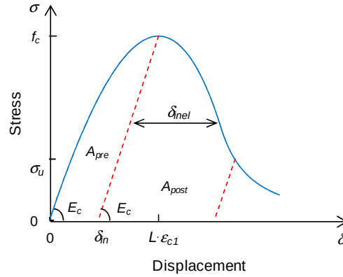
Figure 3: Fracture energy of concrete in compression (Jansen & Shah 1997)
