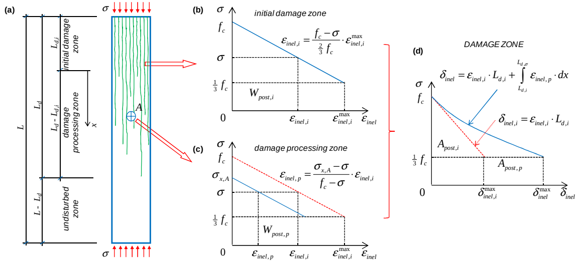
Figure 5: Postpeak inelastic strains of different zones in a specimen
