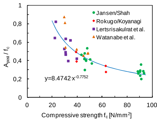
Figure 4: Compressive fracture energy versus compressive strength
