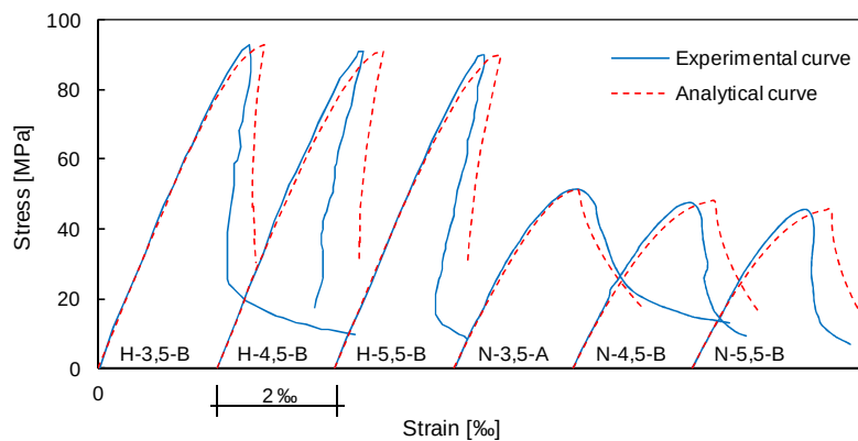
Figure 6: Total stress versus strain curves for some specimens of Jansen and Shah (1997)
