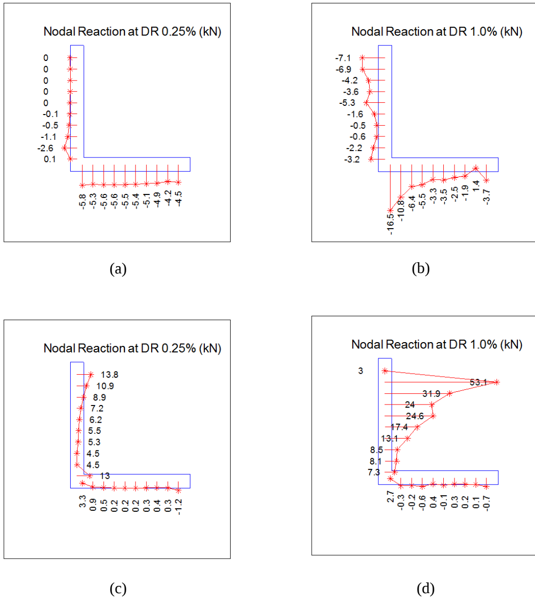
Figure 6: Numerically determined distribution of reaction forces at the base of the wall (a) out-of-plane force (b) out-of-plane force (c) in-plane force (d) in-plane force.
