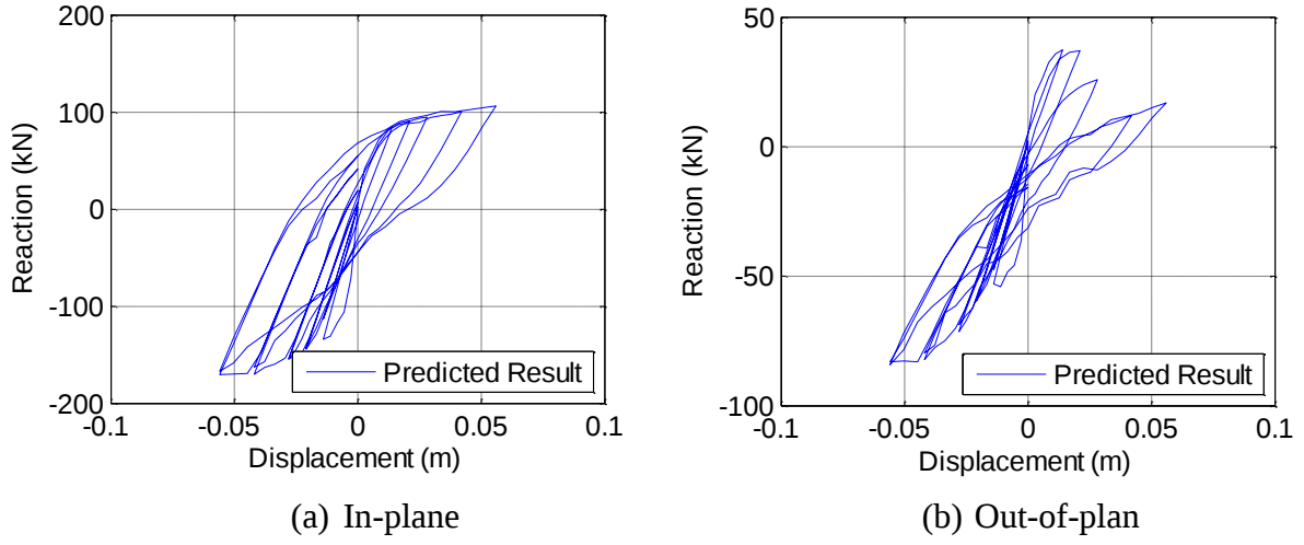
Figure 3: Deformation-reaction hysteresis loops for in-plane and out-of-plane.
