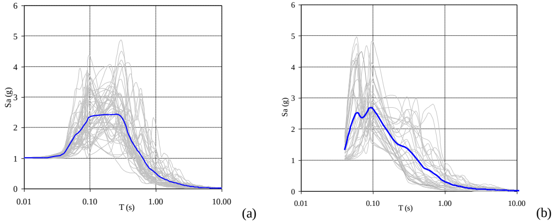
Figure 3: Acceleration response spectra (normalized to have PGA of 1g) with the damping ratio of 5% for a) Tohoku earthquake and b) Peruvian records
