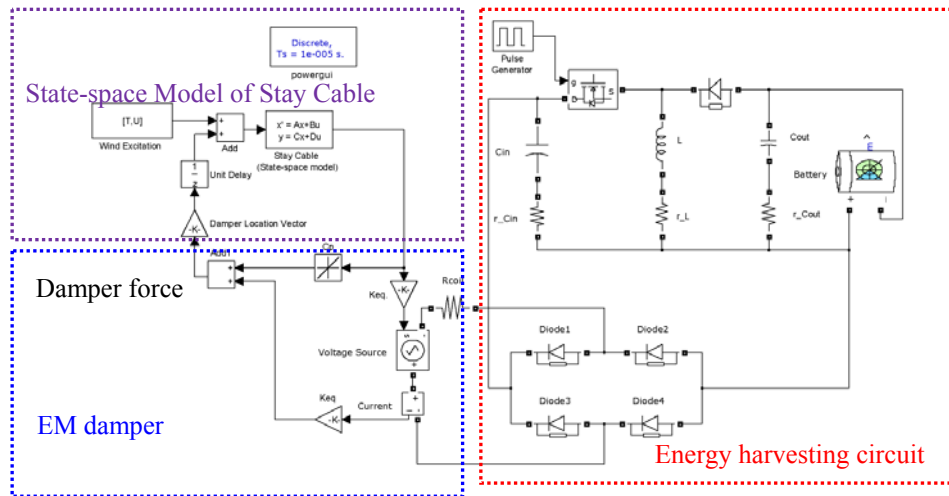
Figure 4: Simulink model of stay cable with EMDEH system.
