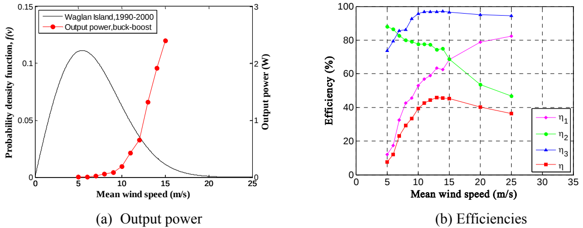
Figure 6: Energy harvesting performance of EMDEH system under different wind speed.
