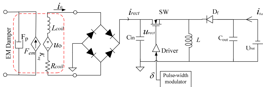
Figure 3: Schematic of energy harvesting circuit.
