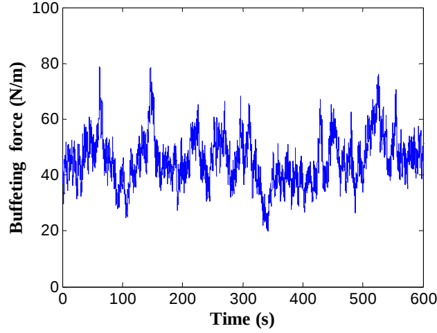
Figure 2: Wind force time histories on element 50 (mean wind speed: 9m/s).
