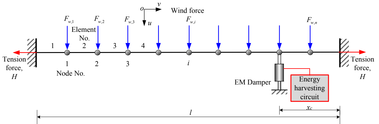
Figure 1: Discretized Model of a stay cable equipped with an EMDEH system.
