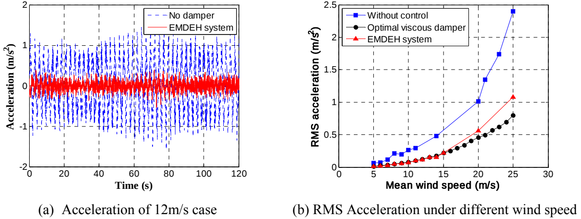
Figure 5: Vibration control performance of EMDEH system.
