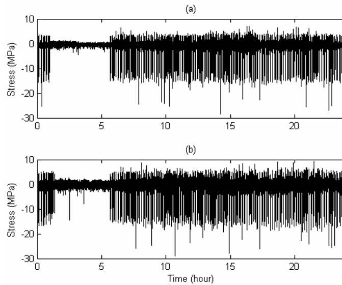
Figure 3: Daily stress time histories under multiple types of dynamic loads at the location of strain gauge SS-TLS-12: (a) computed; (b) measured
