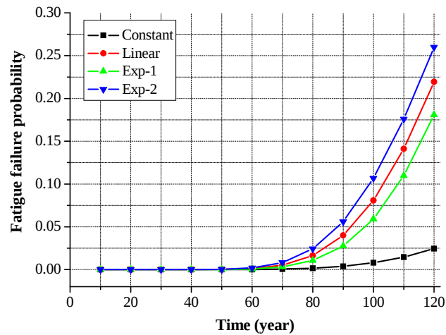
Figure 5 Evolution of fatigue failure probability over time
