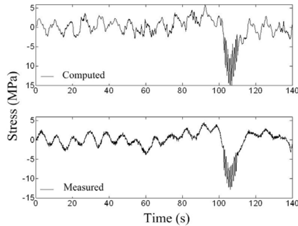
Figure 2: Comparison of stress responses under combined railway, highway and wind loading
