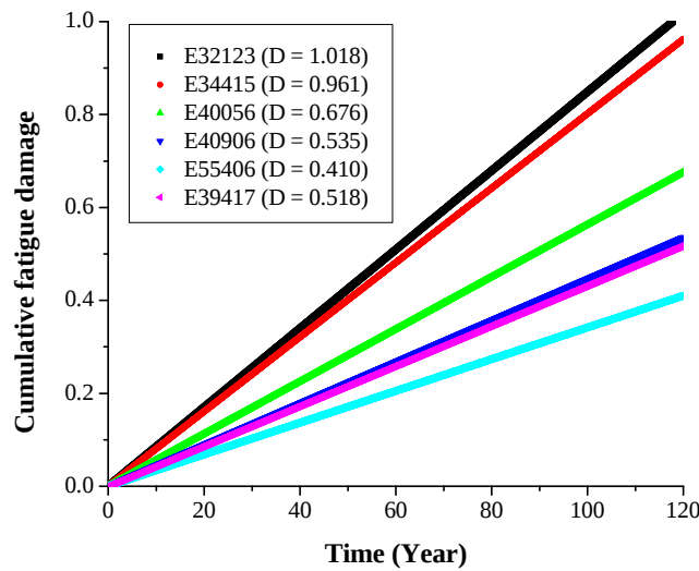
Figure 4: Cumulative fatigue damage curves at the fatigue-critical locations
