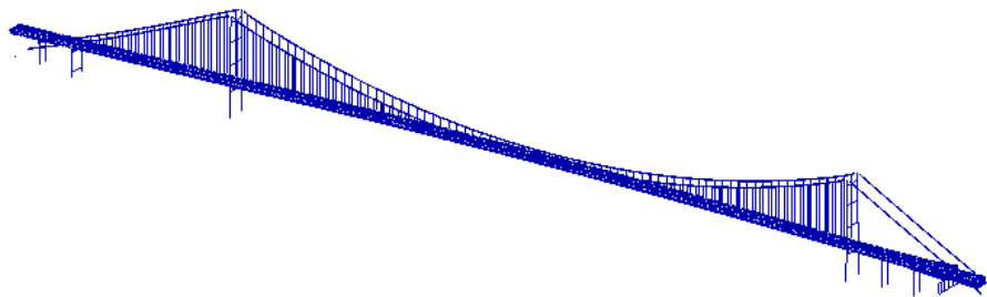
Figure 1: 3-D Finite element model of the Tsing Ma Bridge [3]
