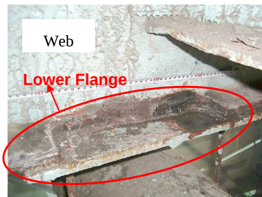
Figure 2: Existing reinforcement plate of transverse beam
