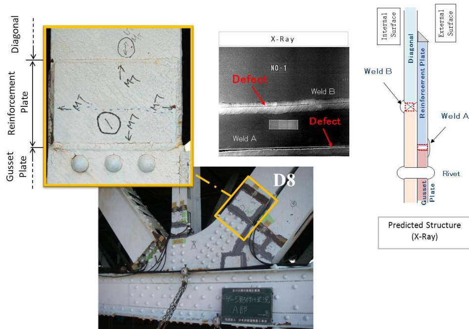
Figure 3: Example of existing reinforcement details in truss members
