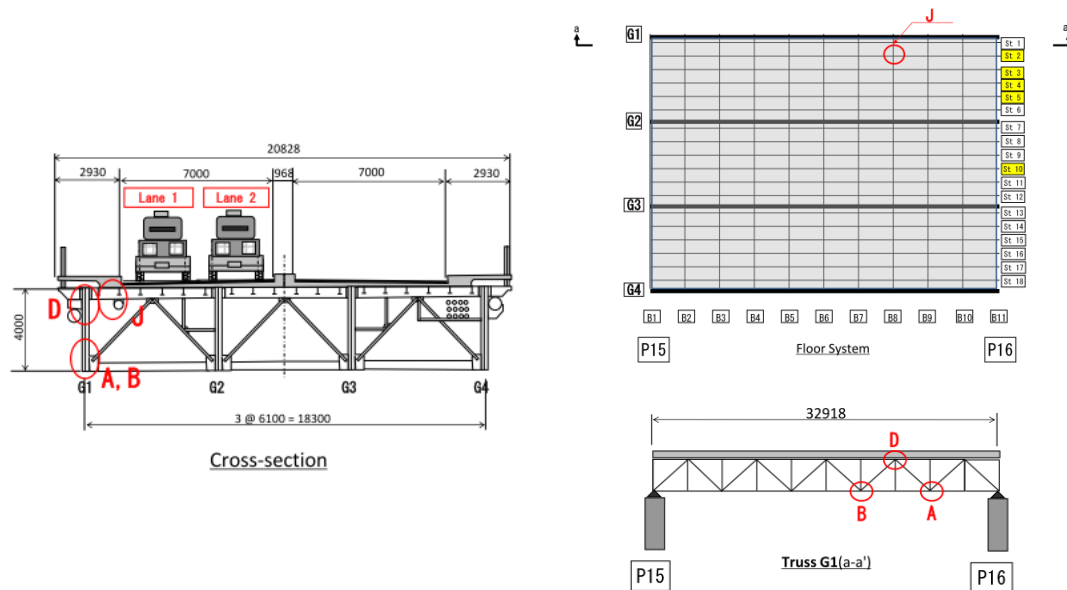
Figure 2: Measurement points
