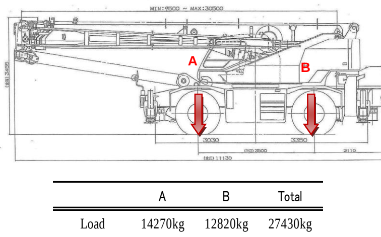
Figure 4: Test vehicle
